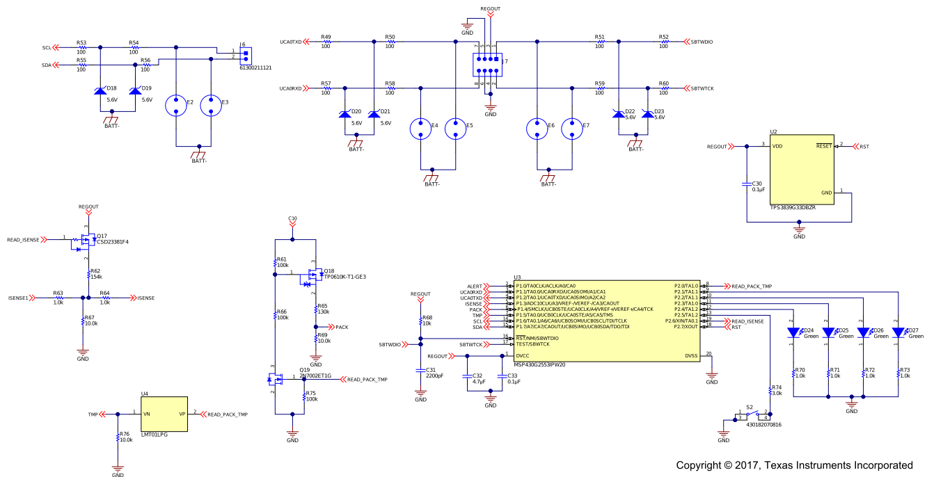
Figure 11. MSP430 Host Example Configuration
