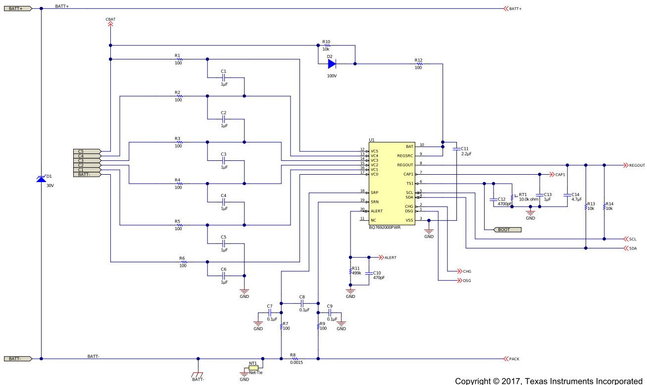
Figure 2. 5S bq76920 Configuration
