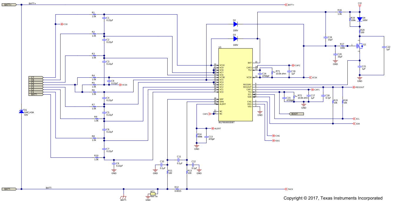
Figure 4. 7S bq76930 Configuration
