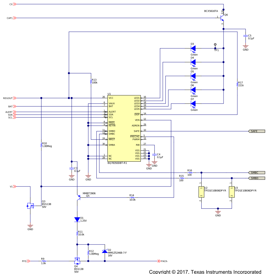
Figure 10. bq78350 configuration for bq76920 and bq76930
