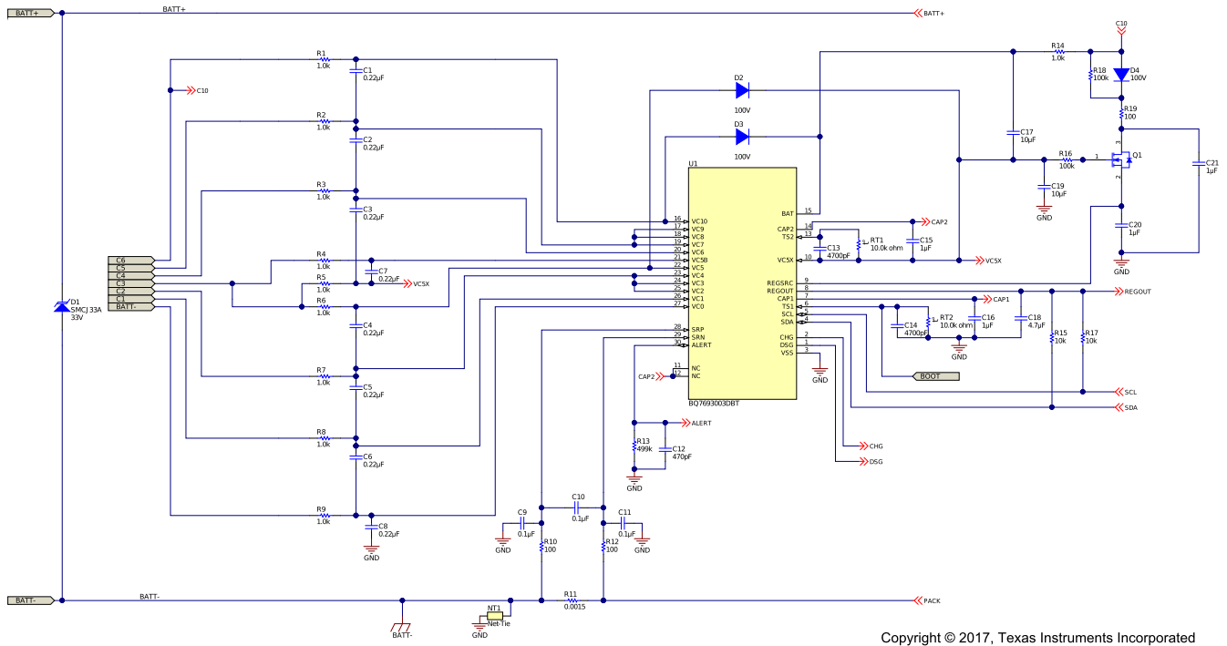
Figure 3. 6S bq76930 Configuration
