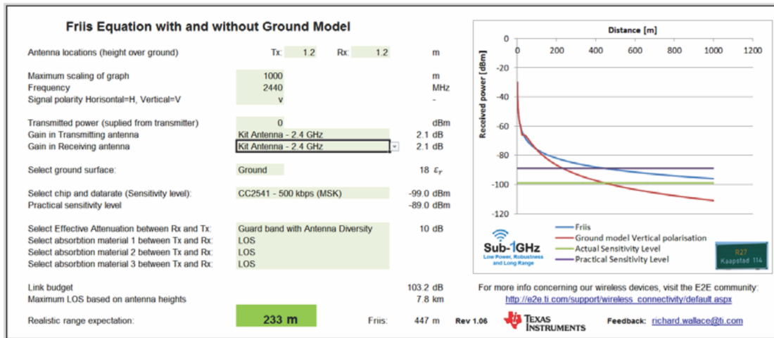
Figure 9. Outdoor LOS, 500 kbps With CC2541 at 2440 MHz; Expected Range 233 m
