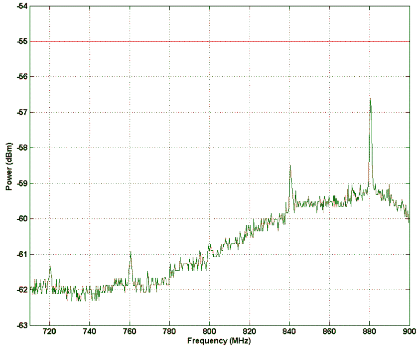
Figure 13. Spurious Emission 710 MHz - 900 MHz
