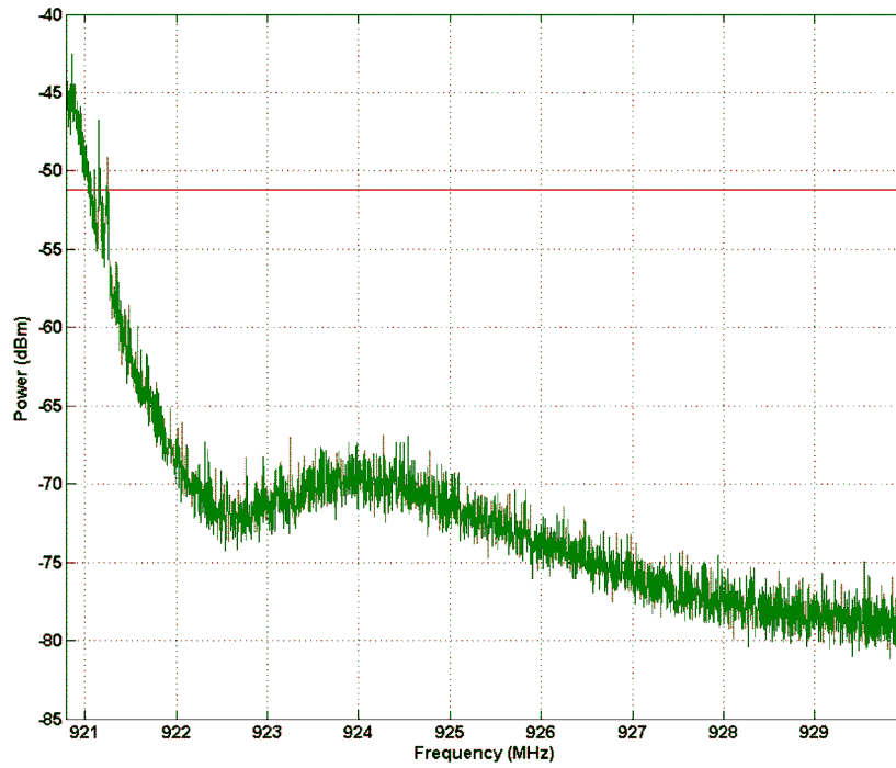
Figure 8. Spurious Emission 920.8 MHz - 930 MHz
