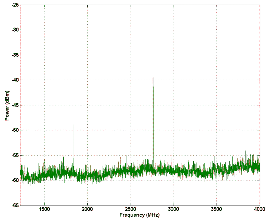
Figure 11. Spurious Emission Above 1215 MHz
