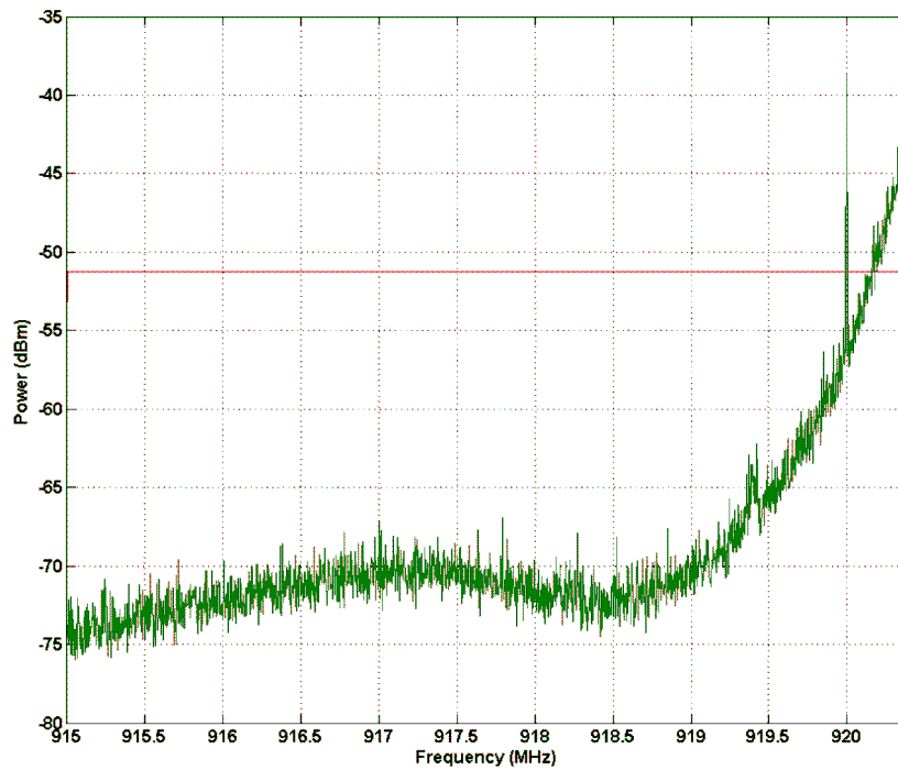
Figure 7. Spurious Emission 915 MHz - 920.4 MHz
