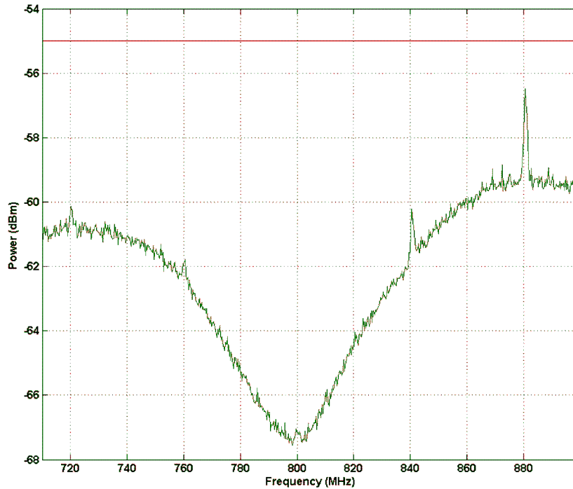
Figure 21. Spurious Emission 710 MHz - 900 MHz
