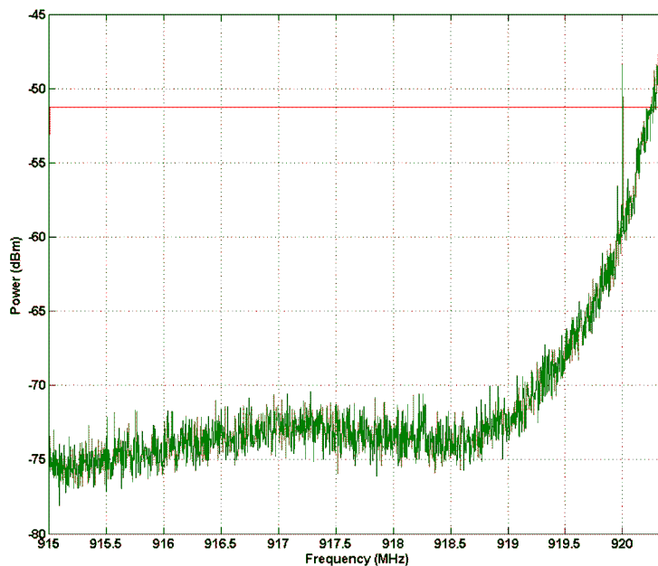
Figure 15. Spurious Emission 915 MHz - 920.4 MHz
