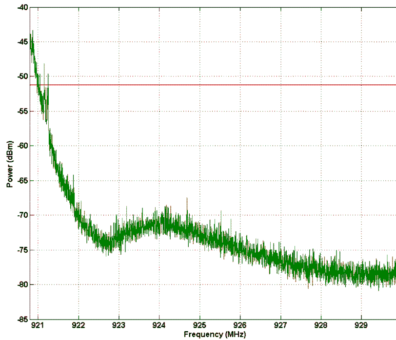
Figure 16. Spurious Emission 920.8 MHz - 930 MHz
