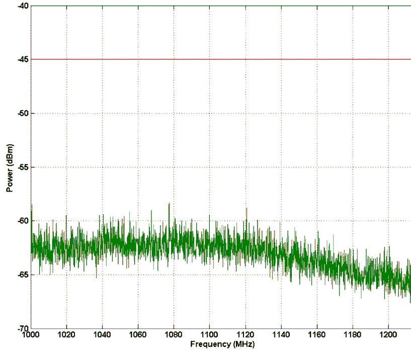
Figure 10. Spurious Emission 1000 MHz - 1215 MHz
