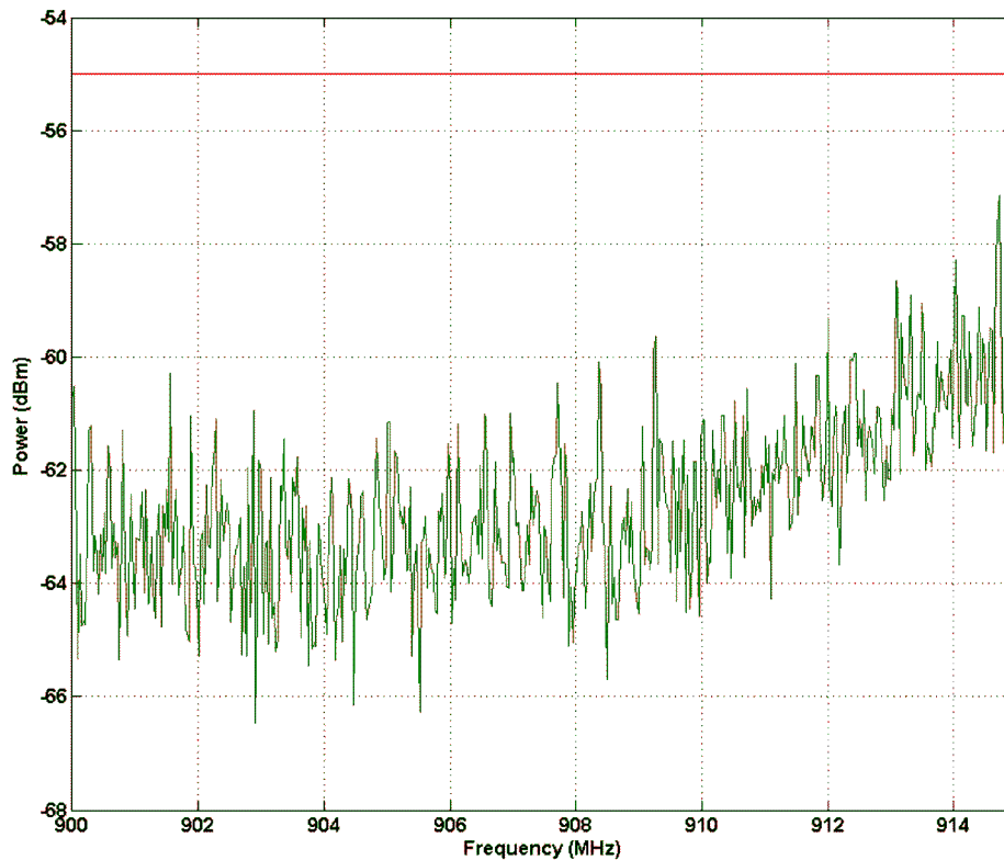
Figure 14. Spurious Emission 900 MHz - 915 MHz
