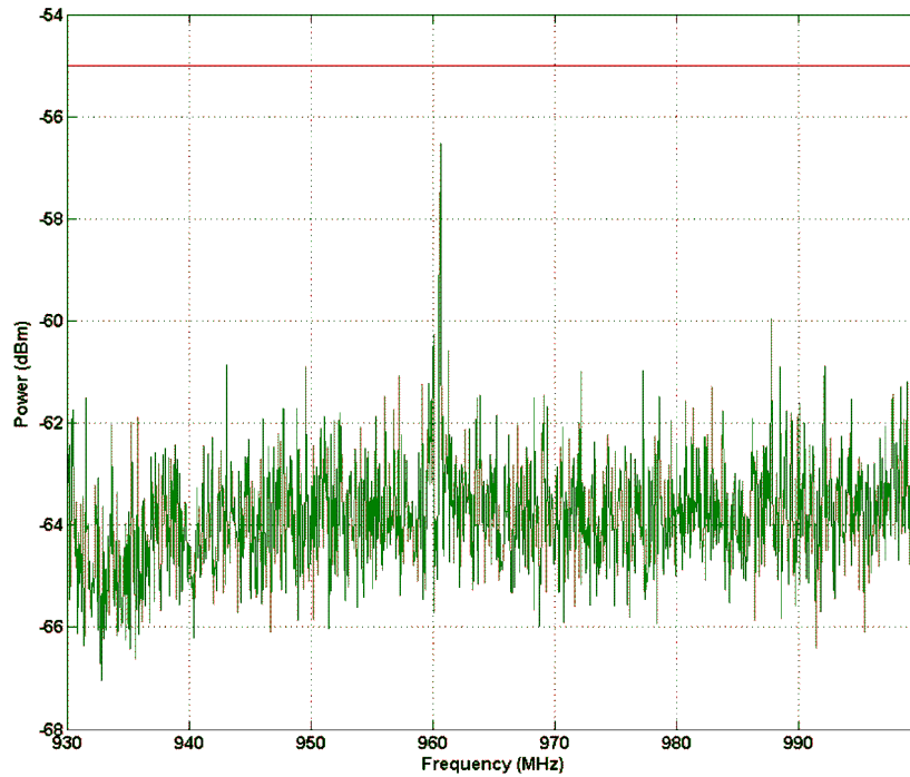
Figure 25. Spurious Emission 930 MHz - 1000 MHz
