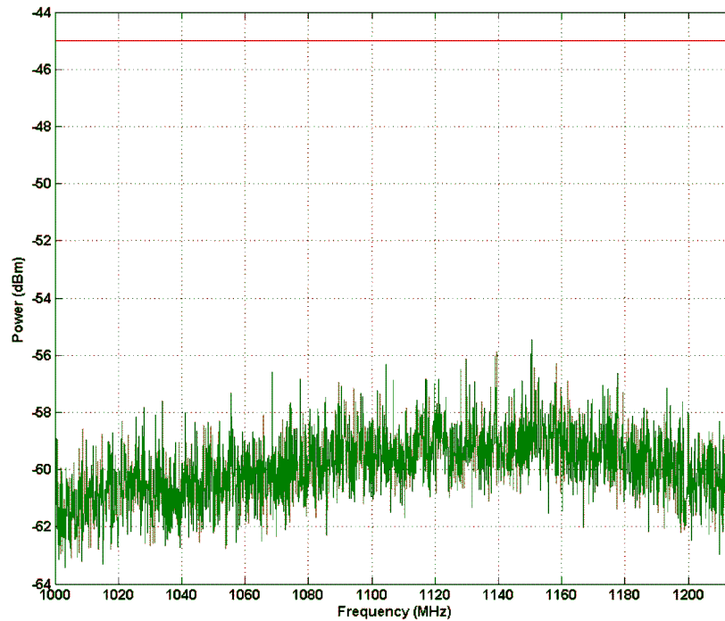
Figure 18. Spurious Emission 1000 MHz - 1215 MHz
