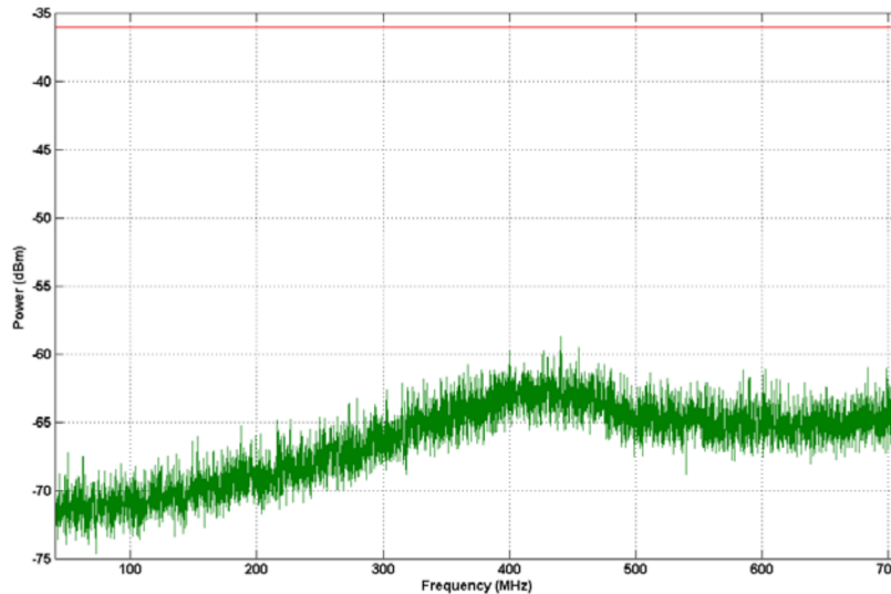
Figure 20. Spurious Emission 40 MHz - 710 MHz
