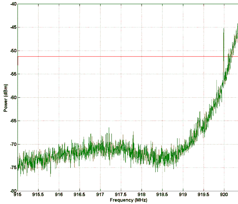
Figure 23. Spurious Emission 915 MHz - 920.4 MHz
