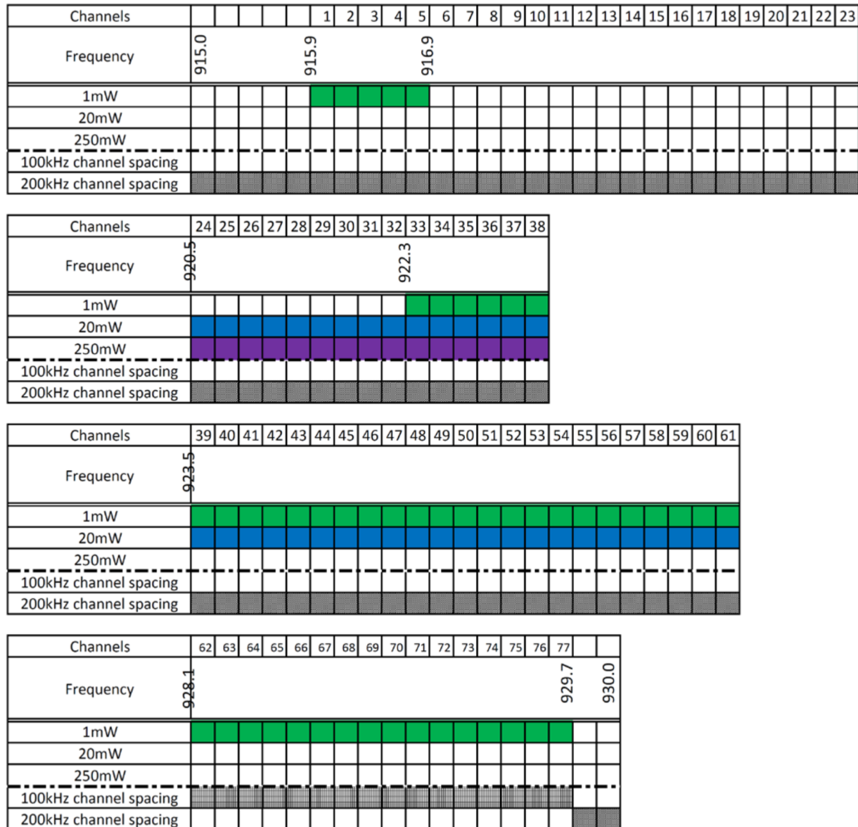
Figure 3. Channel Plan for 920 MHz Band Radio Equipment
