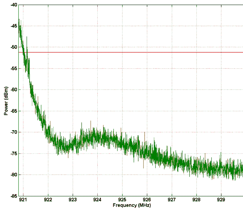
Figure 24. Spurious Emission 920.8 MHz - 930 MHz
