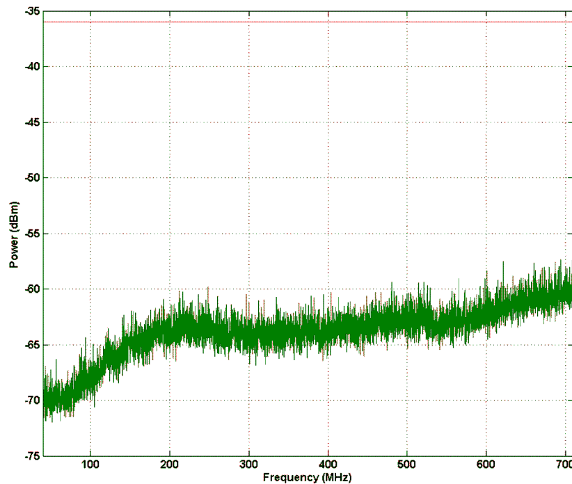
Figure 4. Spurious Emission 40 MHz - 710 MHz
