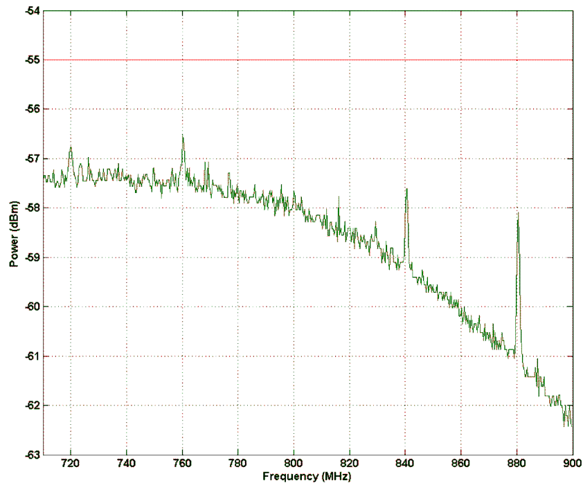
Figure 5. Spurious Emission 710 MHz - 900 MHz
