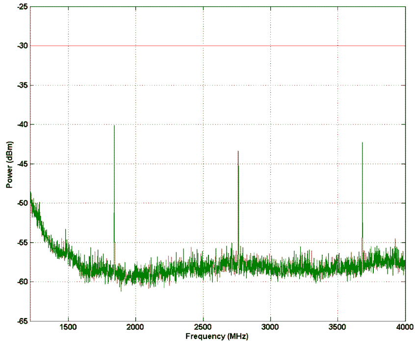
Figure 19. Spurious Emission Above 1215 MHz
