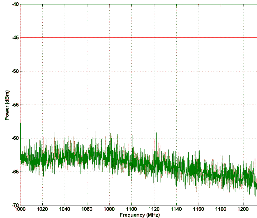
Figure 26. Spurious Emission 1000 MHz - 1215 MHz
