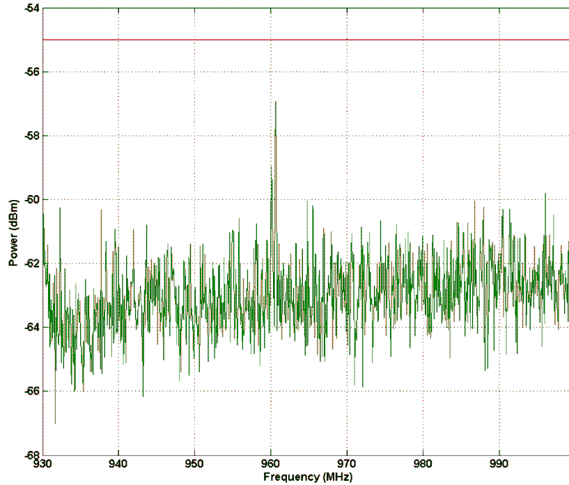
Figure 17. Spurious Emission 930 MHz - 1000 MHz
