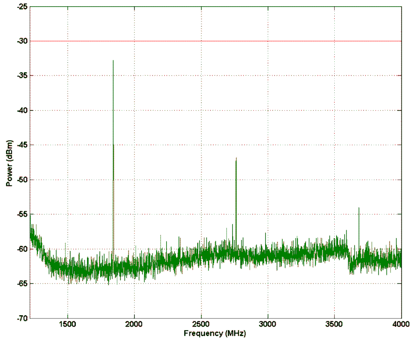
Figure 27. Spurious Emission Above 1215 MHz
