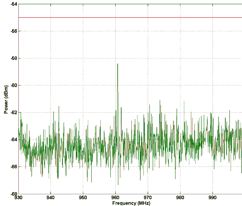
Figure 9. Spurious Emission 930 MHz - 1000 MHz
