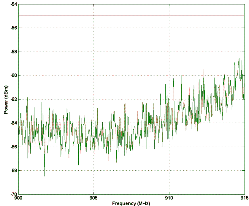
Figure 6. Spurious Emission 900 MHz - 915 MHz
