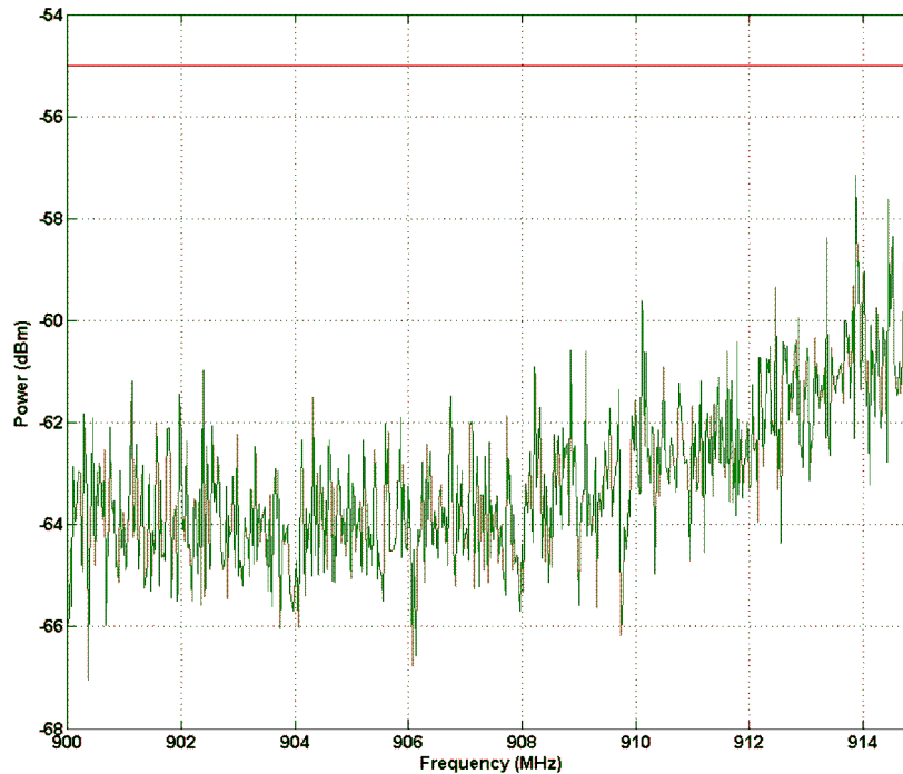
Figure 22. Spurious Emission 900 MHz - 915 MHz
