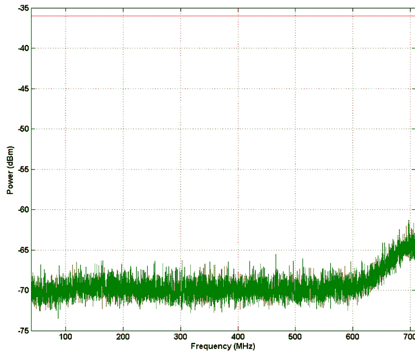
Figure 12. Spurious Emission 40 MHz - 710 MHz
