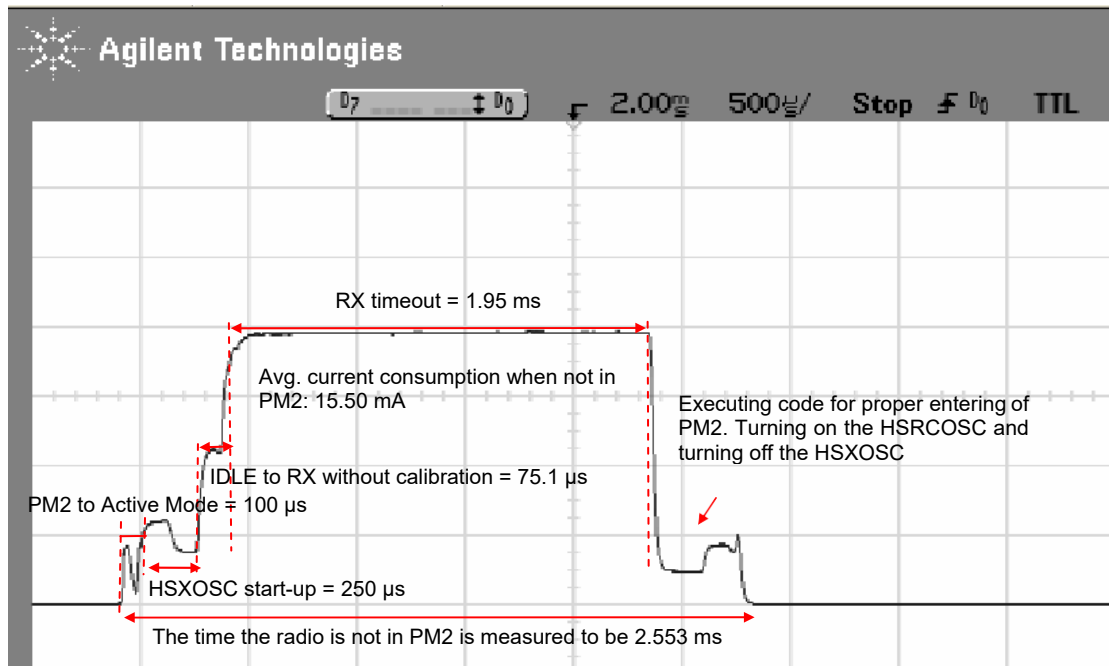
Figure 36. Current Consumption Test Case 11
