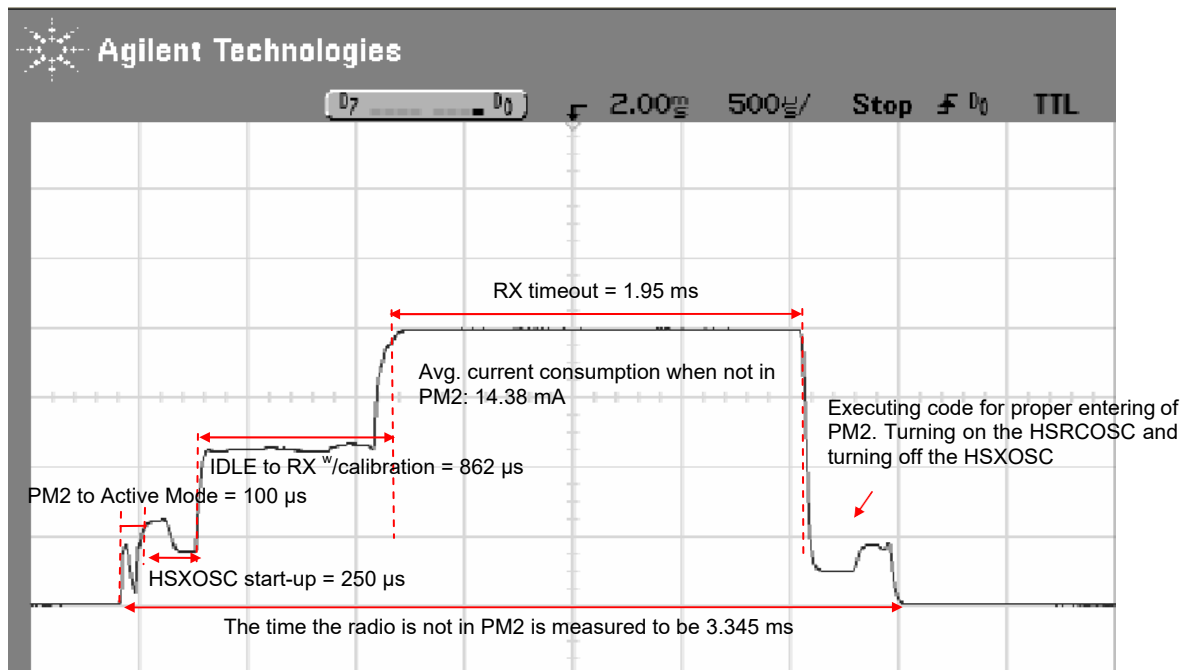
Figure 35. Current Consumption Test Case 10
