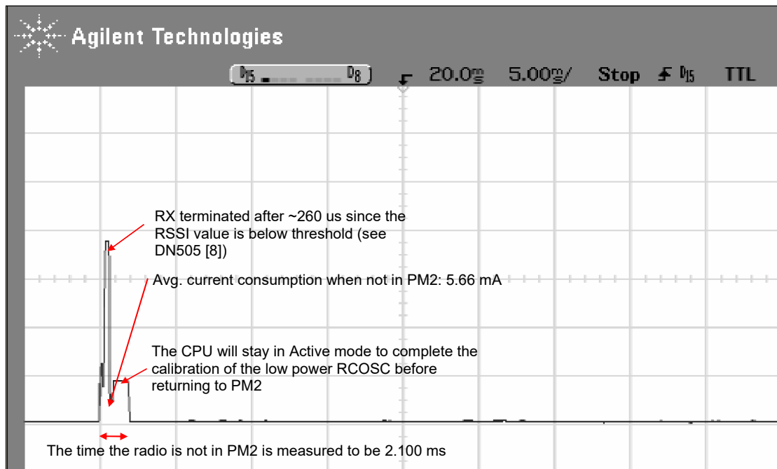
Figure 31. Current Consumption Test Case 9
