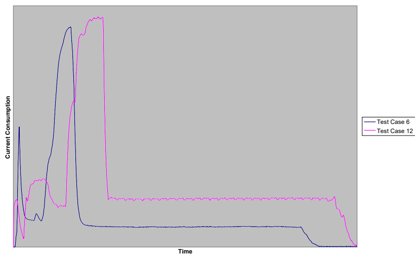
Figure 40. CC2500 vs. CC2510Fx (250 kBaud)
