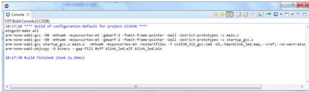
Figure 20. Build Command
