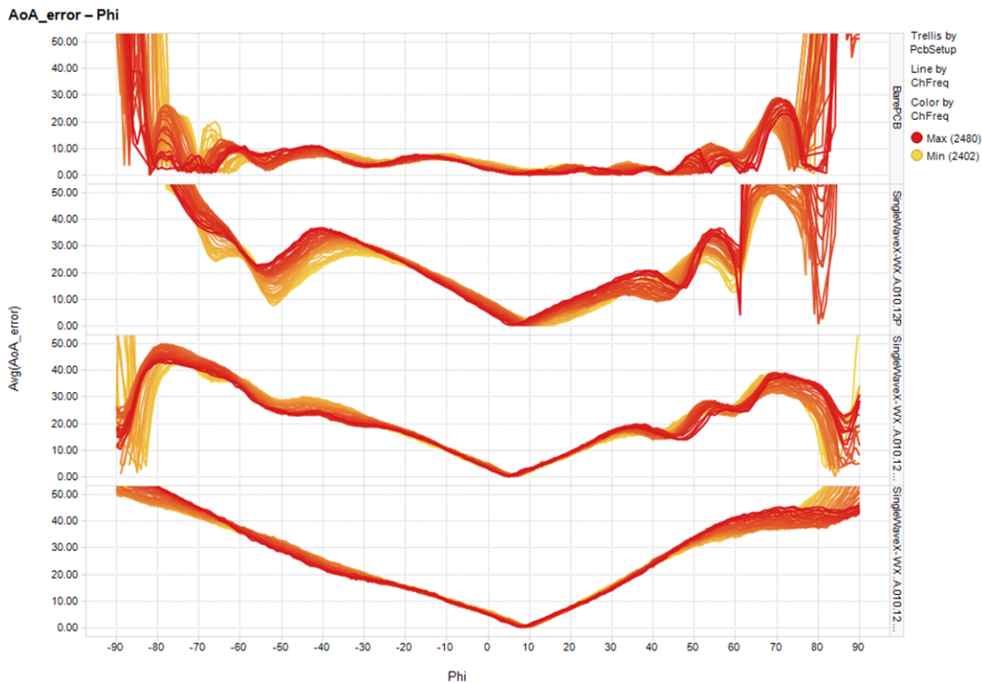
Figure 58. All Hardware AoA Error Results Over all Bluetooth Low Energy Channels
