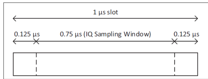
Figure 7. IQ Sampling Window for 1- \mu s Sample Slots
