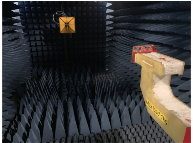
Figure 22. Anechoic Chamber
