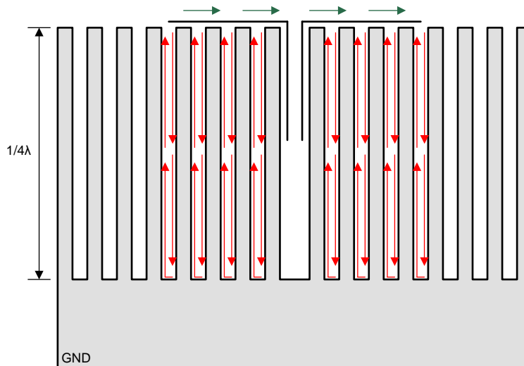
Figure 10. Boundary Current With Corrugated GND Plane
