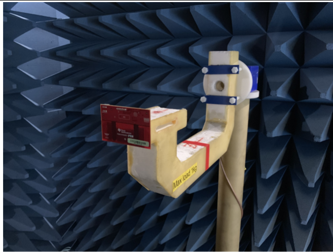
Figure 21. PCB Mounted on Turntable Arm
