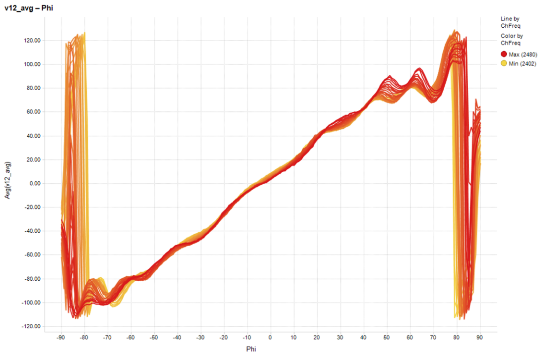
Figure 43. Bare PCB Phase Difference Over Angle Results
