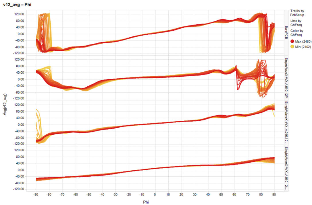
Figure 57. All Hardware AoA Results Over all Bluetooth Low Energy Channels
