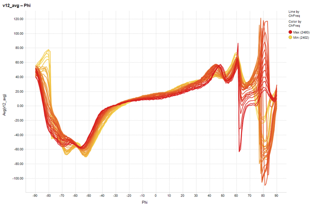
Figure 46. PCB + RF Absorbing Material Phase Difference Over Angle Results
