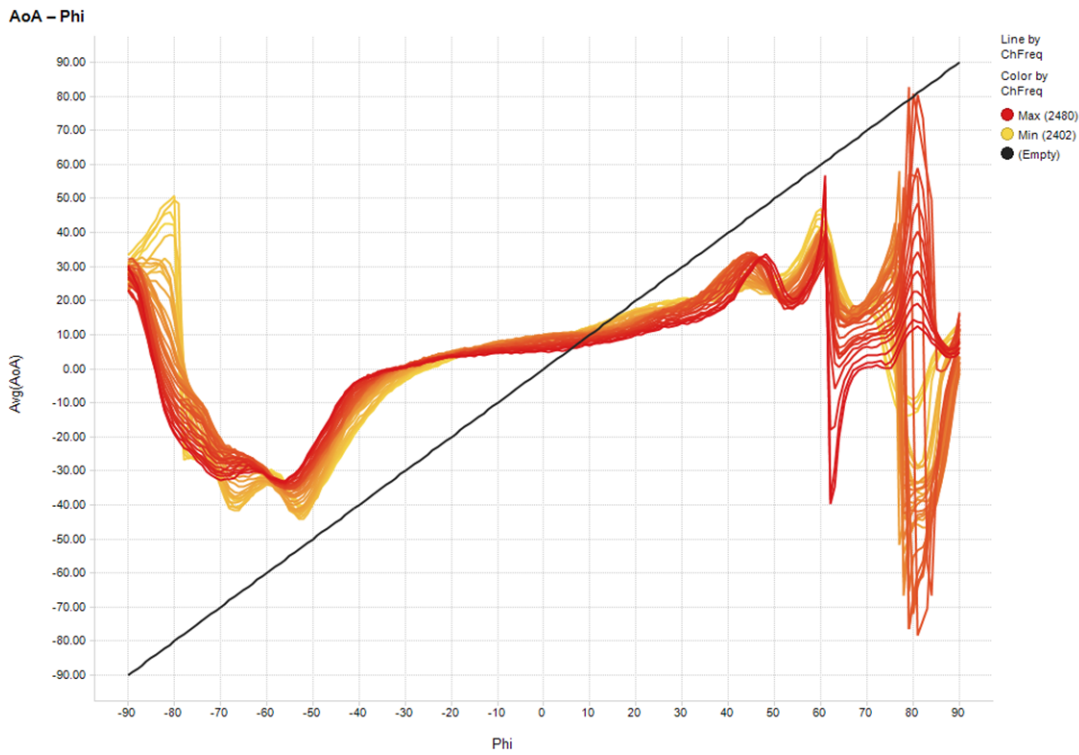
Figure 61. PCB + RF Absorbing Material Uncompensated AoA Over all Bluetooth Low Energy Channels
