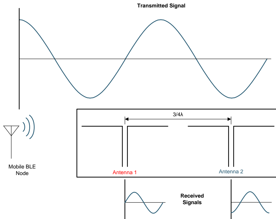
Figure 2. Antenna Array With \frac{3}{4} \lambda Spacing
