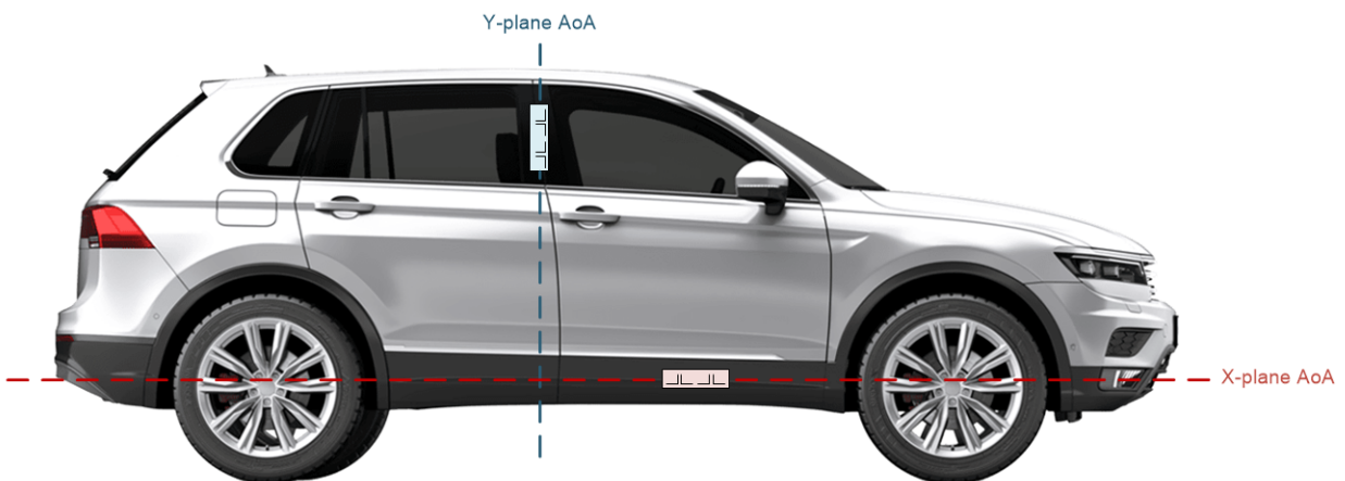
Figure 12. Measuring AoA in Two Planes With Multiple Dipole Antenna Arrays
