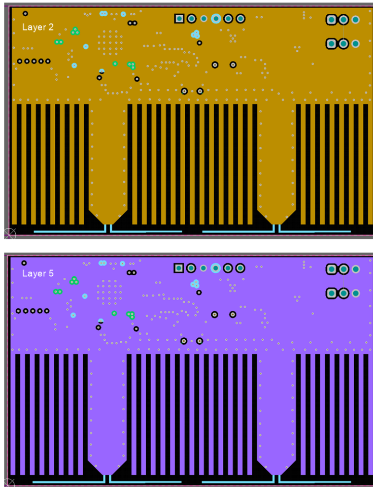
Figure 15. Layer 2 and 5 Ground Planes
