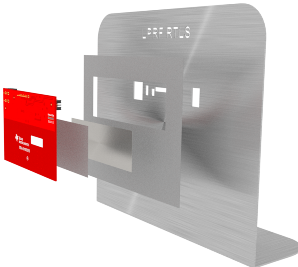
Figure 38. PCB + RF Absorbing Material + Tin-Platted Copper Foil + Metal Stand
