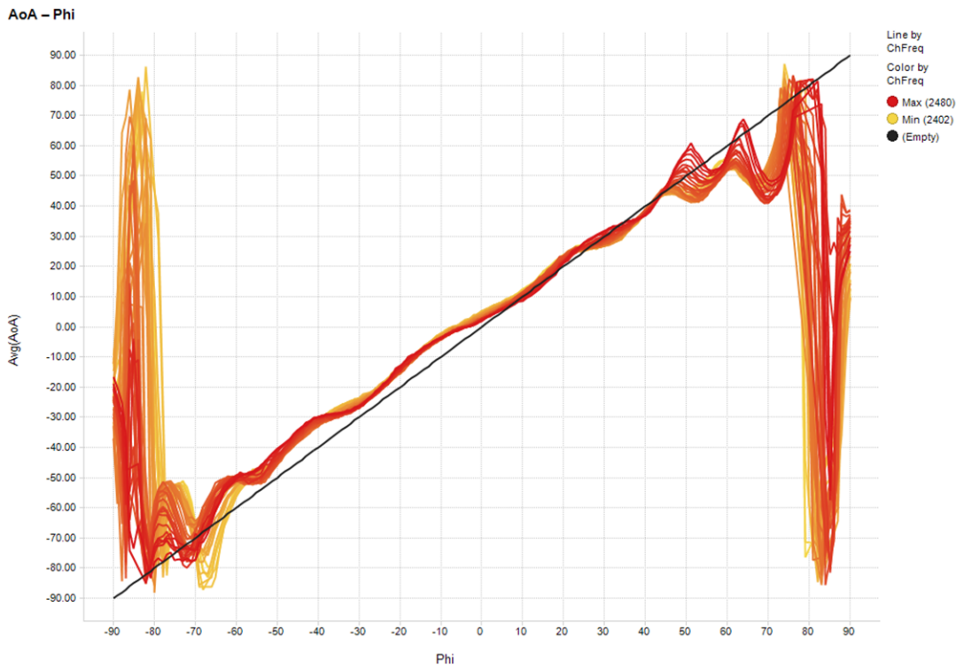
Figure 59. Bare PCB Uncompensated AoA Results Over all Bluetooth Low Energy Channels
