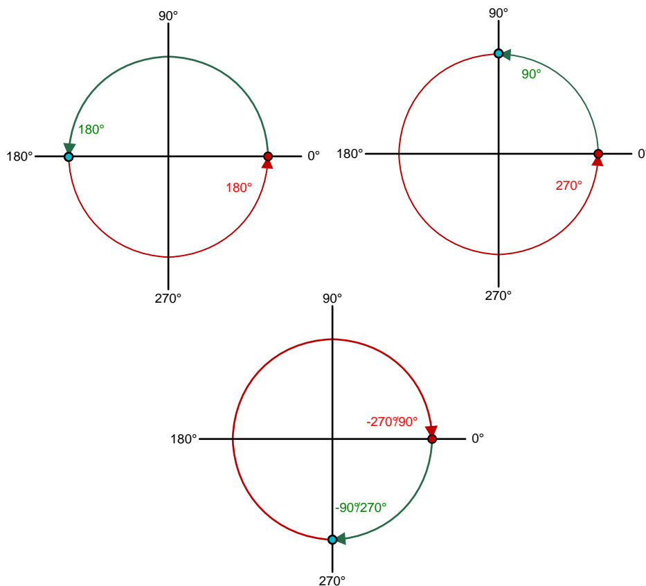
Figure 4. Phasor Diagram with \leq \frac{1}{2} \lambda Antenna Spacing
