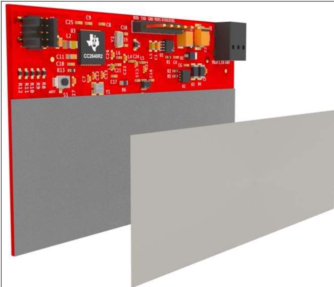
Figure 47. PCB + RF Absorbing Material + Tin-Plated Copper Foil Detached
