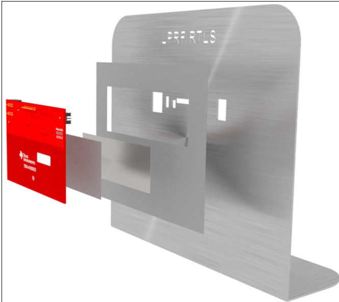
Figure 50. PCB + RF Absorbing Material + Tin-Plated Copper Foil + Metal Individual Pieces
