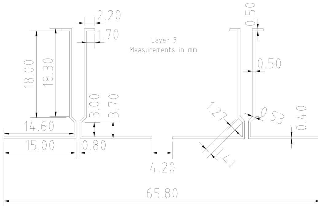
Figure 16. Layer 3 Dipole Antenna Dimensions
