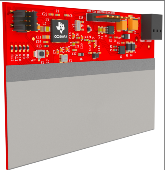
Figure 48. PCB + RF Absorbing Material + Tin-Plated Copper Foil Attached
