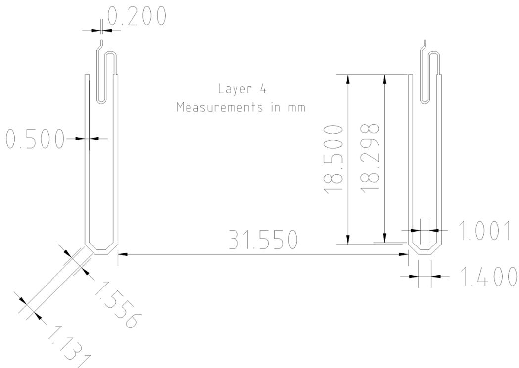
Figure 17. Layer 4 Marchand Balun Dimensions
