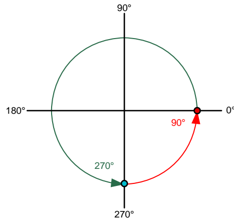
Figure 3. Example Phasor Diagram of \frac{3}{4} \lambda Antenna Spacing
