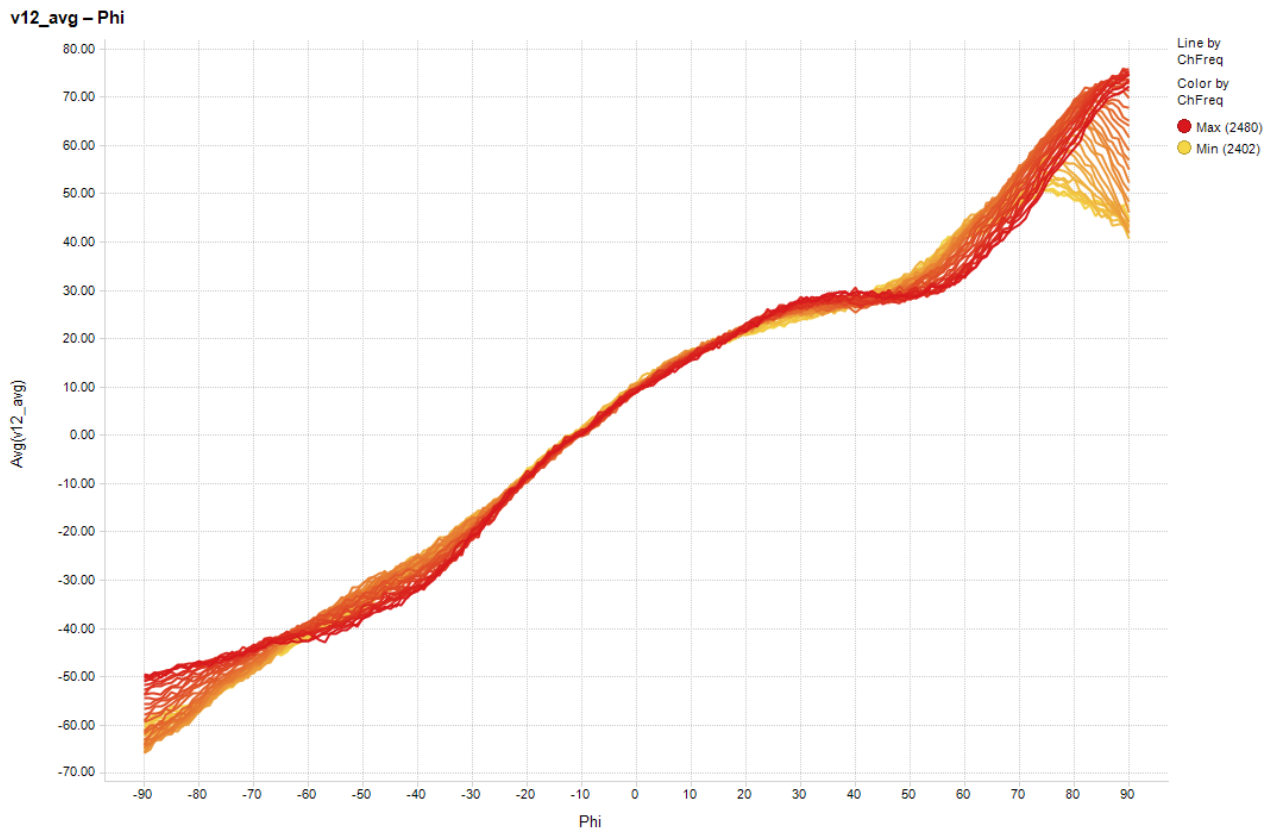
Figure 52. PCB + RF Absorbing Material + Tin-Plated Copper Foil + Metal Phase Difference Over Angle Results
