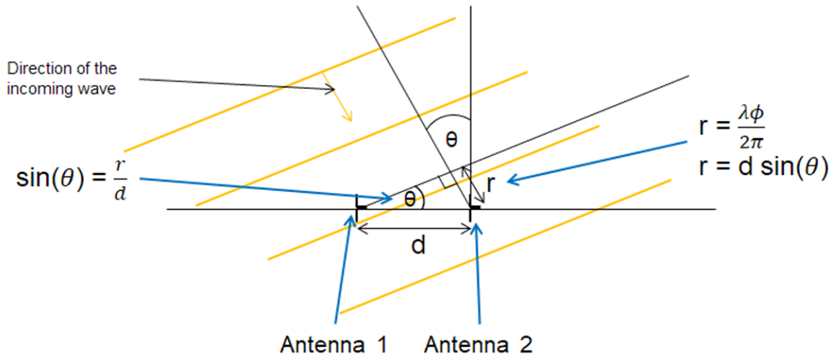
Figure 54. AoA Equations
