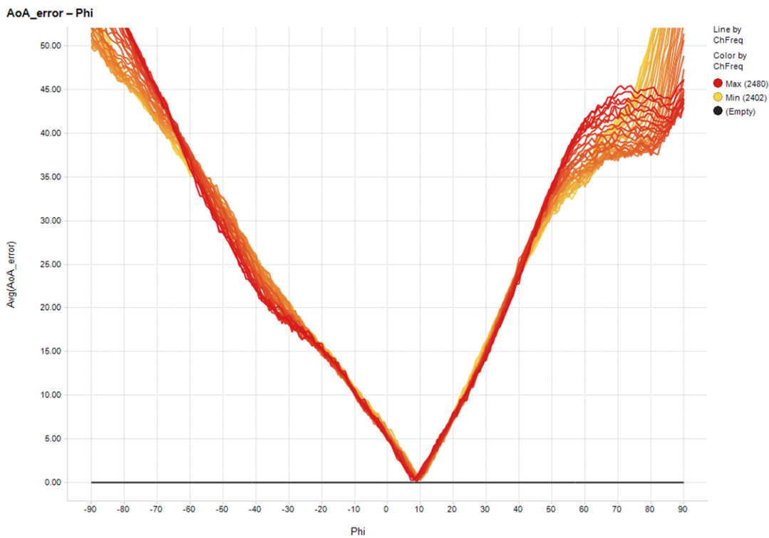
Figure 66. PCB + RF Absorbing Material + Tin-Plated Copper Foil + Metal Uncompensated AoA Error
