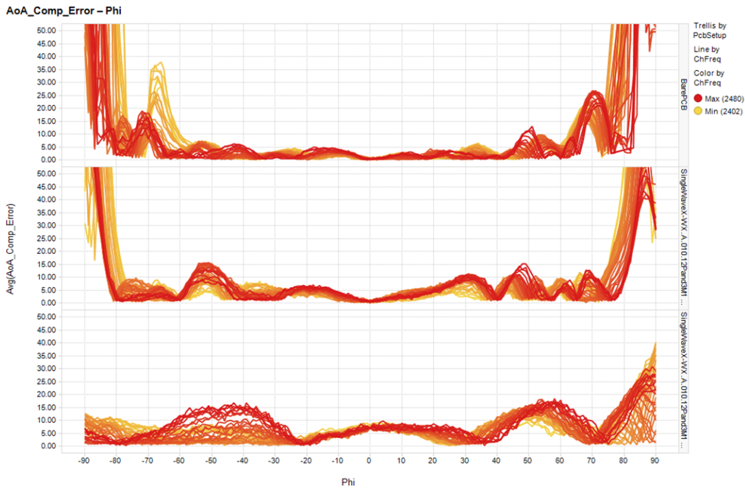
Figure 79. Hardware Setup Comparison: Compensated AoA Error vs Phi
