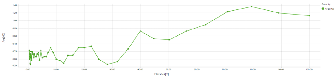
Figure 53. Phase Difference vs Distance
