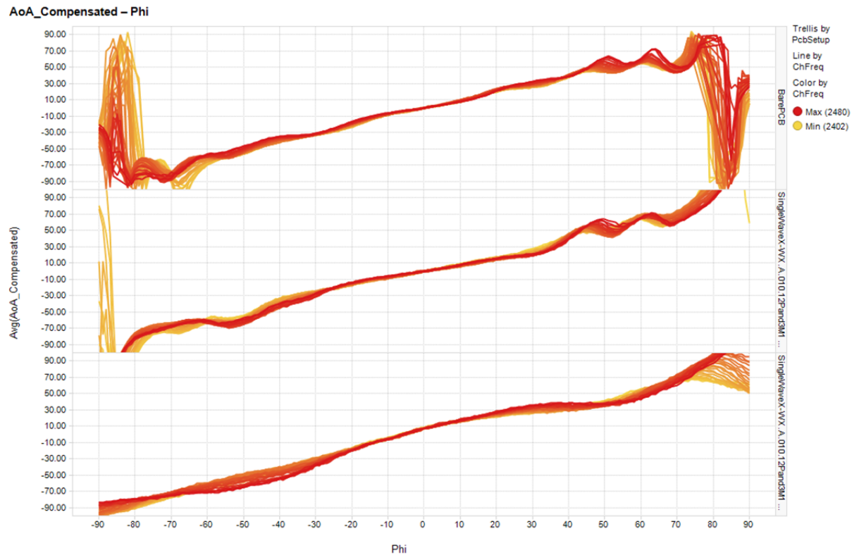
Figure 80. Hardware Setup Comparison: Compensated AoA Results
