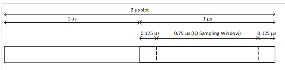
Figure 6. IQ Sampling Window for 2- \mu s Sample Slots
