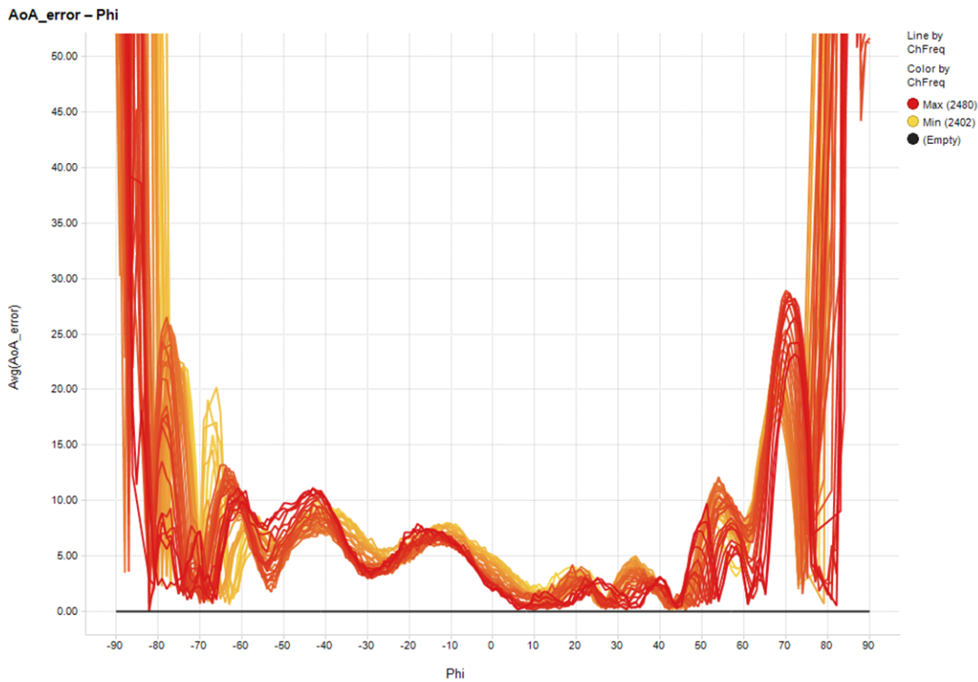
Figure 60. Bare PCB Uncompensated AoA Error Results
