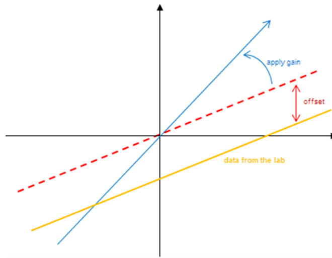
Figure 55. Compensation to Linear Plot
