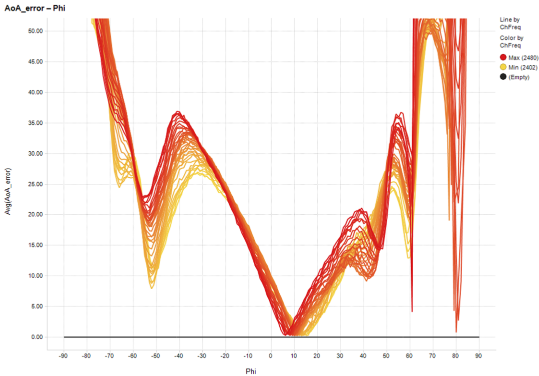
Figure 62. PCB + RF Absorbing Material Uncompensated AoA Error
