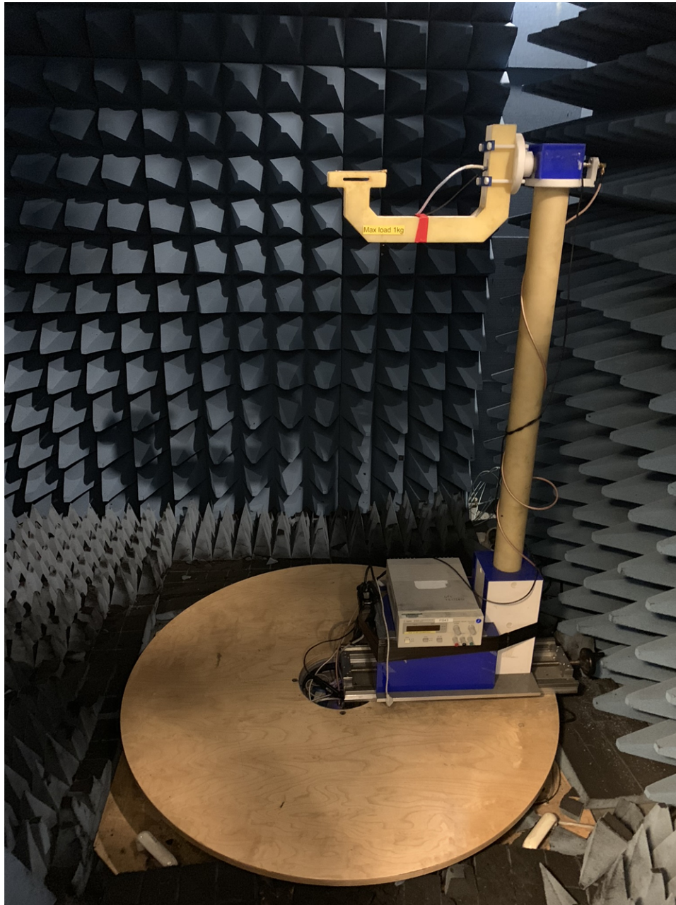
Figure 20. Turntable Test Setup
