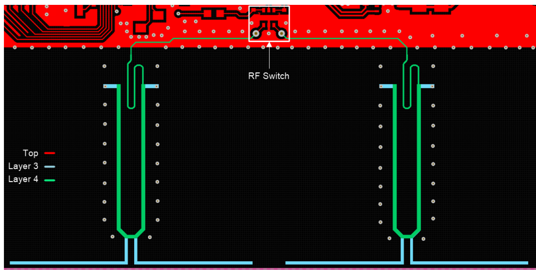
Figure 14. Layer 4 Marchand Balun
