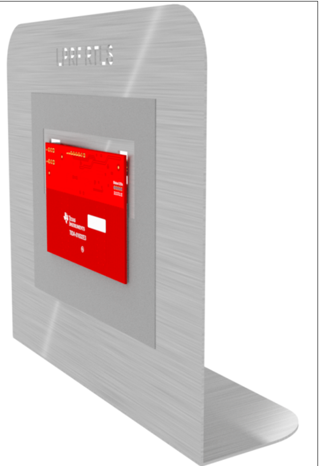
Figure 51. PCB + RF Absorbing Material + Tin-Plated Copper Foil + Metal
