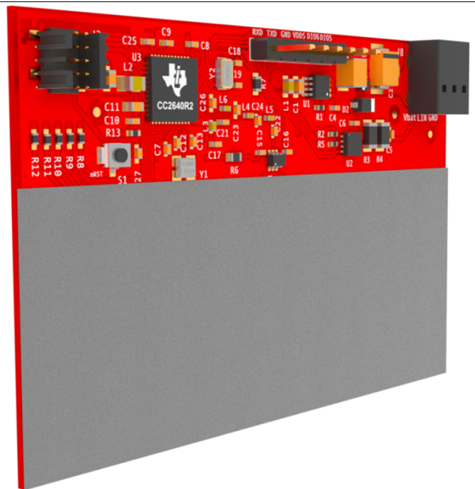
Figure 45. PCB + RF Absorbing Material Attached
