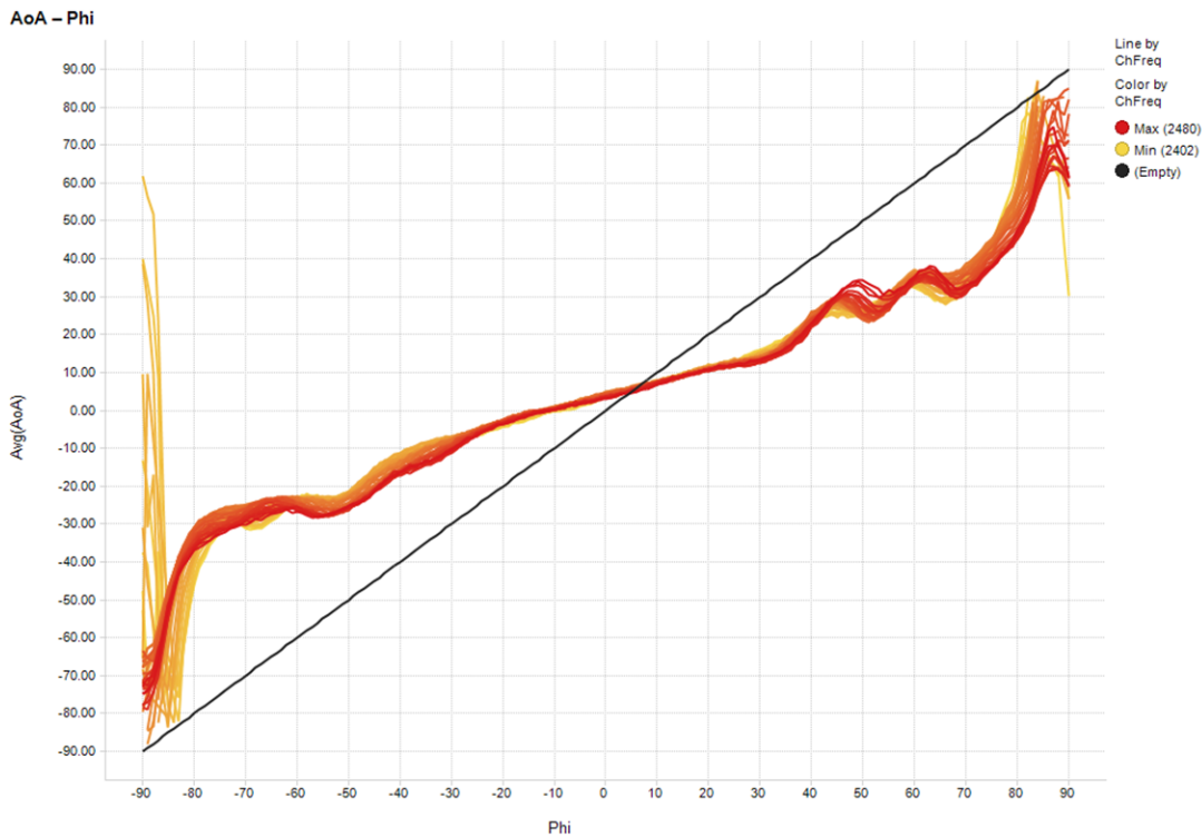
Figure 63. PCB + RF Absorbing Material + Tin-Plated Copper Foil Uncompensated AoA Results Over all Bluetooth Low Energy Channels
