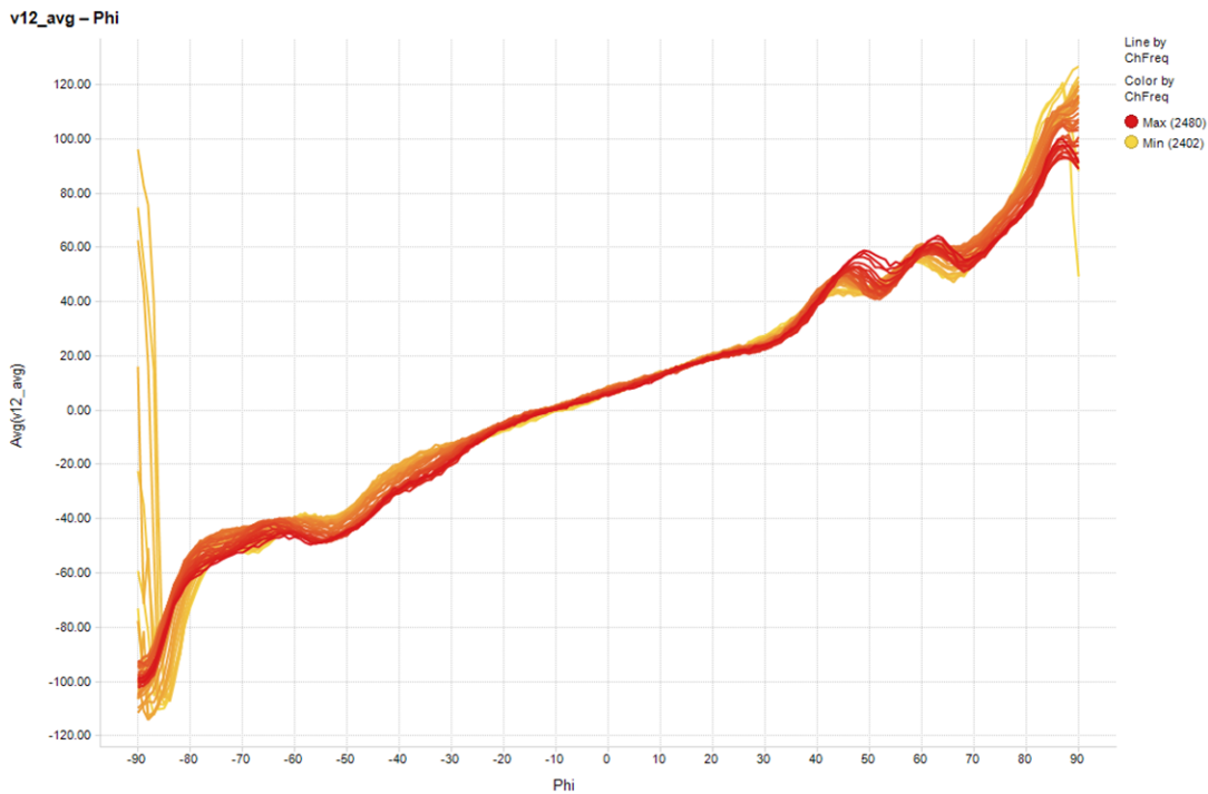
Figure 49. PCB + RF Absorbing Material + Tin-Plated Copper Foil Phase Difference Over Angle Results
