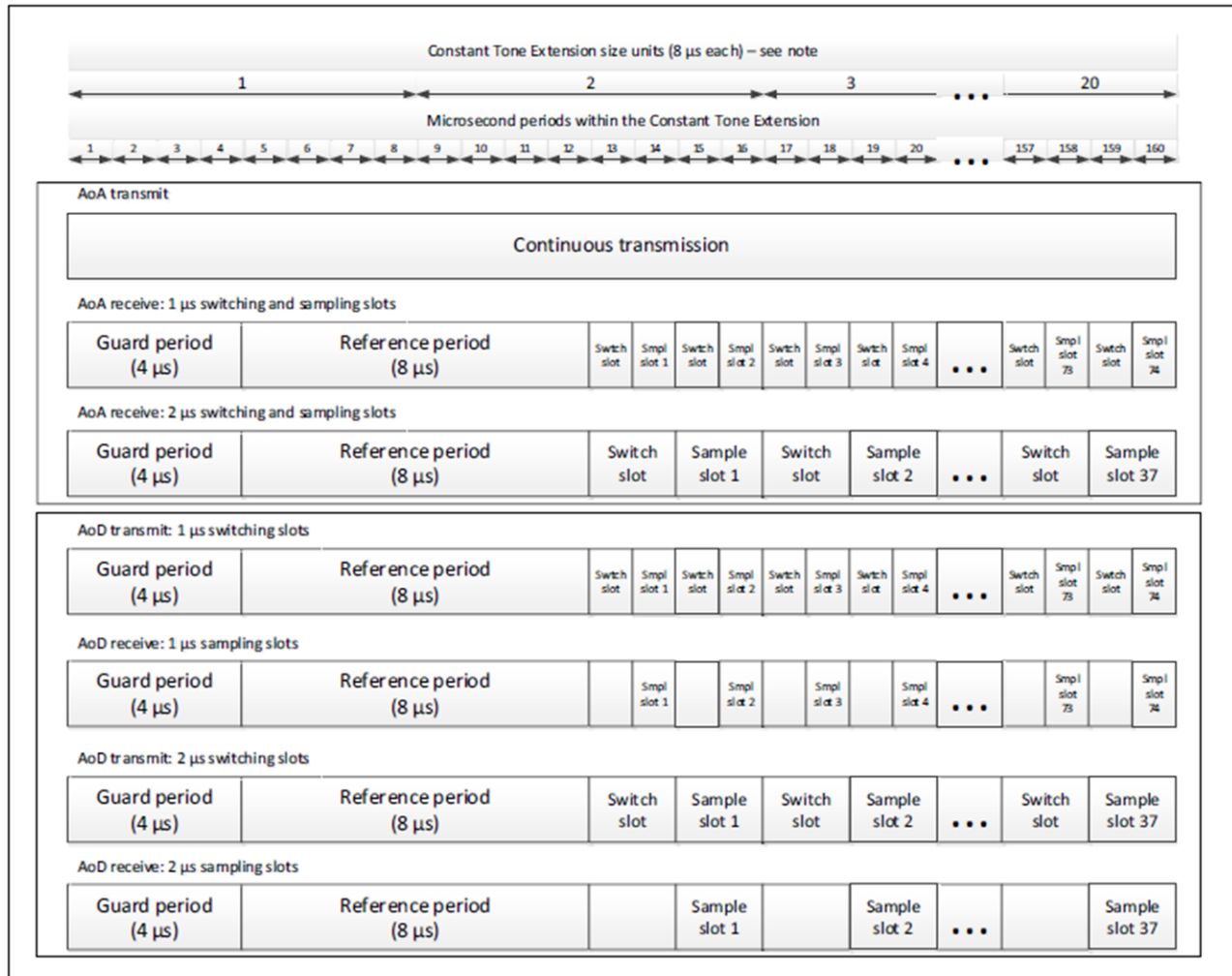
Figure 5. Constant Tone Extension Structure Bluetooth Specification v5.1
