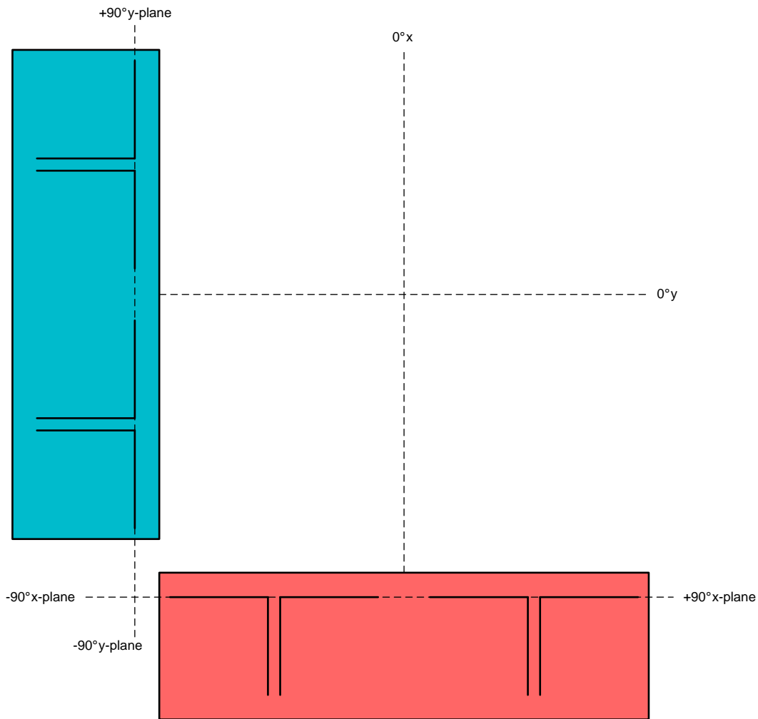
Figure 11. Antenna Array Orientation
