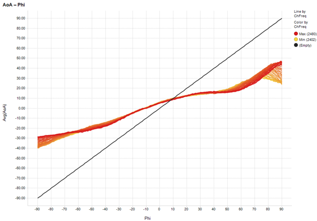
Figure 65. PCB + RF Absorbing Material + Tin-Plated Copper Foil + Metal Uncompensated AoA Results Over all Bluetooth Low Energy Channels
