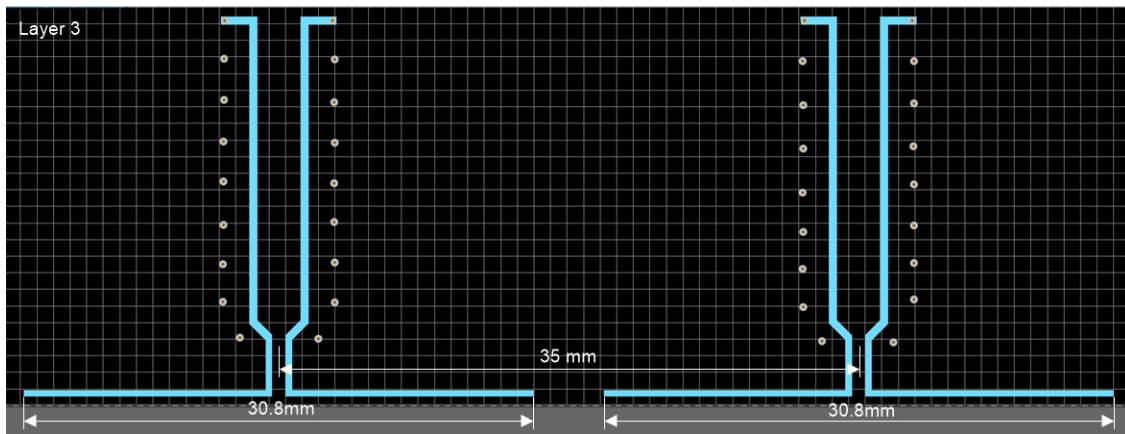
Figure 13. Layer 3 Dipole Spacing and Width
