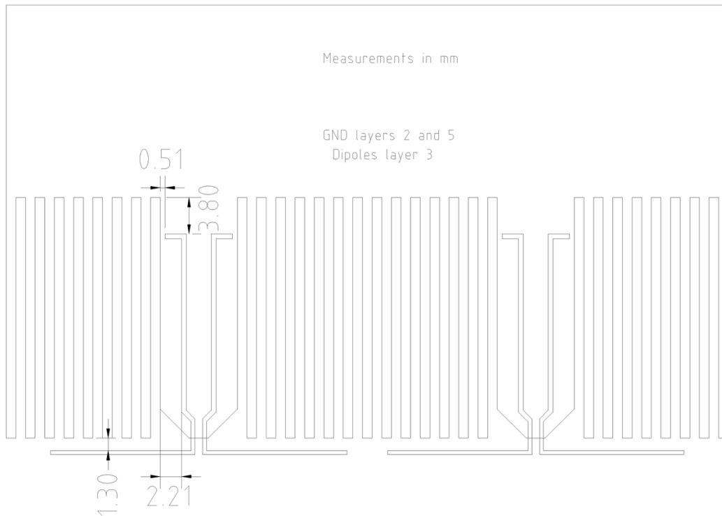
Figure 19. Dipole With Ground Plane Dimensions
