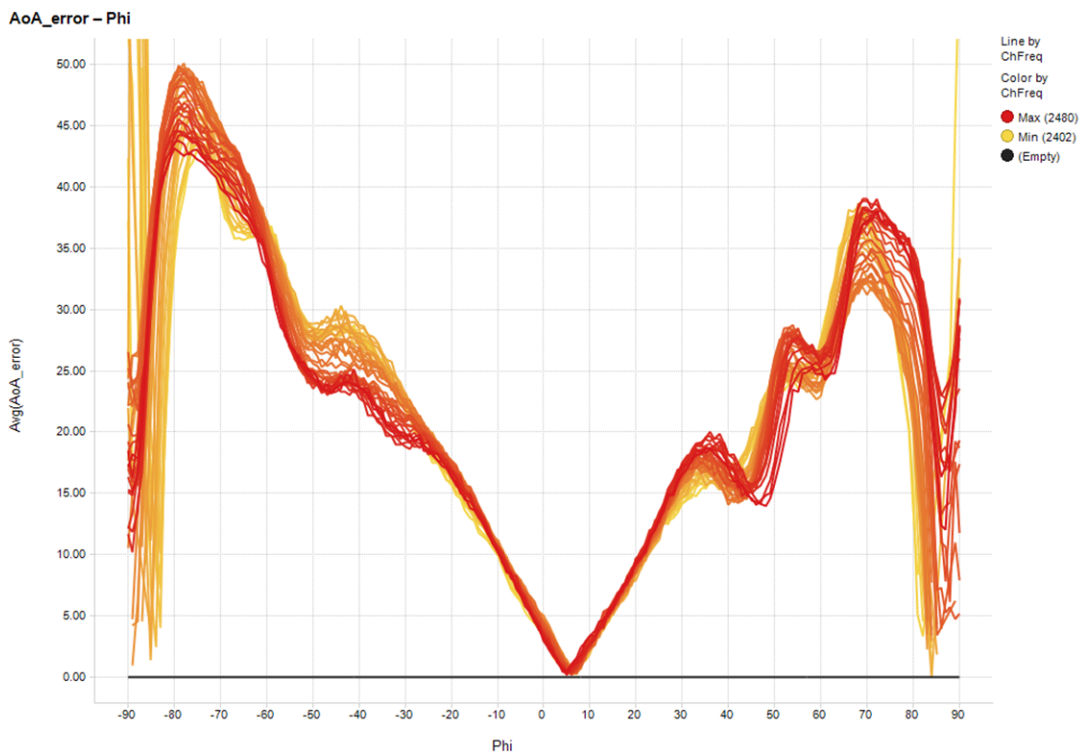
Figure 64. PCB + RF Absorbing Material + Tin-Plated Copper Foil Uncompensated AoA Error
