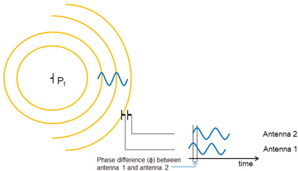
Figure 1. Transmitter Phase Measured by Antenna Array
