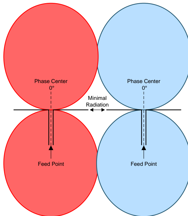
Figure 8. Dipole Antenna Radiation Pattern and Phase Center
