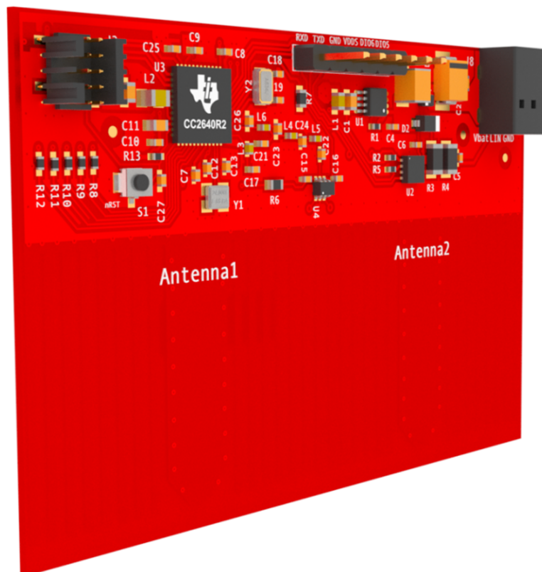
Figure 42. Bare PCB
