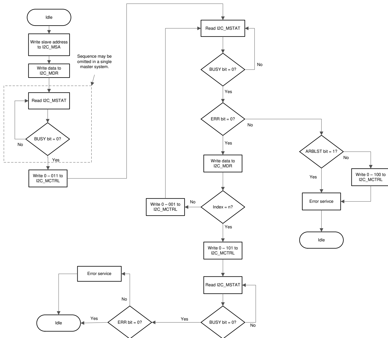
Figure 23-9. Master TRANSMIT With Repeated Start Condition
