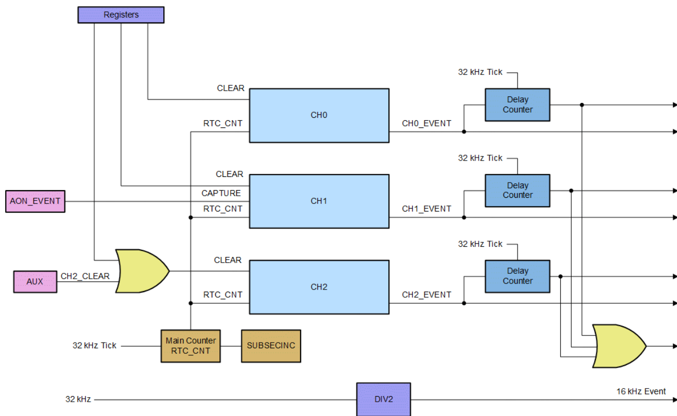
Figure 16-1. AON_RTC Channels
