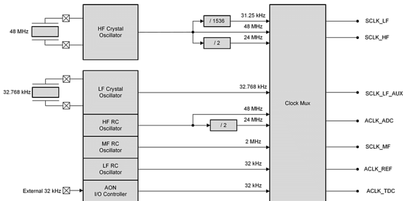
Figure 7-4. Clock Sources
