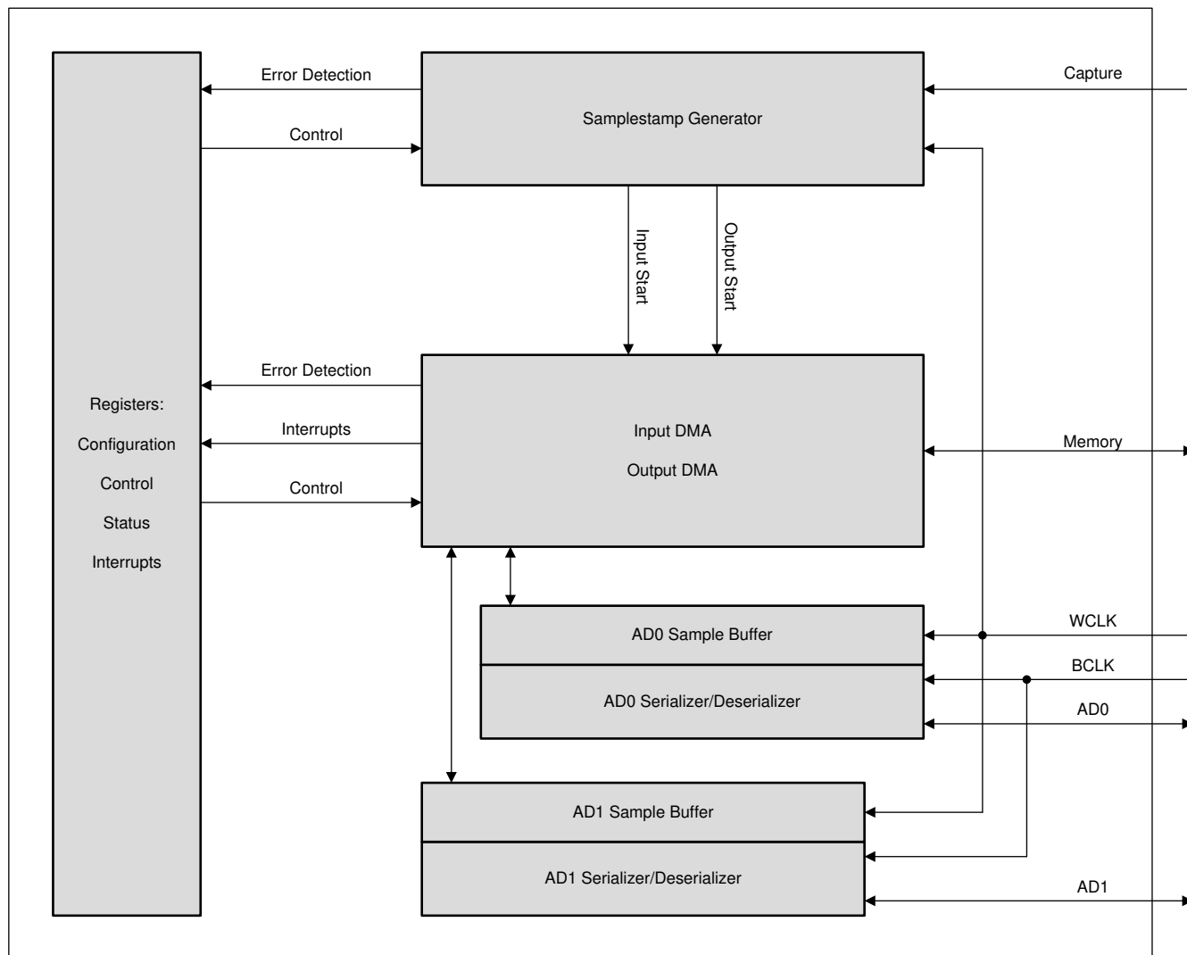
Figure 24-1. Simplified I 2 S Module Block Diagram
