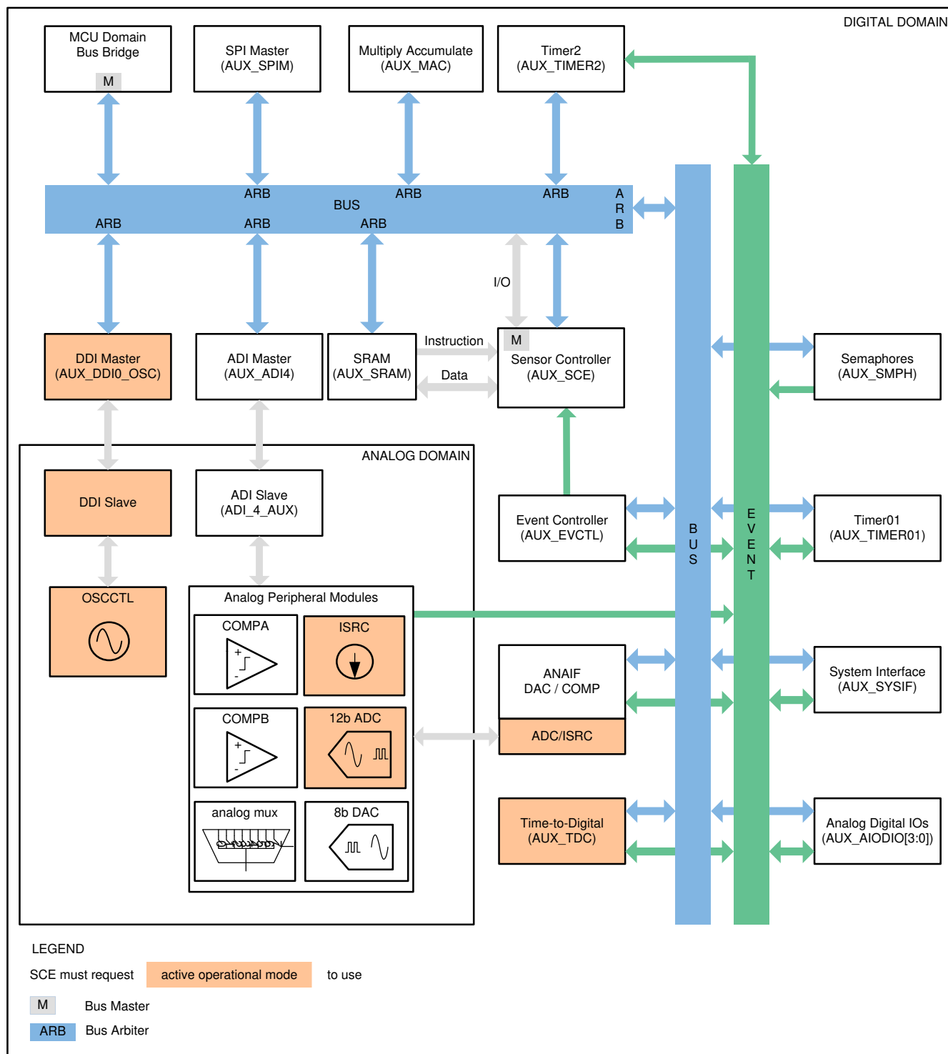
Figure 19-1. AUX Domain Block Diagram
