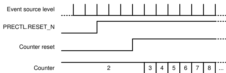
Figure 19-22. Pulse Counting
