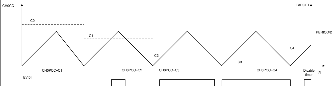
Figure 19-26. Center-Aligned PWM
