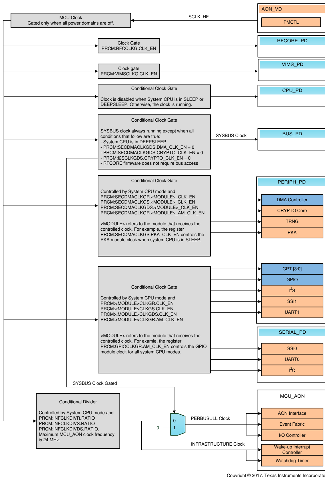
Figure 7-6. Clocks in MCU_VD
