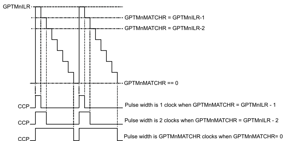
Figure 15-7. CCP Output, GPT:TnILR > GPT:TnMATCHR
