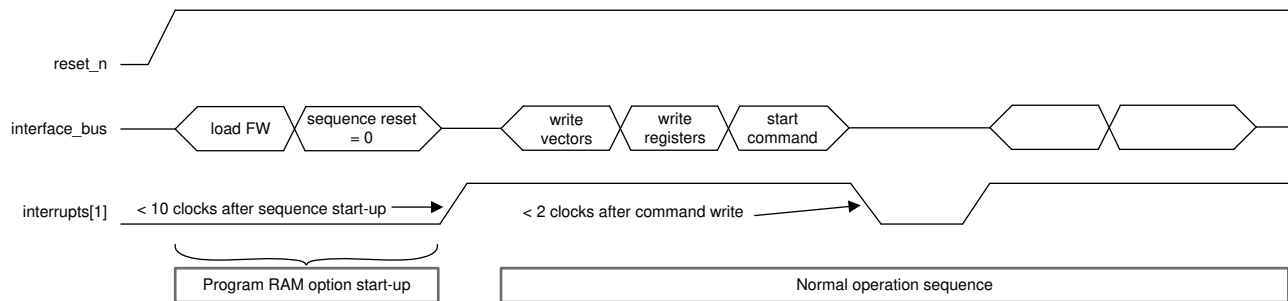
Figure 12-5. Operation Sequence
