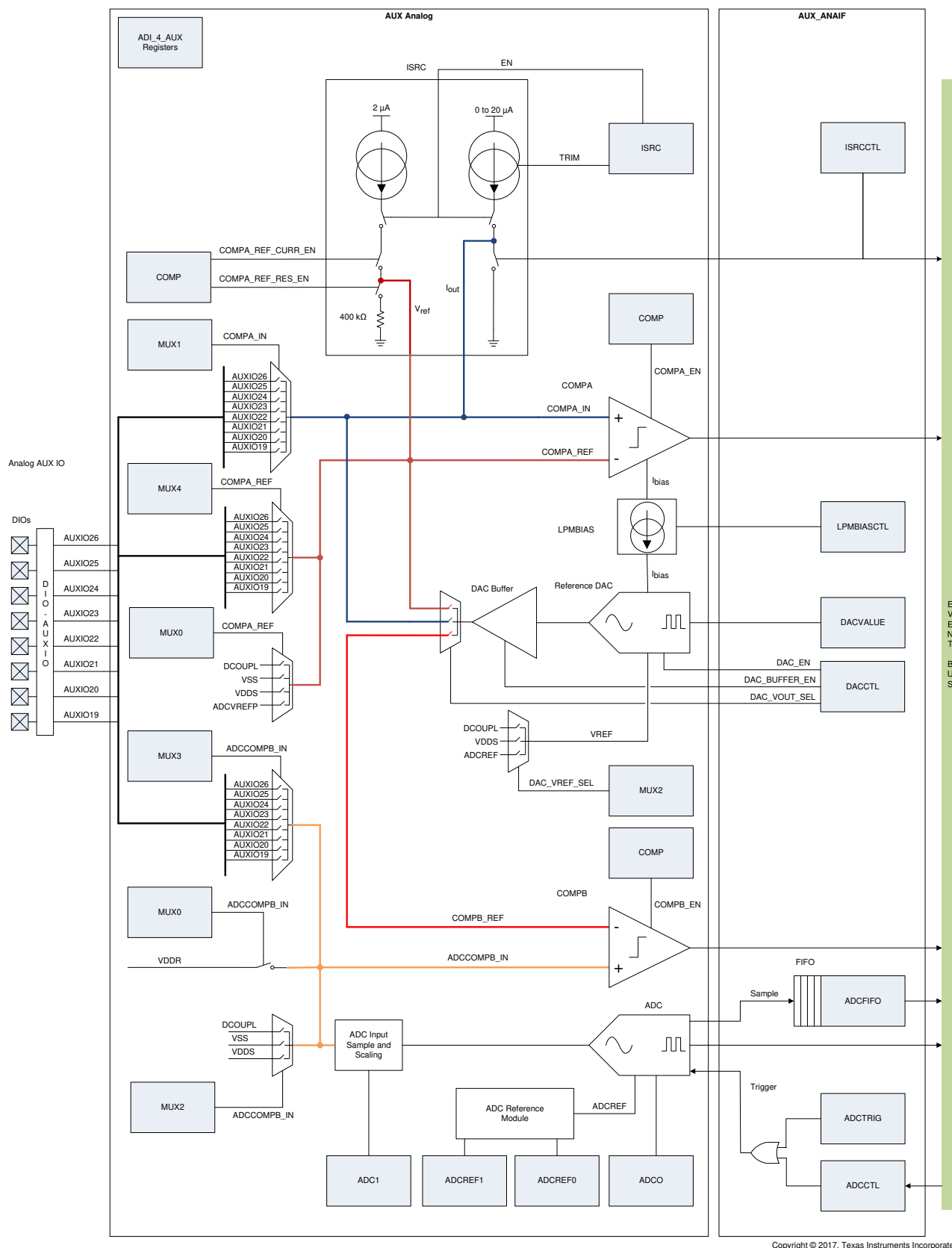
Figure 19-28. AUX Analog Block Diagram
