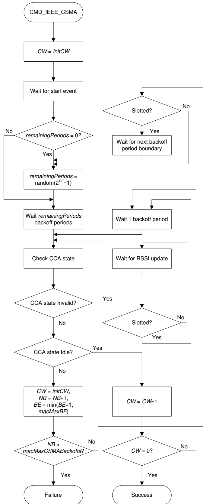
Figure 25-7. CSMA-CA Operation
