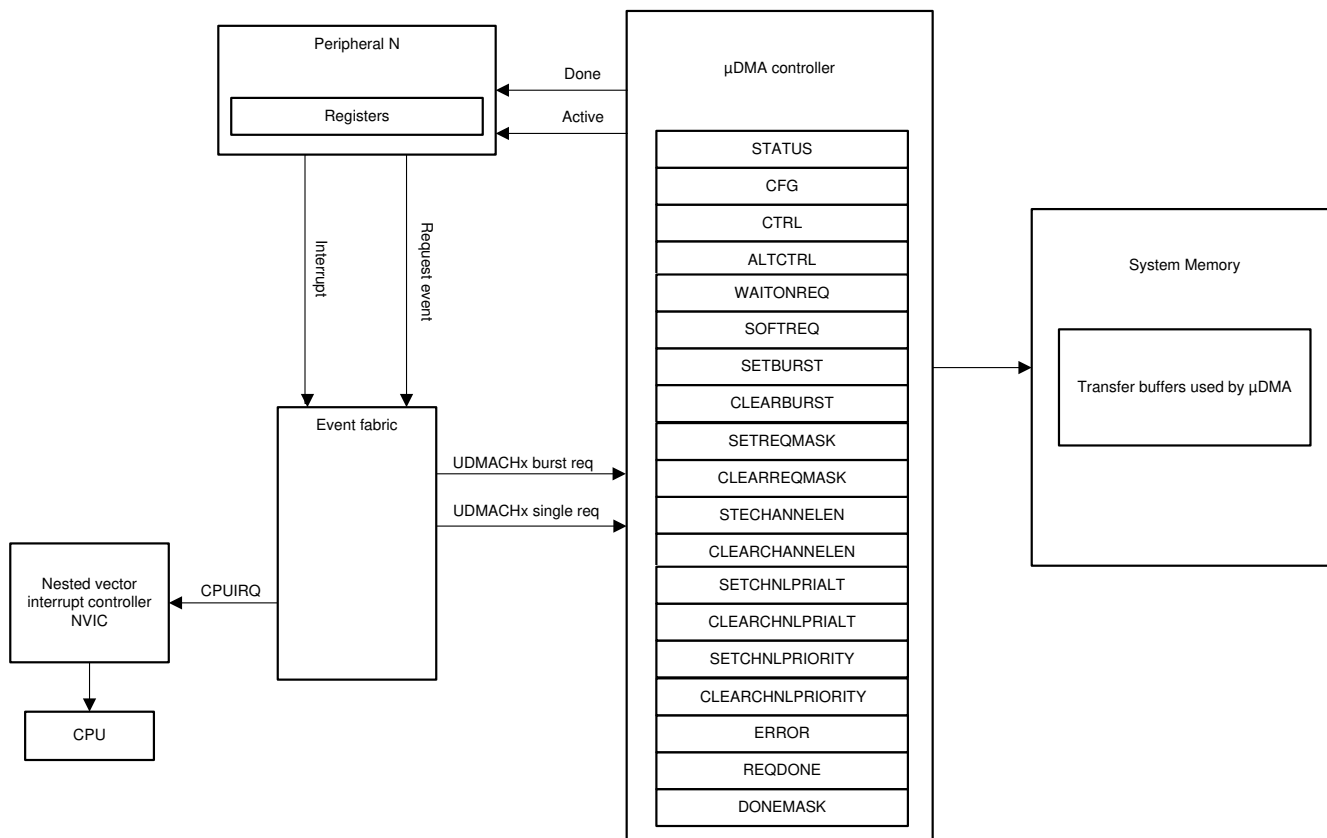
Figure 14-1. \mu DMA Block Diagram
