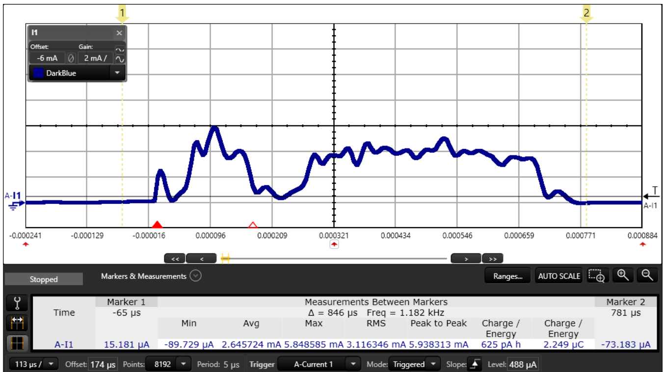
Figure 17. SPI Transfer: One SPI Transmit from the System CPU
