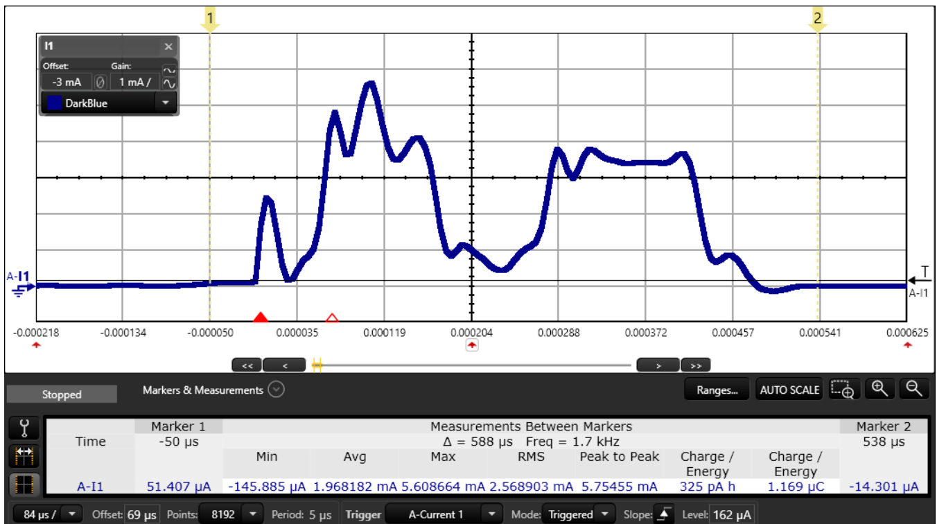
Figure 20. Wake-up: One wake-up of the System CPU
