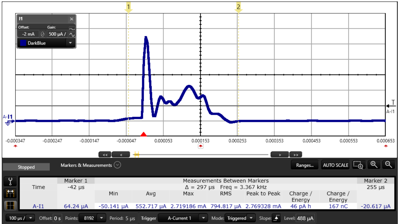
Figure 16. SPI Transfer: One SPI Transmit in Active Mode
