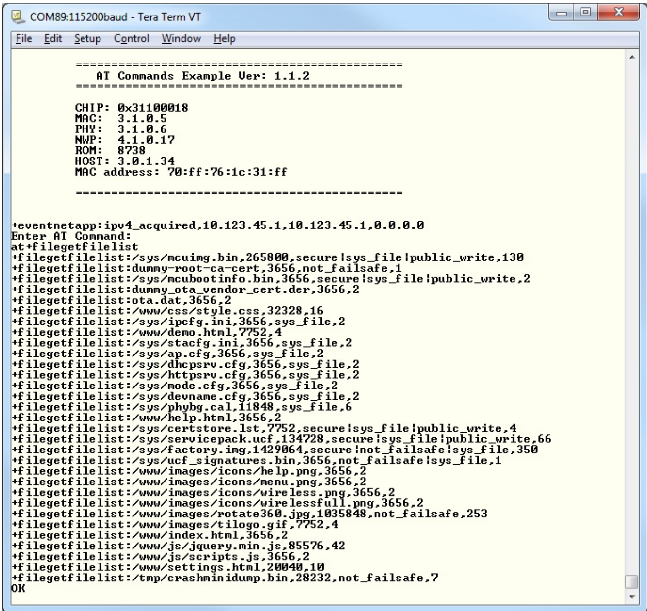
Figure 2-3. File Listing Through Host API
