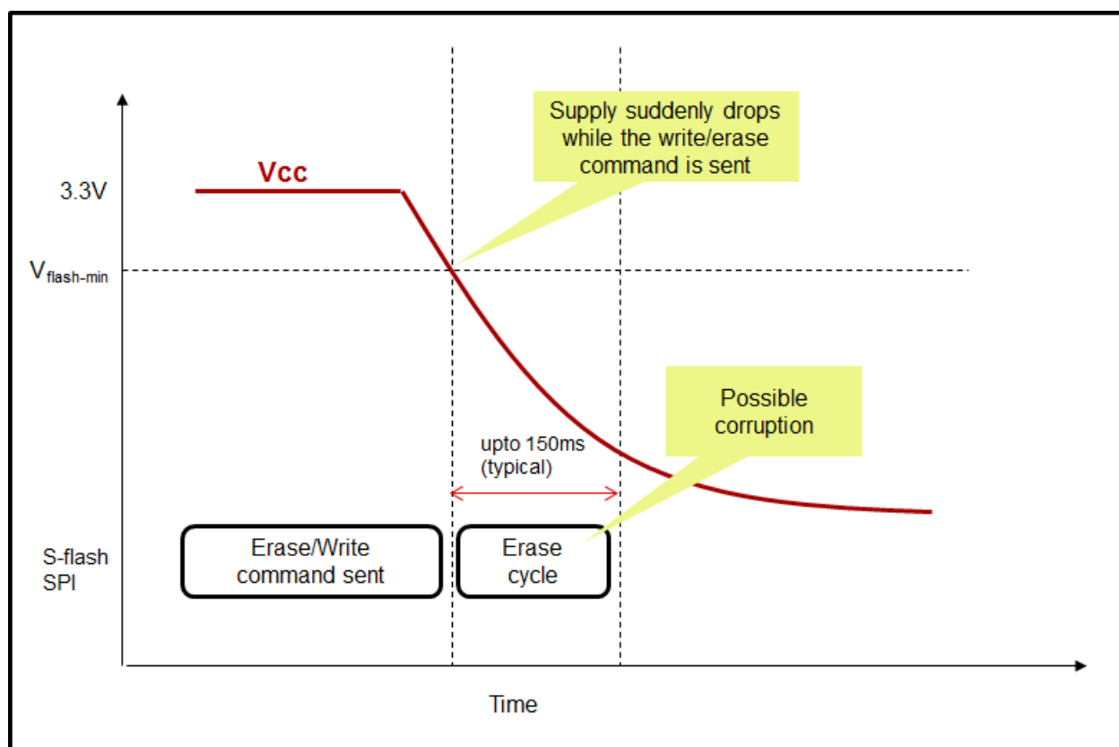
Figure 1-1. Sudden Power Off During Flash Erase
