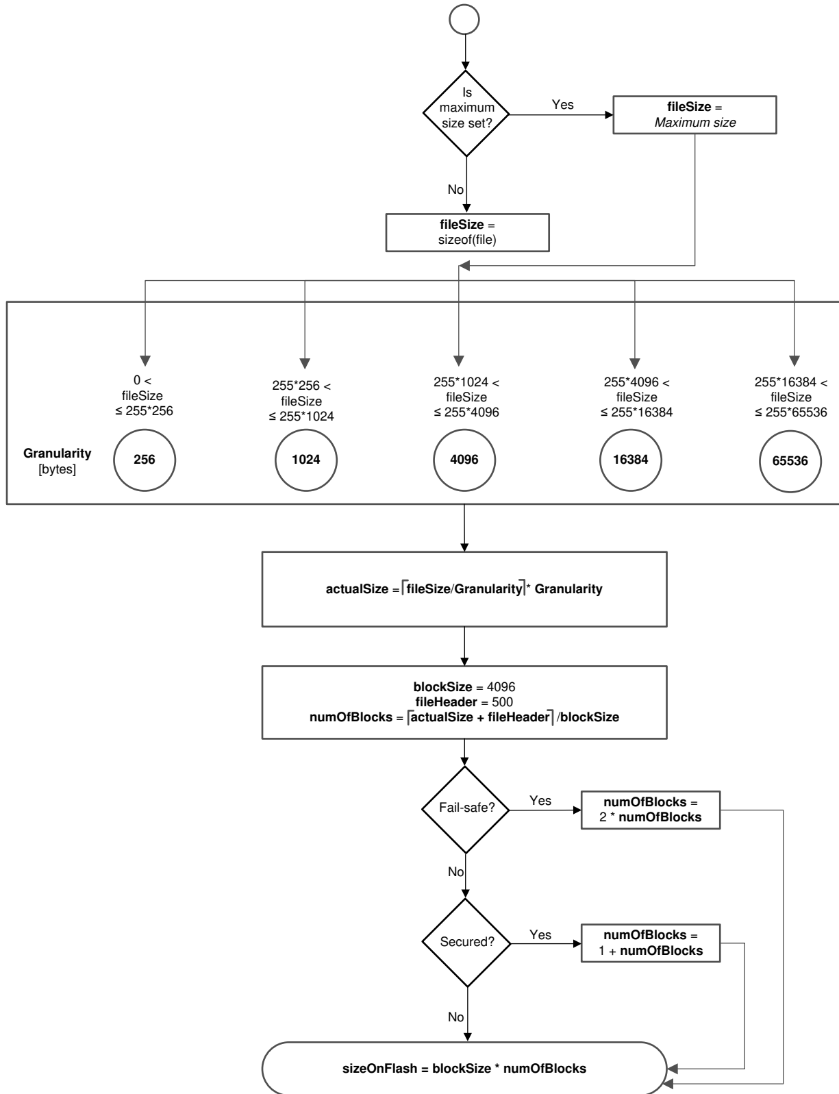
Figure 2-1. File Memory Consumption on Flash
