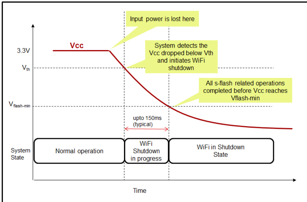
Figure 1-2. Sudden Power Off in Line-Powered Device
