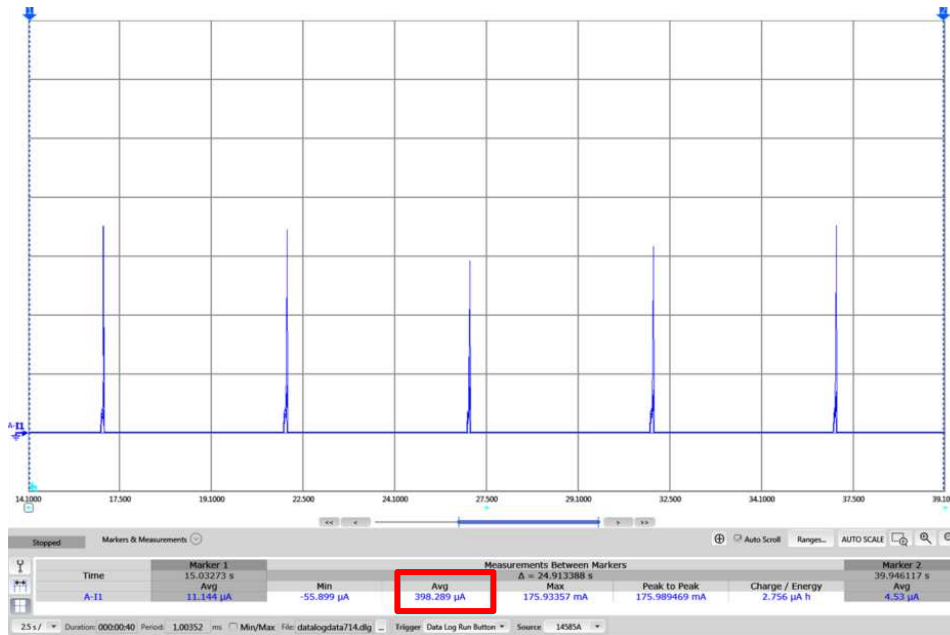
Figure 33. CC3120 Device in Transceiver Mode
