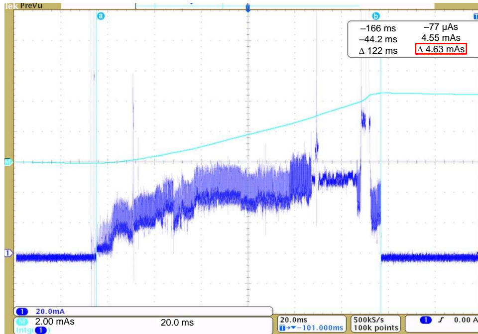
Figure 18. Current Measurement With Current Probe
