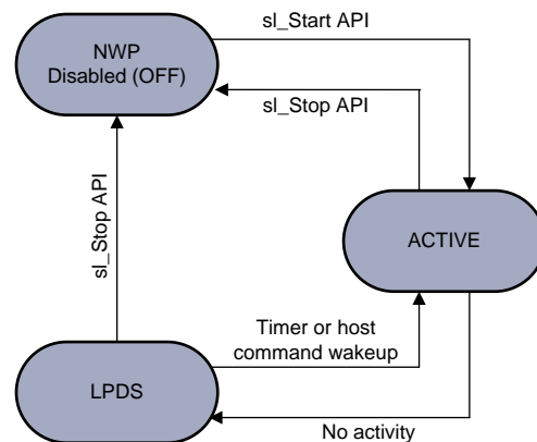
Figure 2. Transitions Between States
