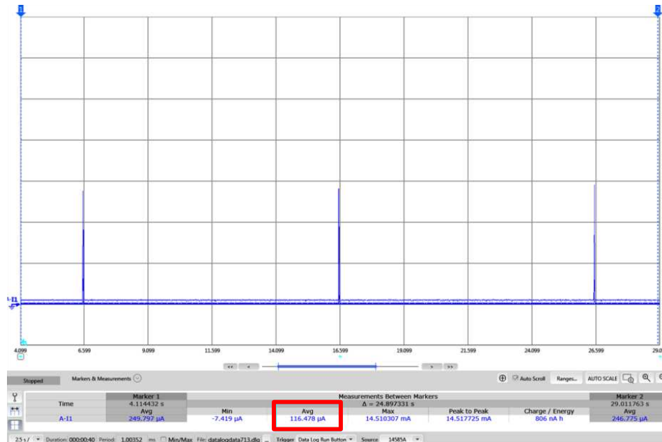
Figure 31. CC3120 Device in LPDS Mode
