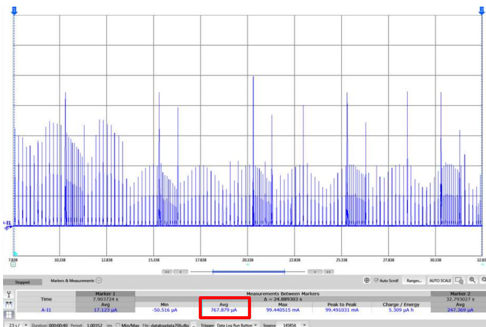
Figure 40. CC3220SF Device in Always Connected Mode (UDP)
