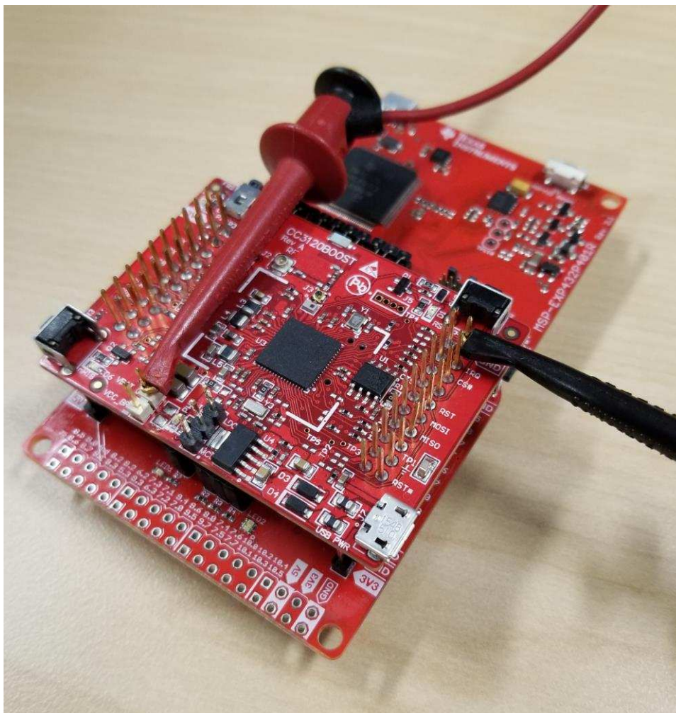
Figure 9. DC Power Analyzer Connection to CC3120 Device
