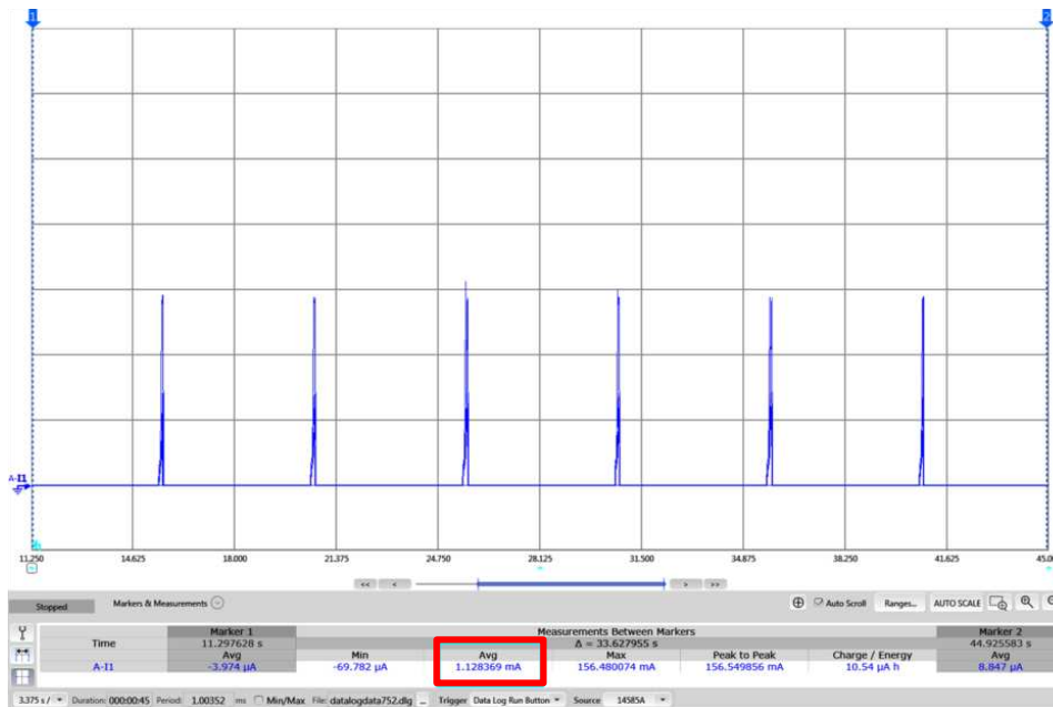
Figure 36. CC3120 Device Intermittently Connected Mode
