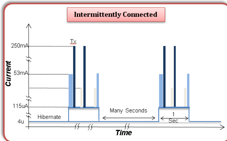
Figure 3. Intermittently Connected Test Case
