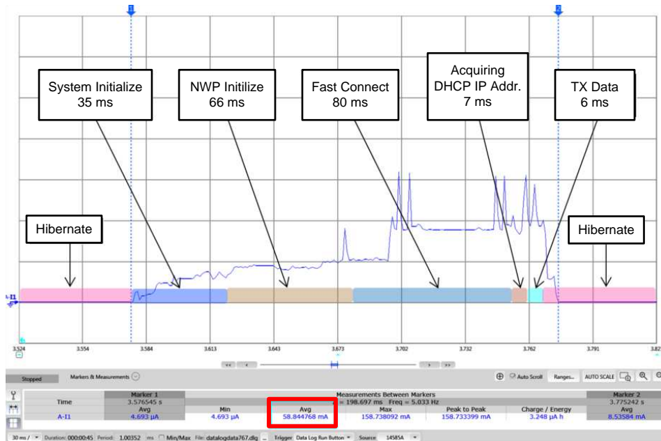
Figure 38. Intermittently Connected Mode Close-Up View
