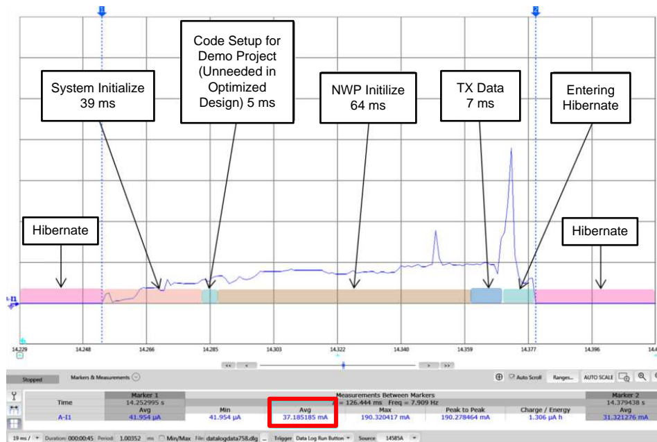
Figure 35. Transceiver Mode Close-Up View
