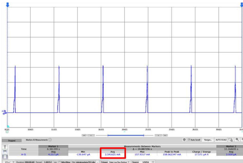
Figure 37. CC3220SF Device in Intermittently Connected Mode
