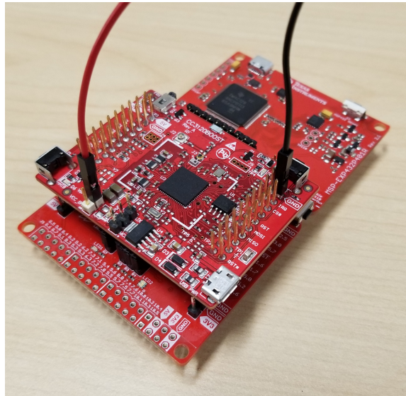
Figure 21. XDS110 ETHDR Connection to CC3120 Device
