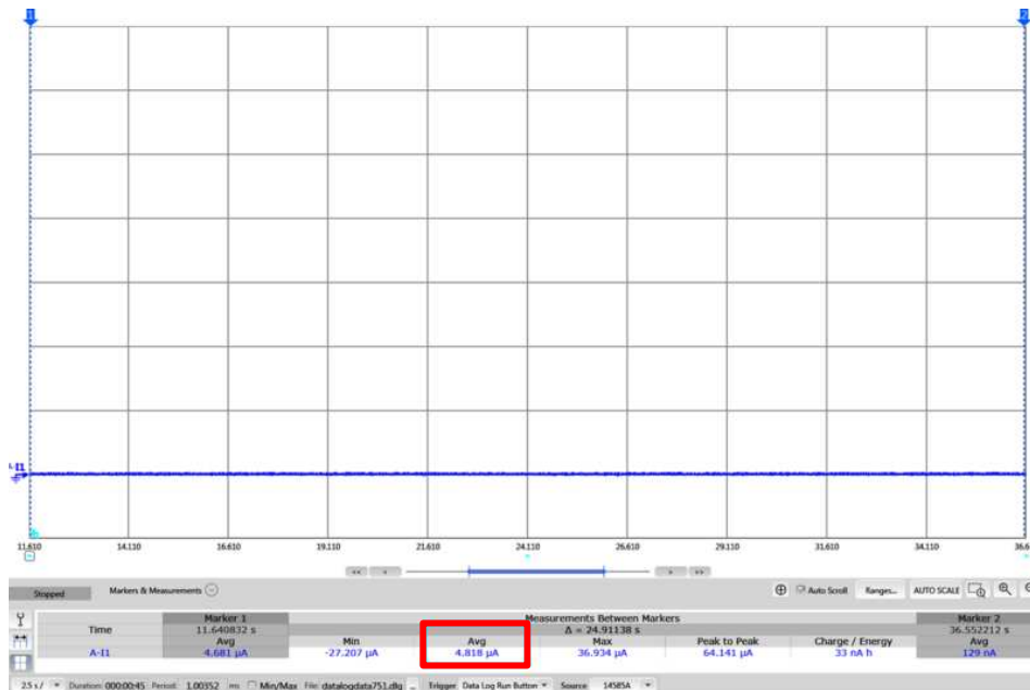
Figure 29. CC3120 Device in Hibernate Mode
