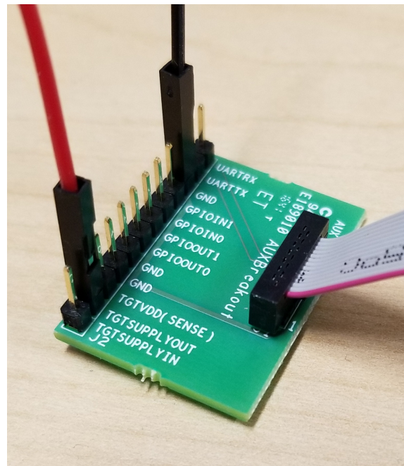
Figure 22. Breakout Board Connection
