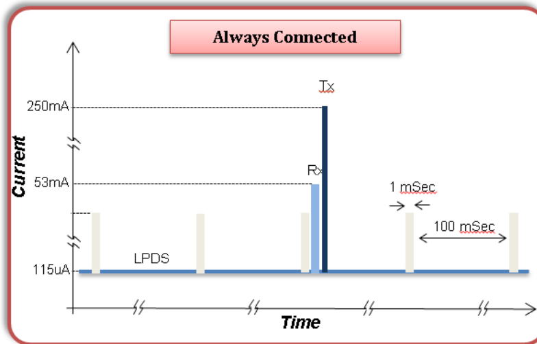
Figure 4. Always Connected Test Case
