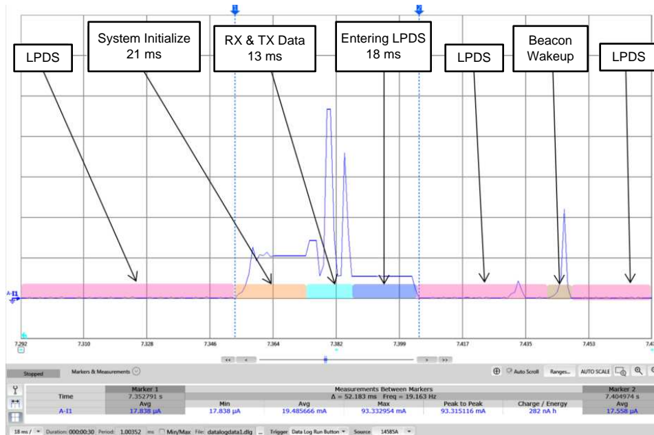
Figure 41. Always Connected Close-Up View
