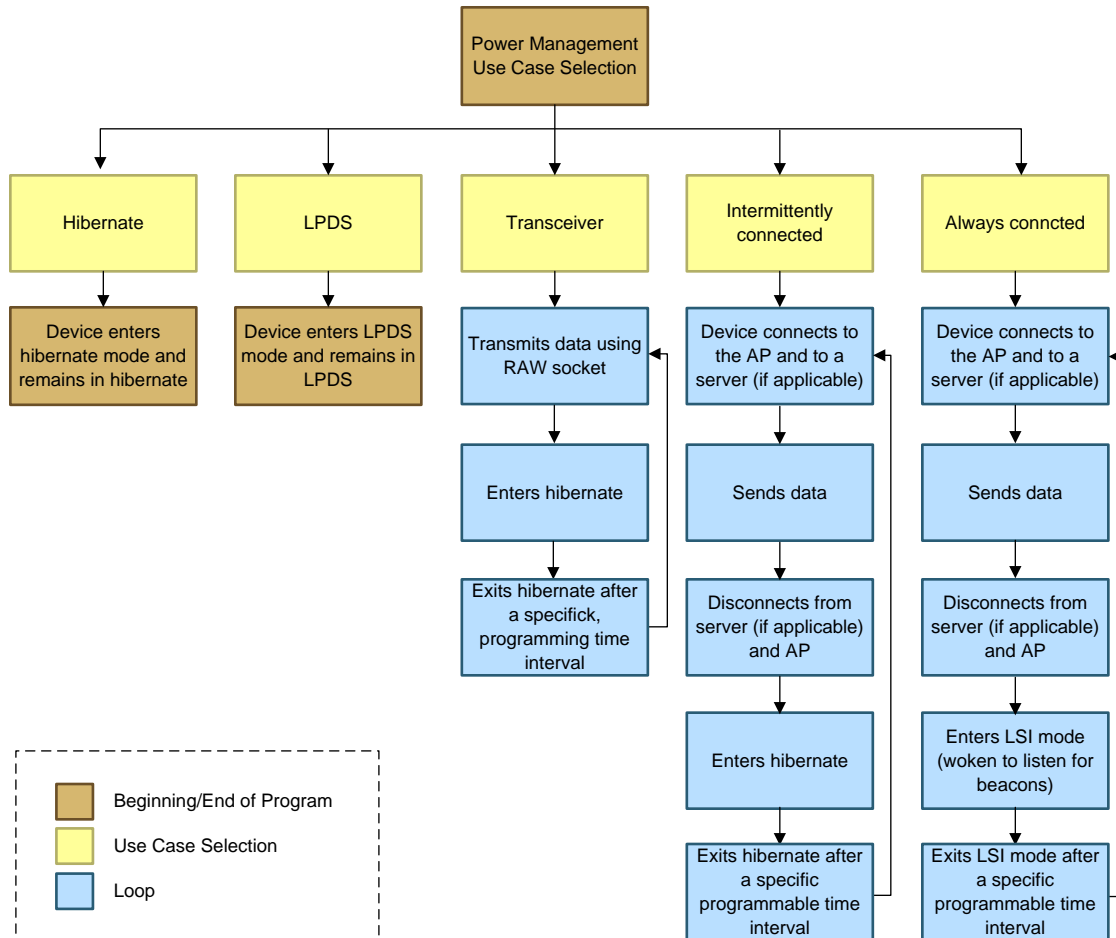
Figure 8. Power Management Use-Case Selection Flowchart
