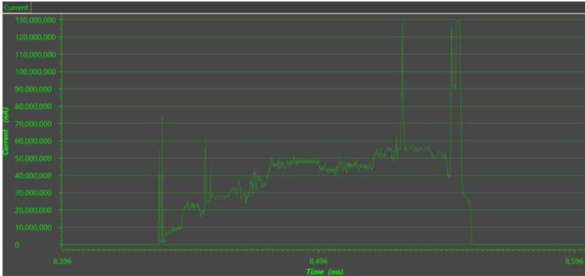
Figure 28. Average Current Measurement With EnergyTrace™
