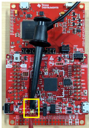
Figure 13. Current Measurement Tool Connection to CC3120 Device
