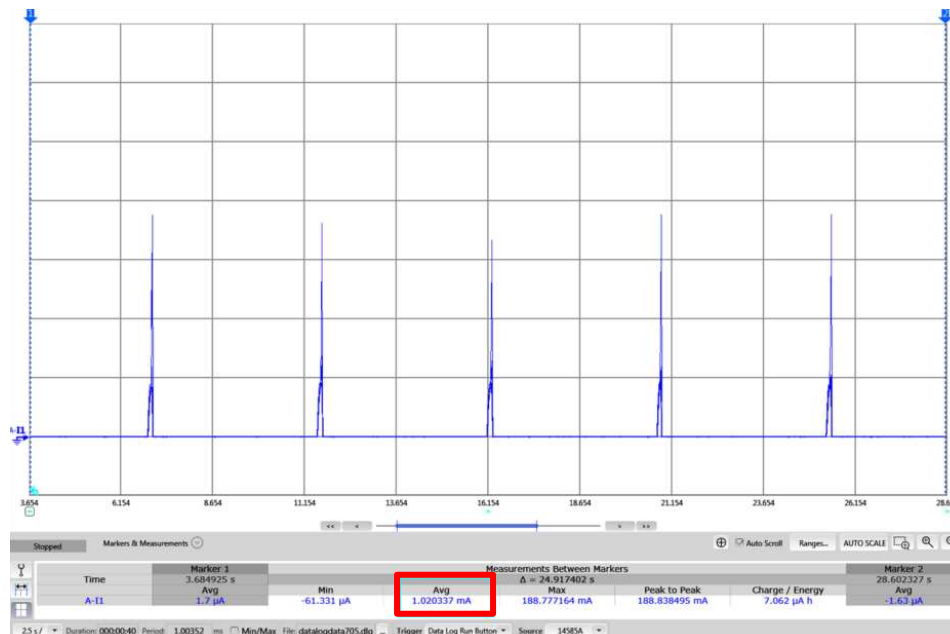
Figure 34. CC3220SF Device in Transceiver Mode
