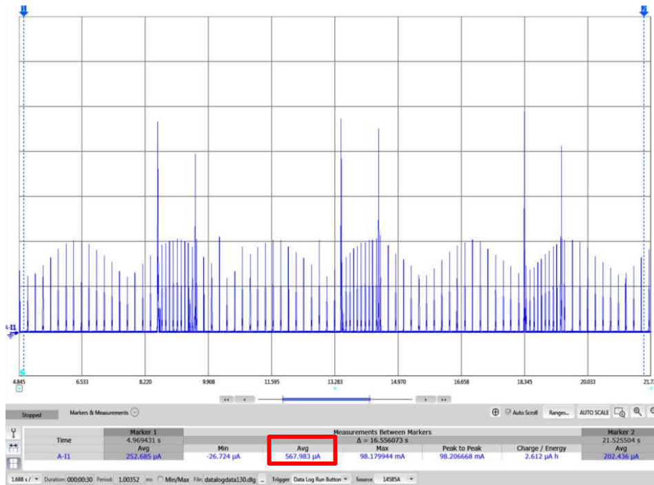
Figure 39. CC3120 Device in Always Connected Mode (UDP)
