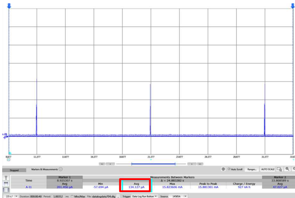
Figure 32. CC3220SF Device in LPDS Mode
