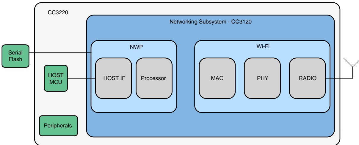
Figure 1. CC3120 and CC3220 Device Block Diagram
