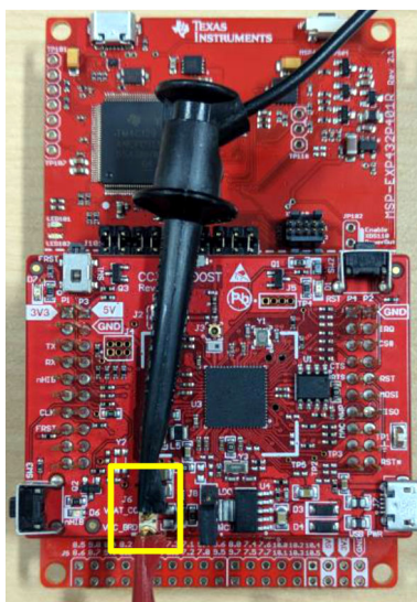
Figure 2-9. Current Measurement Tool Connection to CC3135 Device
