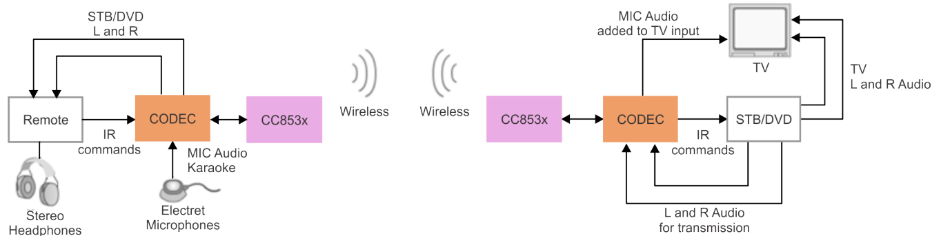
Figure 4. Demo Architecture
