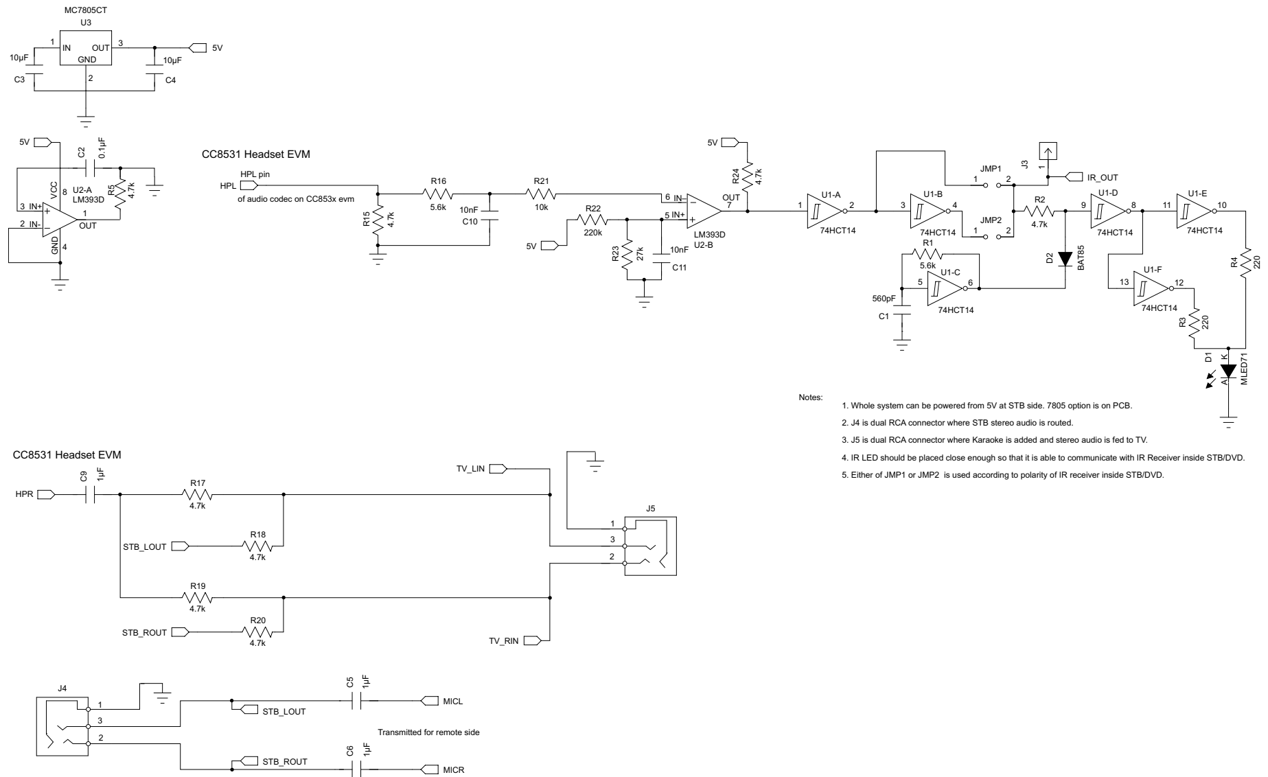
Figure 11. STB-Side Schematics
