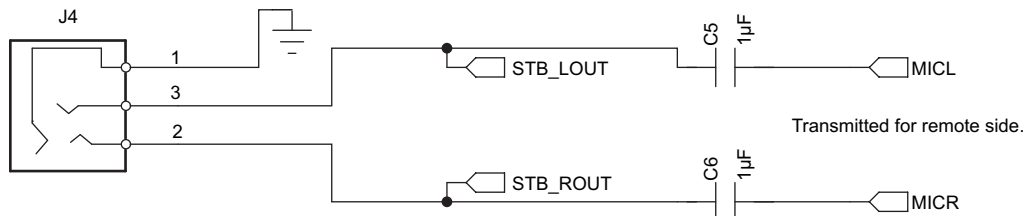
Figure 9. STB/DVD Stereo Audio Added to MIC Input for Transmission to Remote
