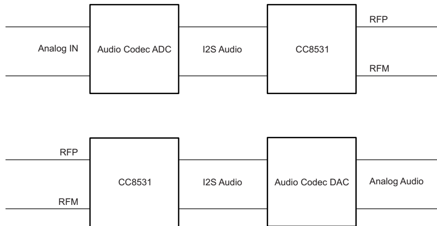
Figure 2. Audio Conversion Signal Chain
