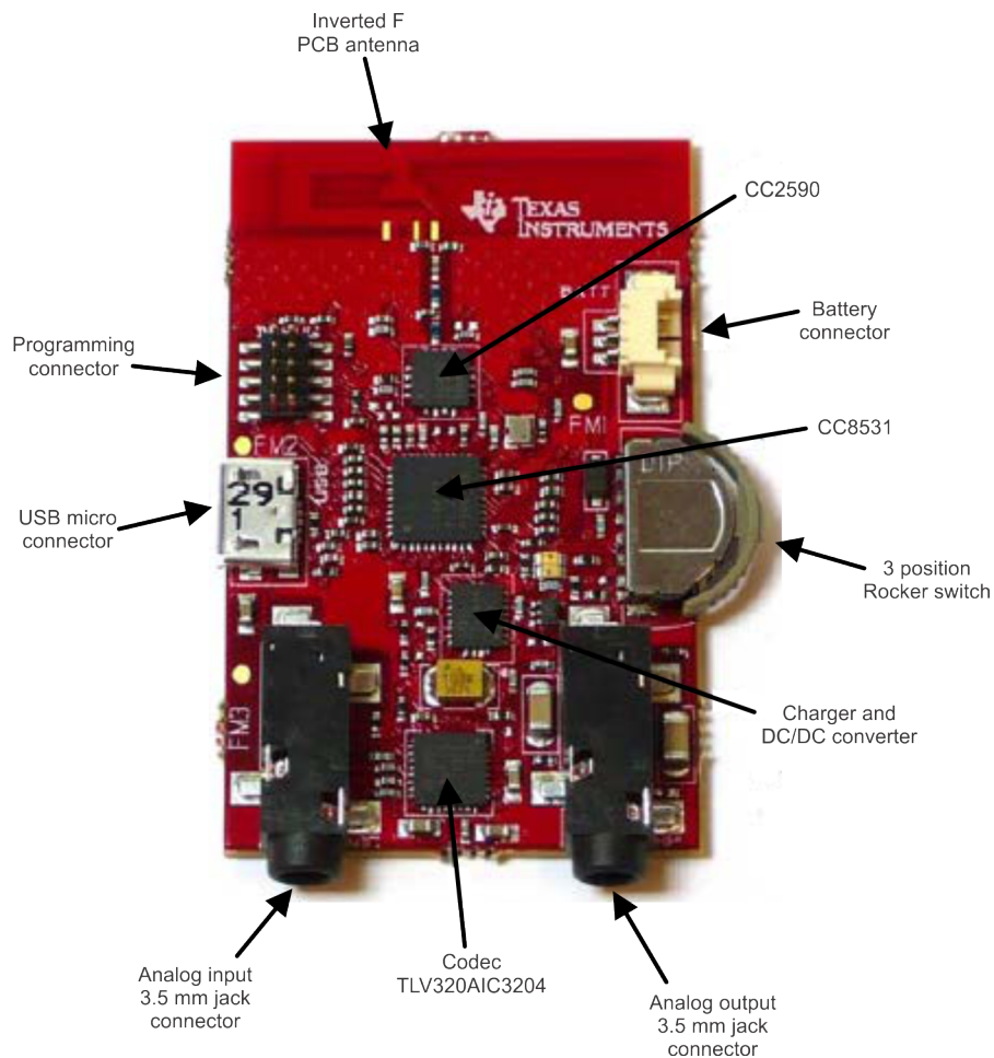
Figure 3. CC85xx Headset EVM (Master or Slave)
