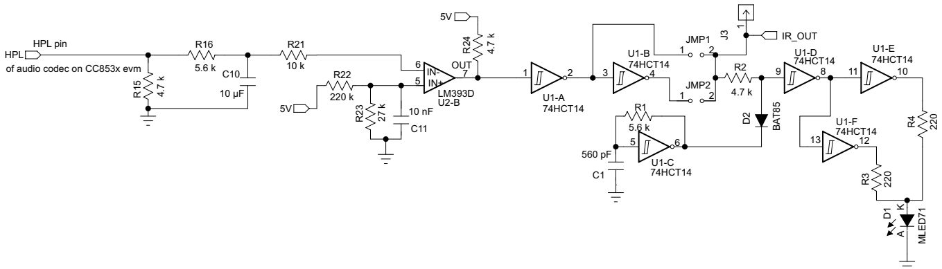
Figure 7. Processing of Received RC5 Remote Commands
