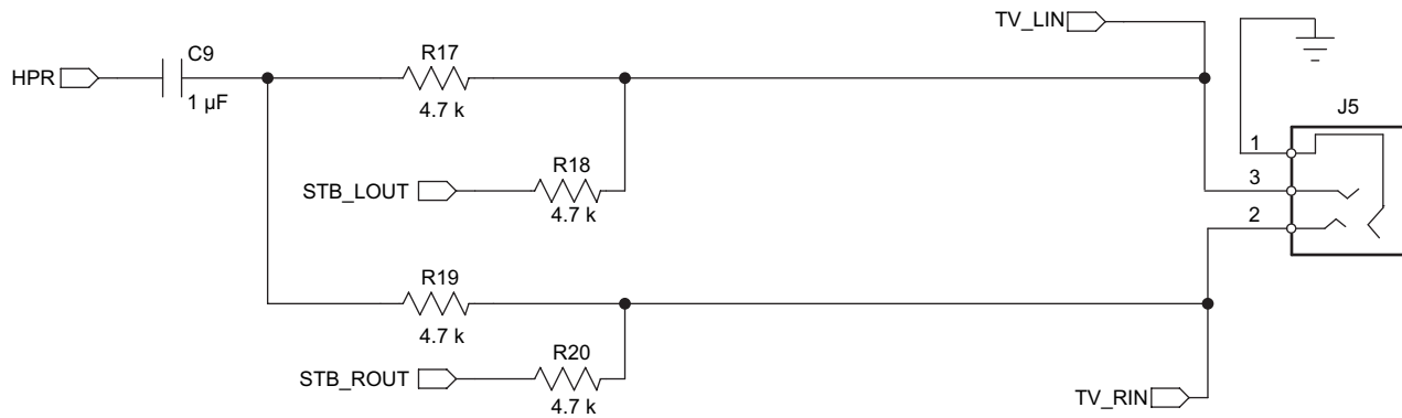
Figure 8. Add the Received Karaoke Sound to TV Audio Input
