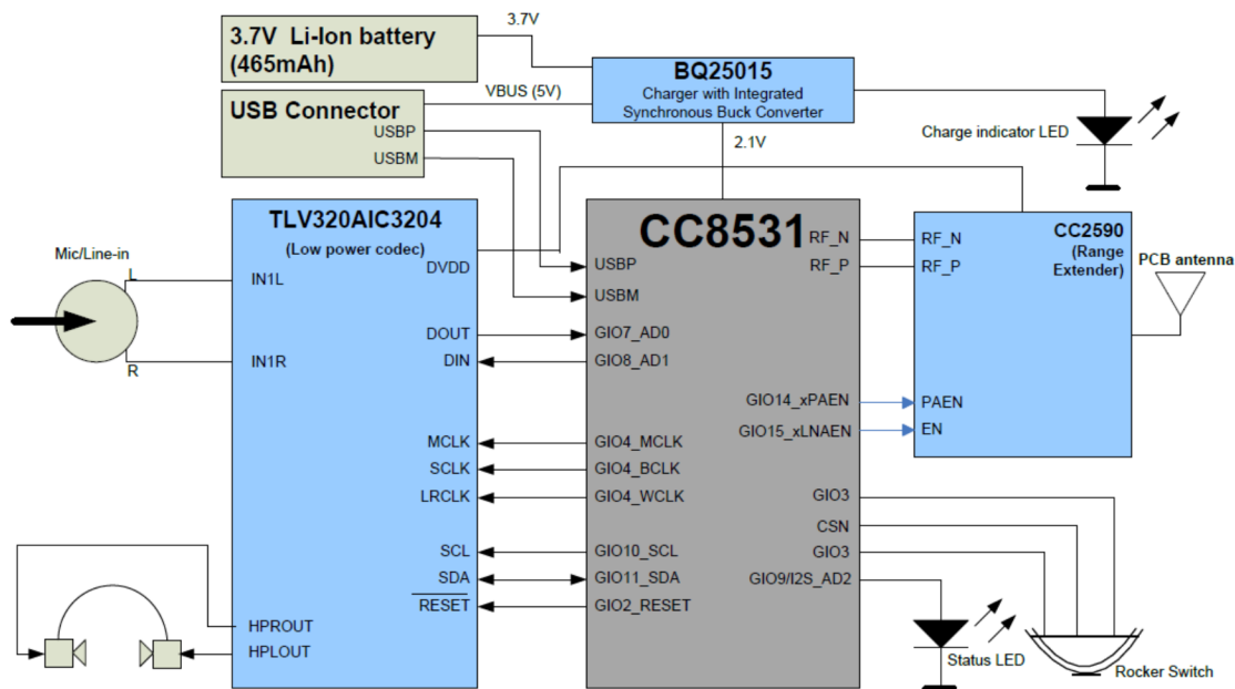
Figure 1. Typical CC85xx and TLV320AIC3204 Application Schematic
