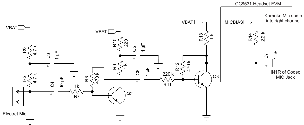
Figure 6. Karaoke MIC Audio into Right Channel
