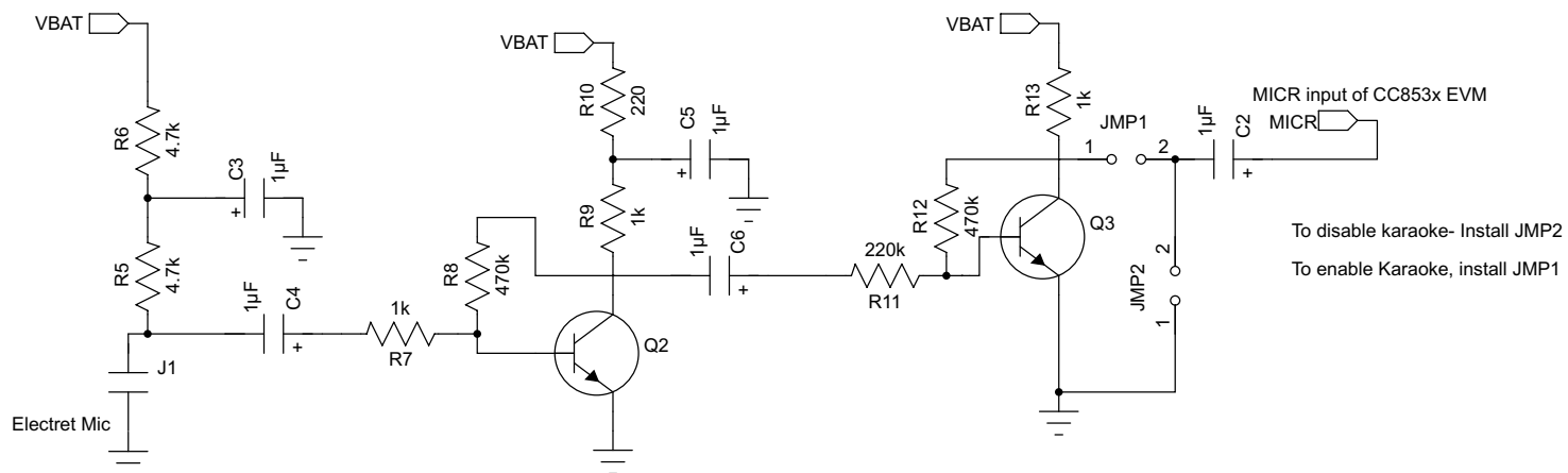
Figure 10. Remote-Side Schematics
