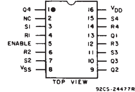
TOP VIEW 92CS-24477R1 NC = NO CONNECTION CD4044B
