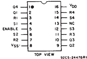
TOP VIEW 92CS-24476R1 NC = NO CONNECTION CD4043B
