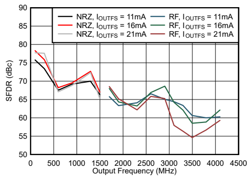
f_{CLK} = 3.2 GHz
