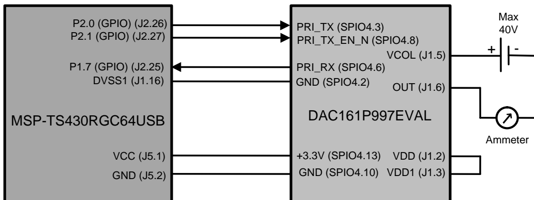
Figure 2. DAC161P997 to MSP430 Connection Diagram
