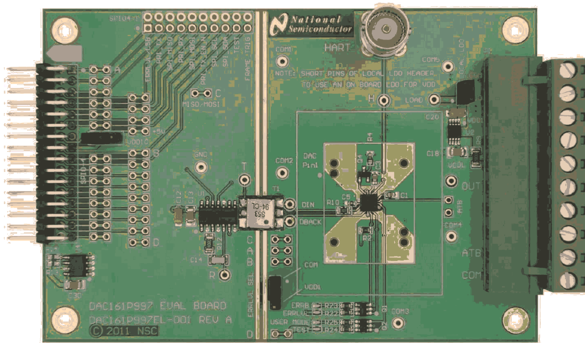
Figure 3. DAC161P997SDEVAL Jumper Settings
