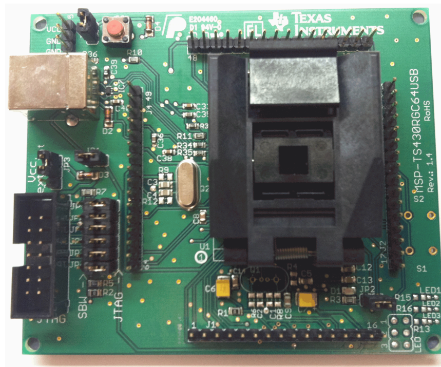
Figure 4. MSP-TS430RGC64USB Jumper Settings
