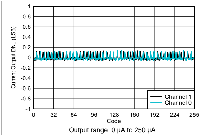
Figure 6-36. Current Output DNL vs Digital Input Code
