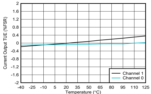
Figure 6-37. Current Output TUE vs Temperature
