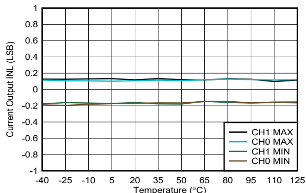
Figure 6-31. Current Output INL vs Temperature
