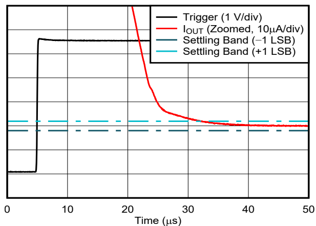
Figure 6-43. Current Output Setting Time, Falling Edge
