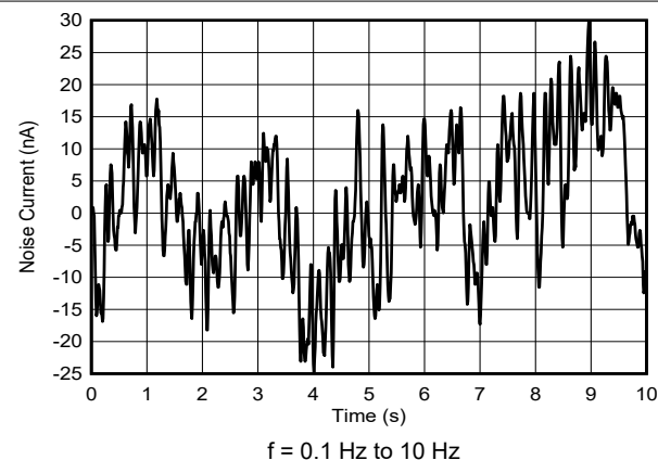
Figure 6-47. Current Output Flicker Noise
