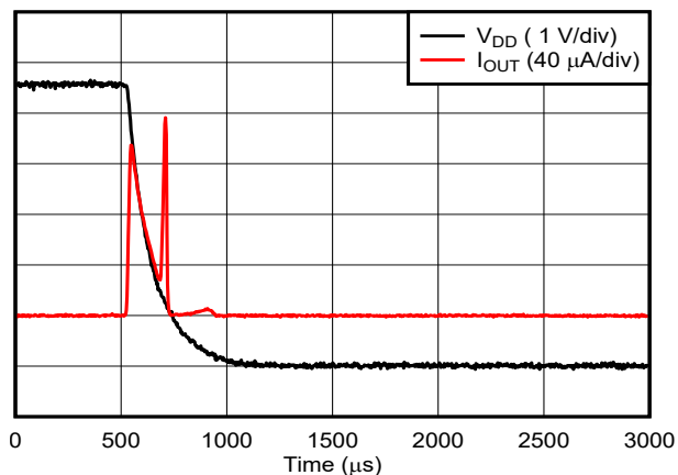
Figure 6-43. Current Output Setting Time, Falling Edge
