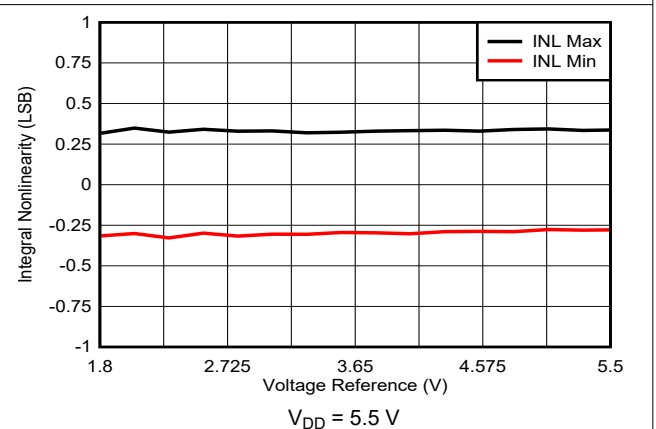
Figure 7-7. Integral Nonlinearity vs Voltage Reference
