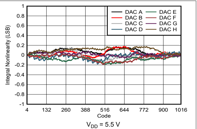
Figure 7-3. Integral Nonlinearity vs Digital Input Code
