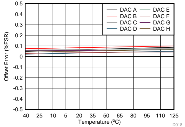
Figure 19. Offset Error vs Temperature
