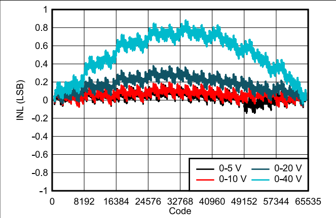
Figure 7-4. DAC81404 INL vs Digital Input Code (Unipolar Outputs)
