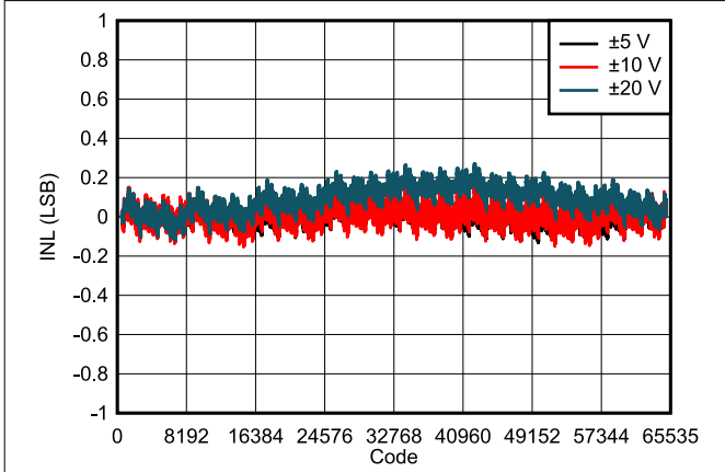
Figure 7-3. DAC81404 INL vs Digital Input Code (Bipolar Outputs)
