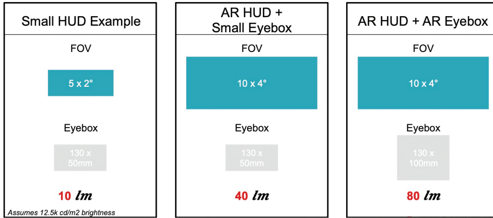
Figure 6. As the FOV and eyebox increase, more light is required
