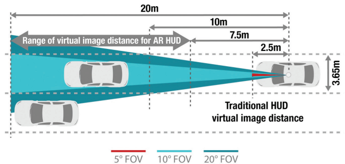
Figure 3. AR HUDs have a VID of up to 20 m, while traditional HUDs have a much shorter VID
