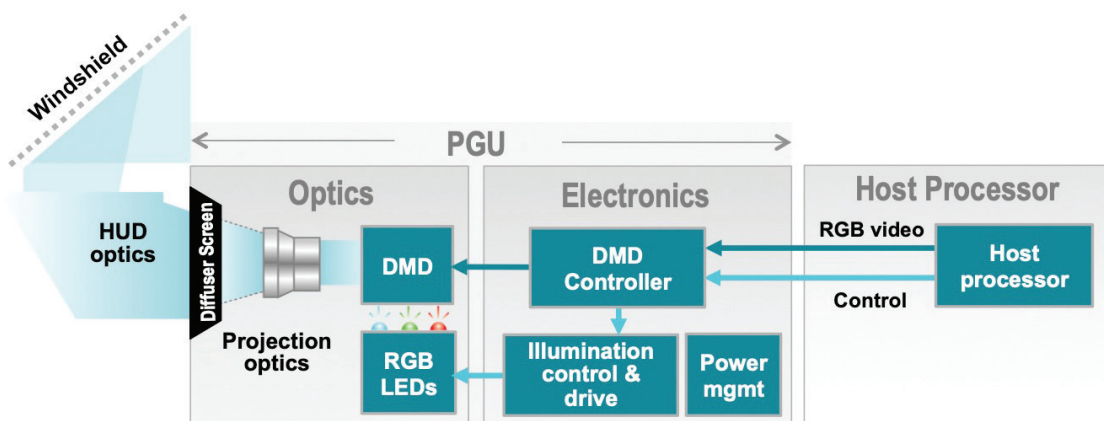
Figure 9. A DLP Auto PGU with diffuser screen
