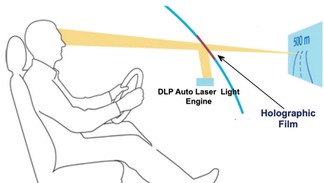
Figure 17. Holographic film based AR HUD
