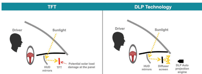
Figure 7. Comparison of a TFT-based HUD vs. a DLP technology-based HUD
