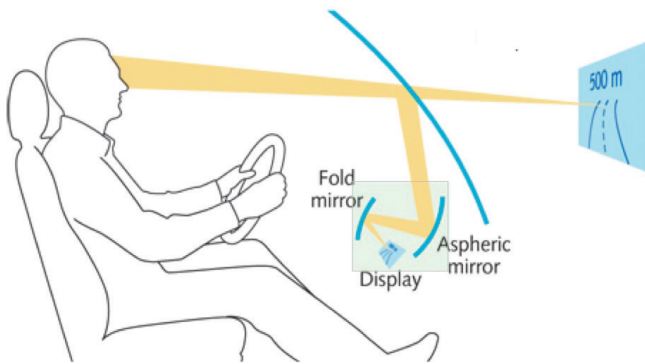
Figure 15. Traditional optics based HUD with large aspheric mirror
