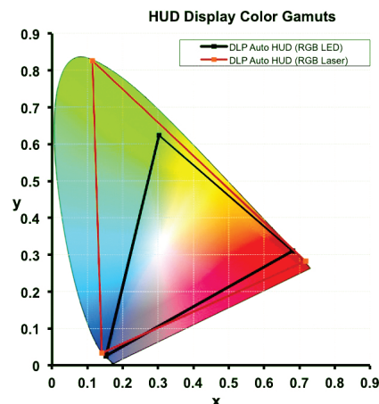
Figure 14. HUD laser vs LED color gamuts when using DLP technology
