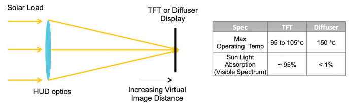
Figure 8. The longer the VID, the more concentrated the solar load
