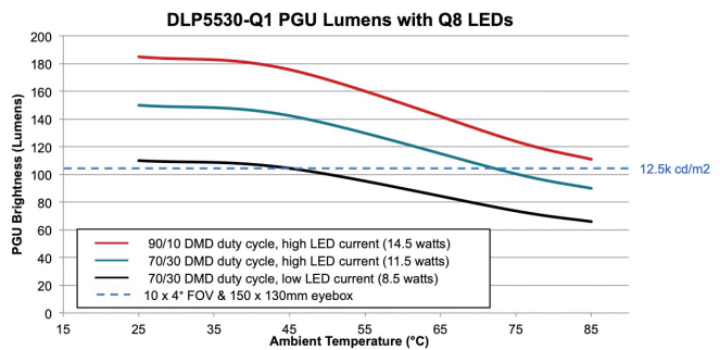
Figure 11. PGU brightness as a function of temperature, DMD duty cycle and LED current
