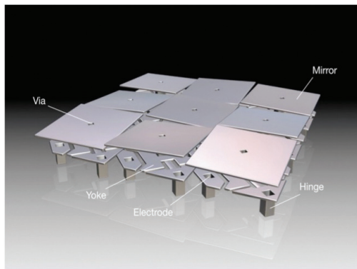
Figure 10. Example of a DMD micromirror array
