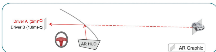
Figure 5. A larger eyebox supports both Driver A and Driver B
