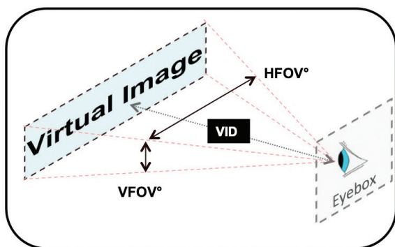
Figure 1. FOV and VID in a HUD
