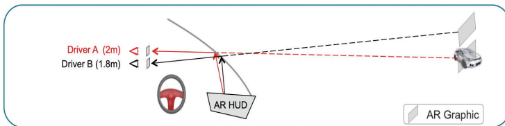
Figure 4. In an AR HUD, adjusting the eyebox height loses graphic alignment for Driver B
