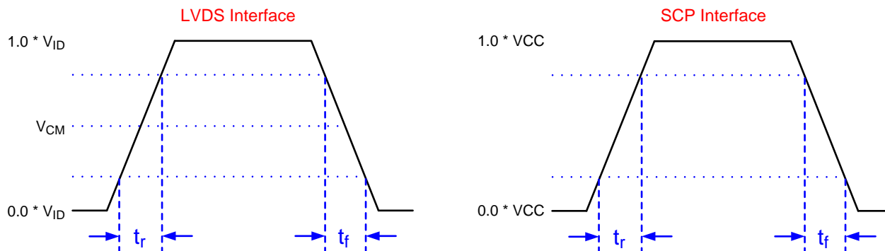
Figure 2. SCP Timing Parameters
