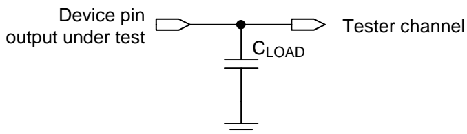
Figure 4. Test Load Circuit for Output Propagation Measurement
