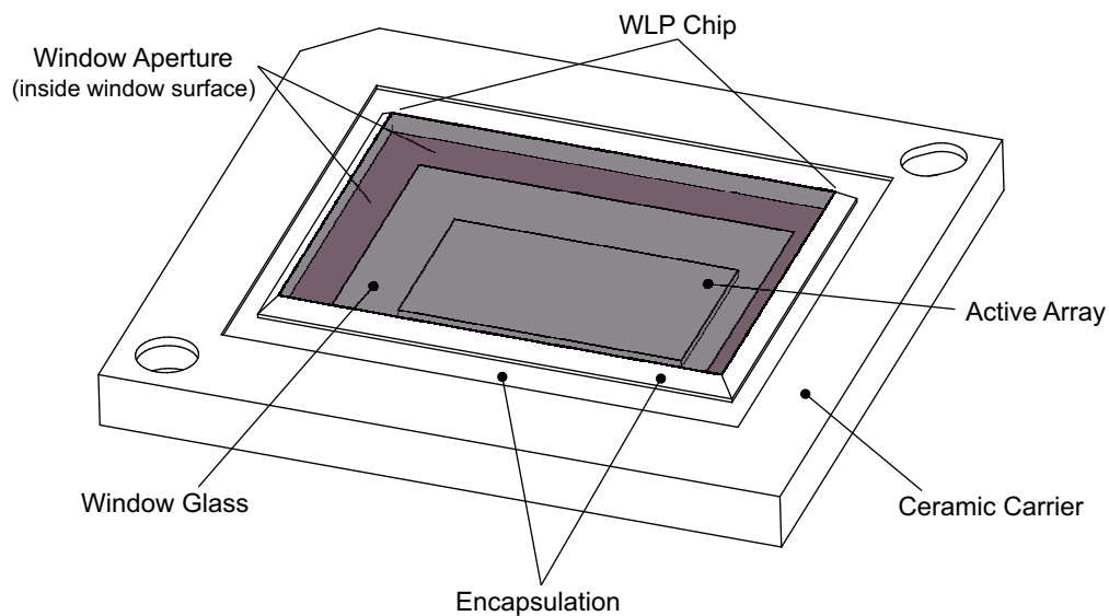
Figure 1. Series-600 DMD Features – Window Side
