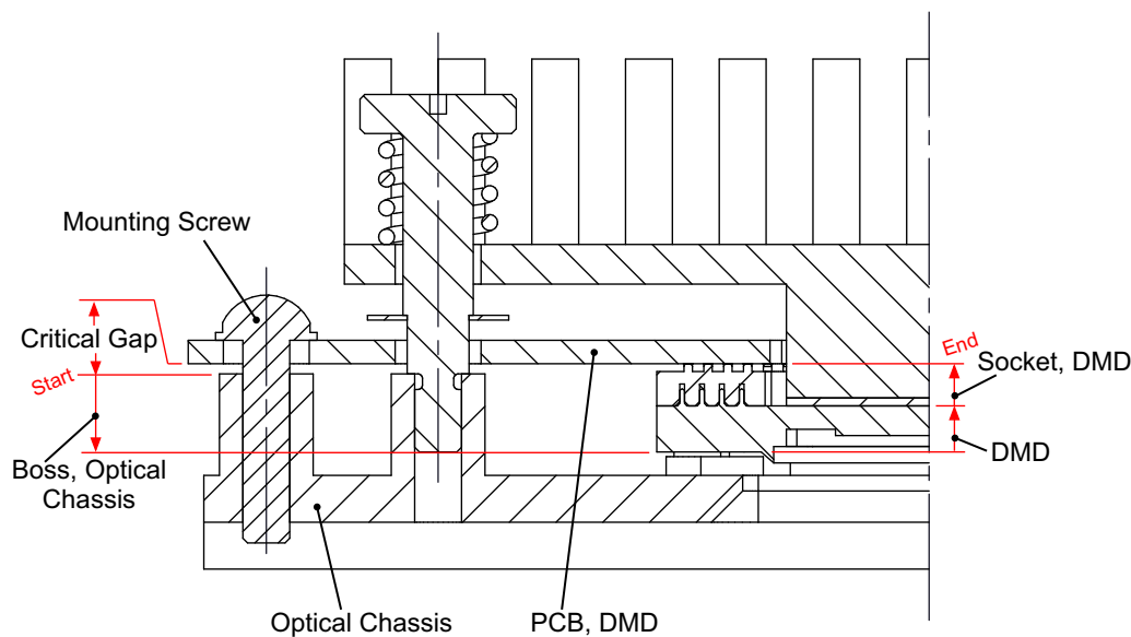
Figure 19. DMD-PCB Gap Analysis Schematic Diagram
