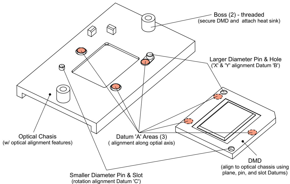
Figure 12. Optical Interface (Alignment) Features
