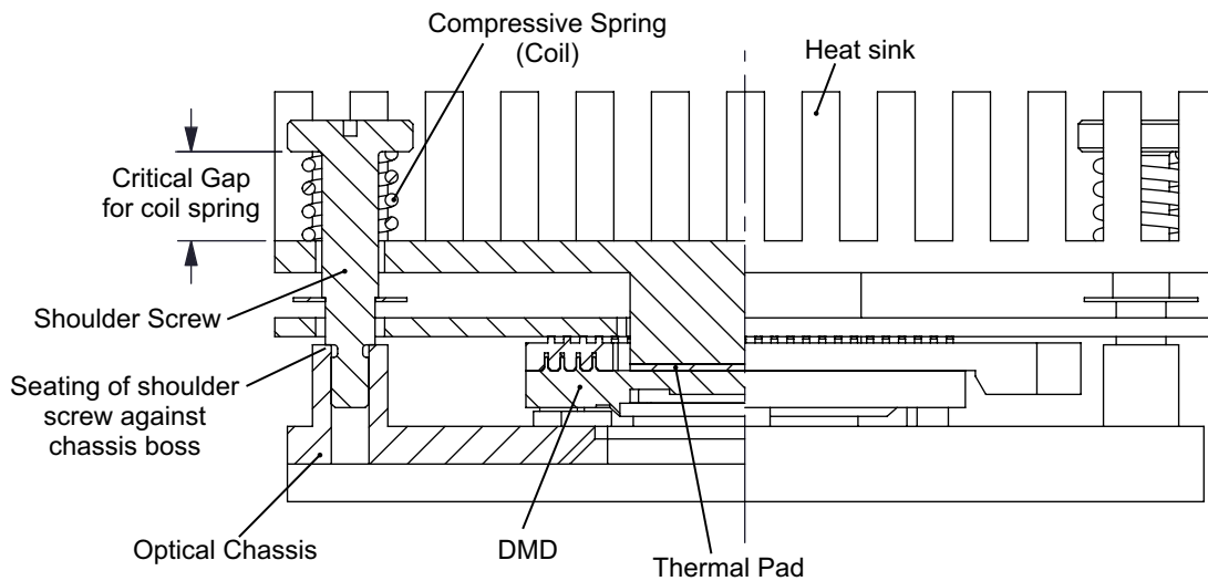
Figure 13. Heat Sink Mounting – Load Control by Design
