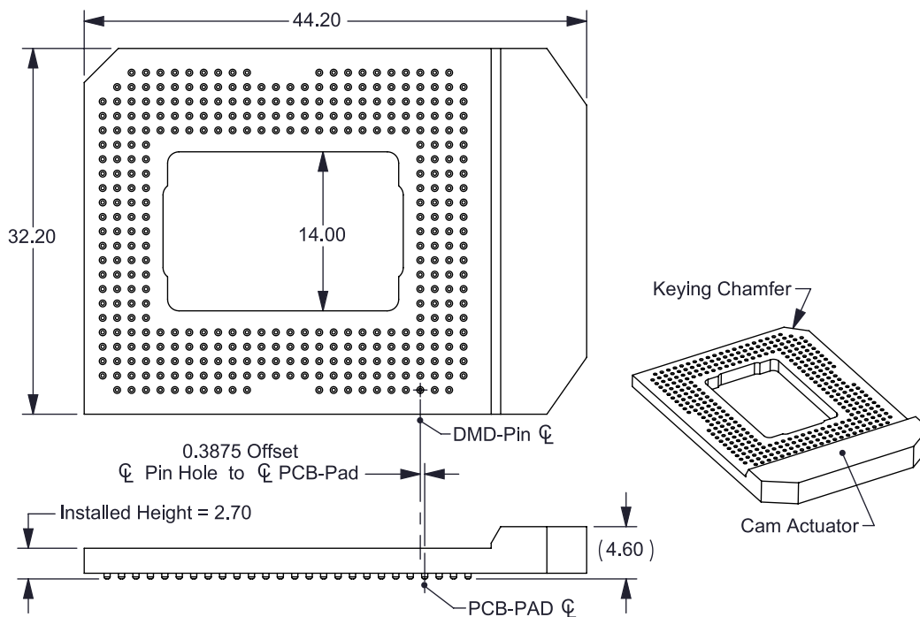
Figure 21. Zero Insertion Force Style Series-600 Socket
