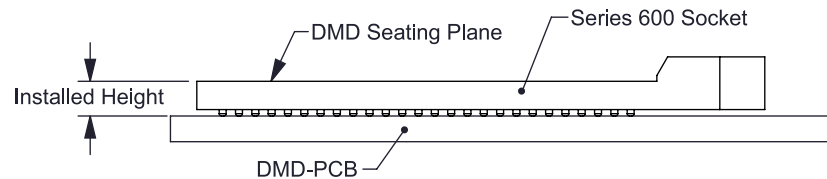
Figure 20. Socket Installed Height
