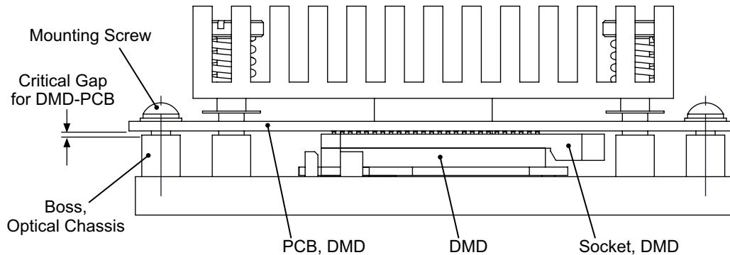
Figure 15. DMD-PCB Mounting Gap - Indirect Control of Load on DMD
