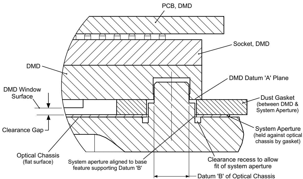
Figure 16. System Aperture and Dust Gasket
