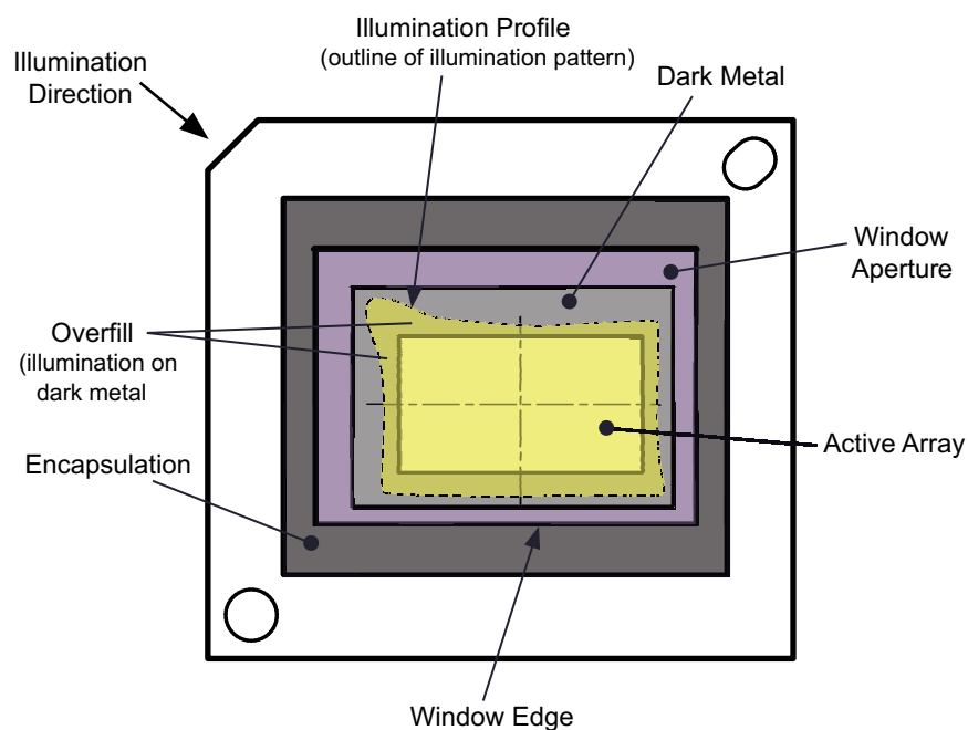
Figure 5. Optical Illumination Overfill
