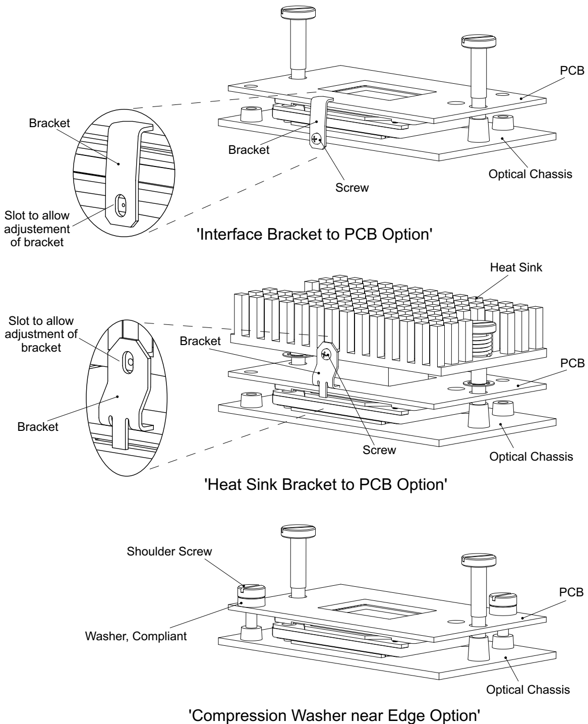
Figure 14. Direct Control of DMD-PCB Mounting Options
