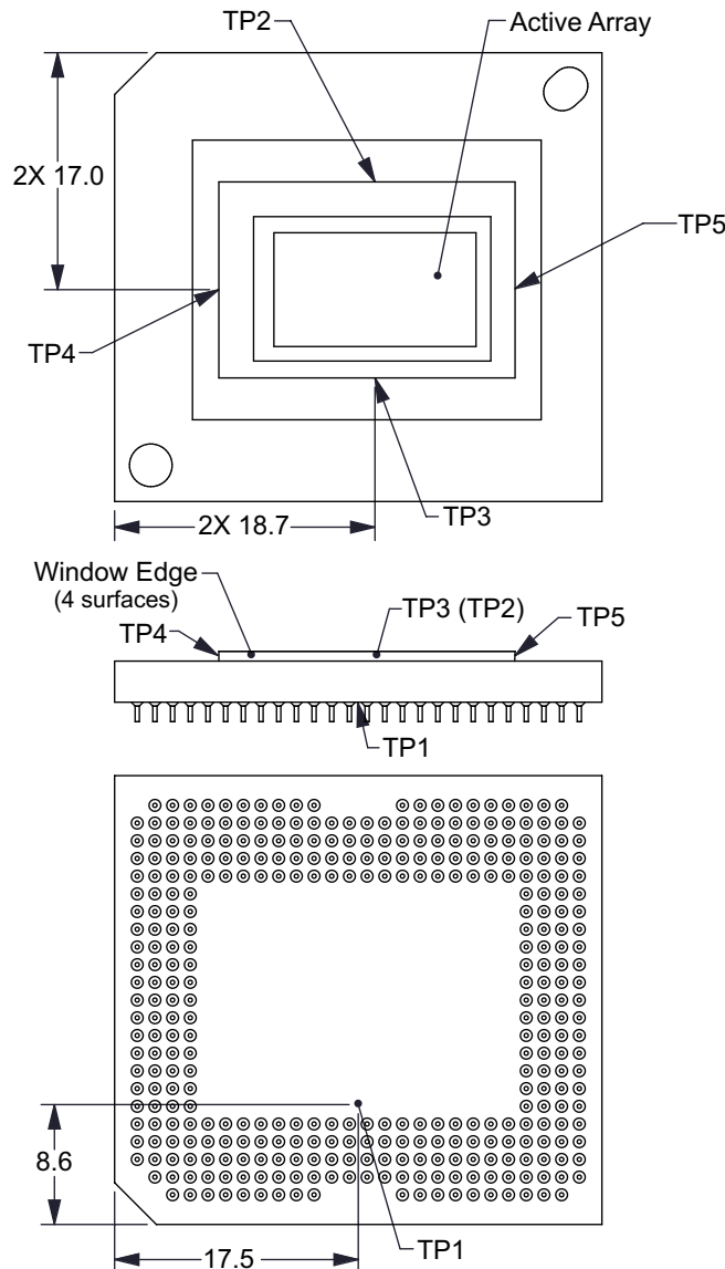
Figure 9. Thermal Test Points – Standard Locations
