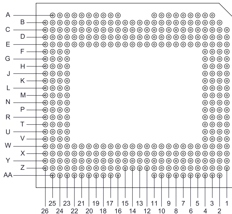
Figure 7. Pin Numbering Scheme
