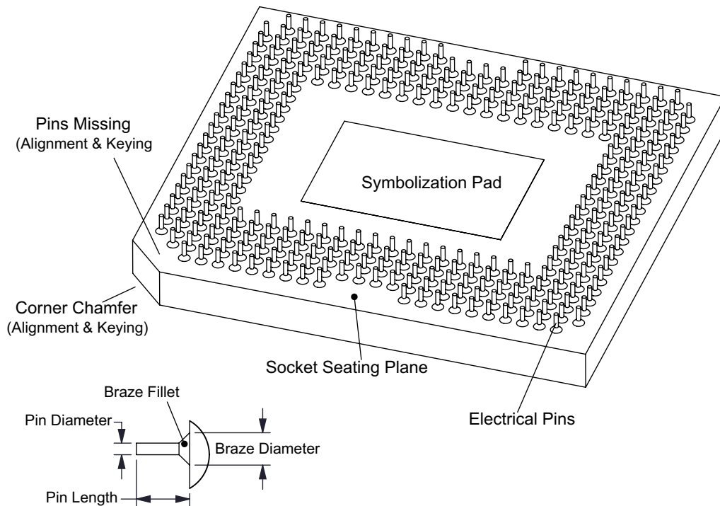
Figure 8. Electrical and Thermal Interface
