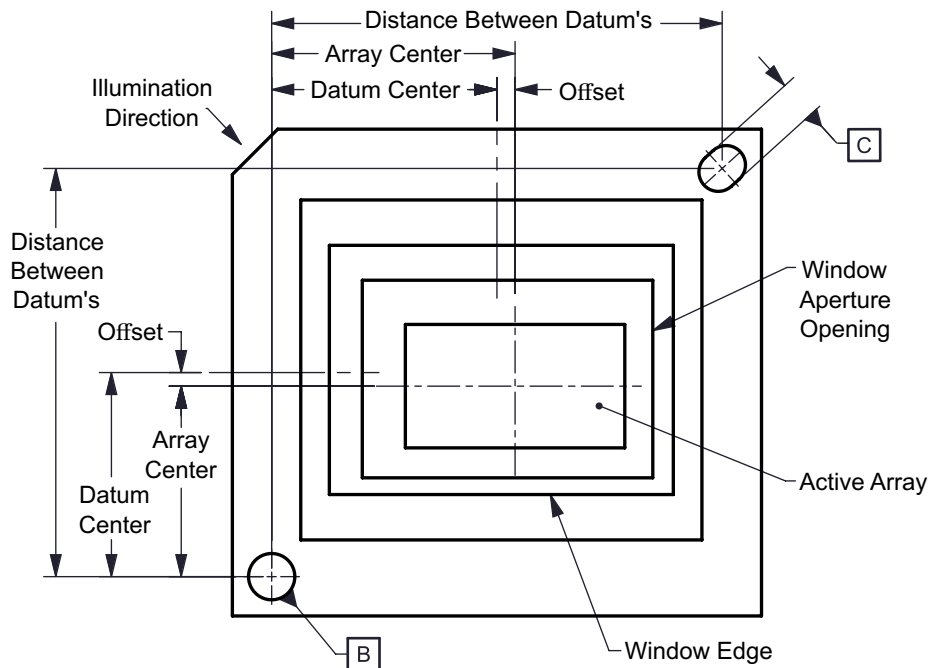
Figure 6. Active Array Location
