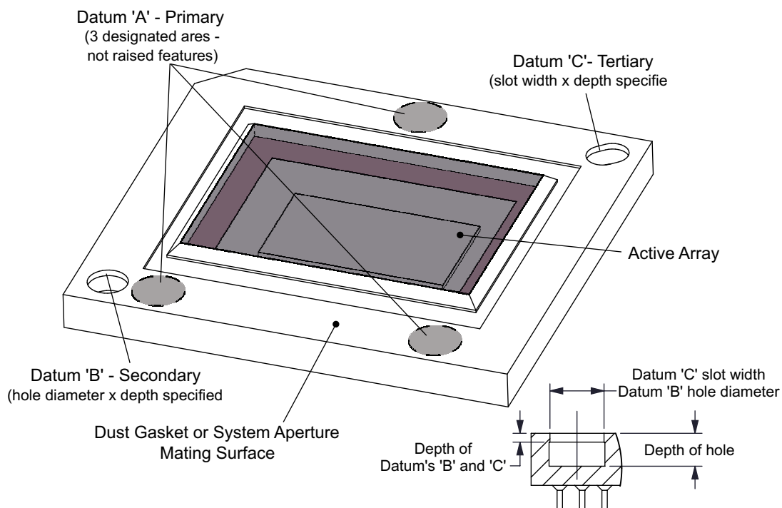
Figure 3. Series-600 DMD Datum Features
