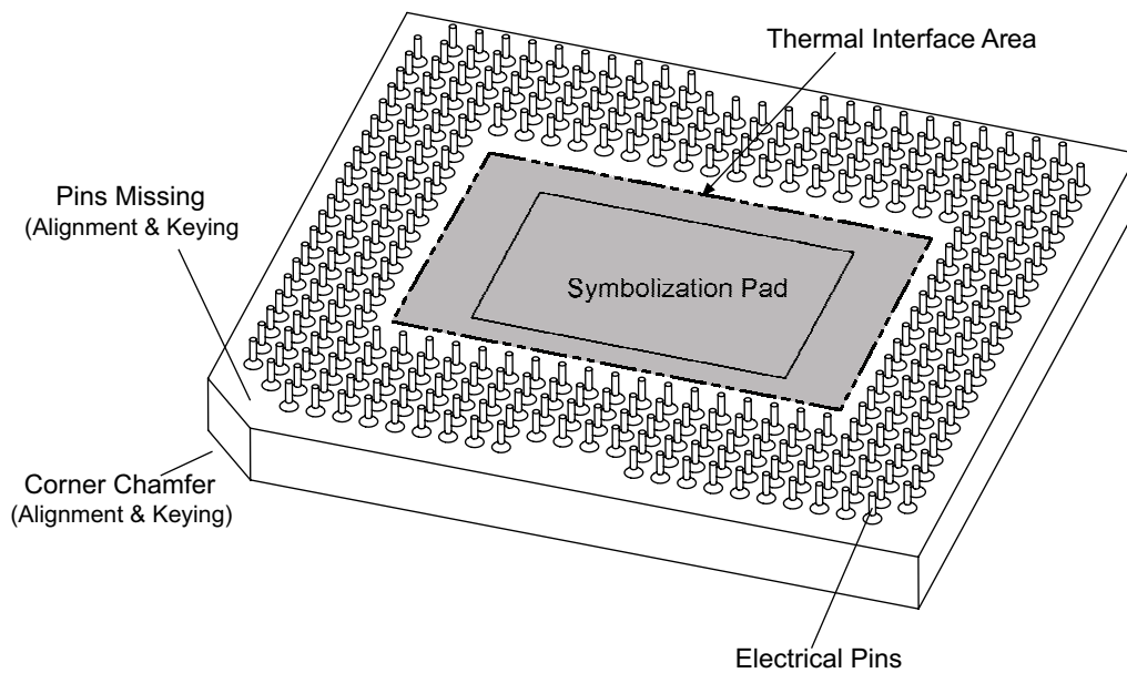
Figure 2. Series-600 DMD Features – Pin Side
