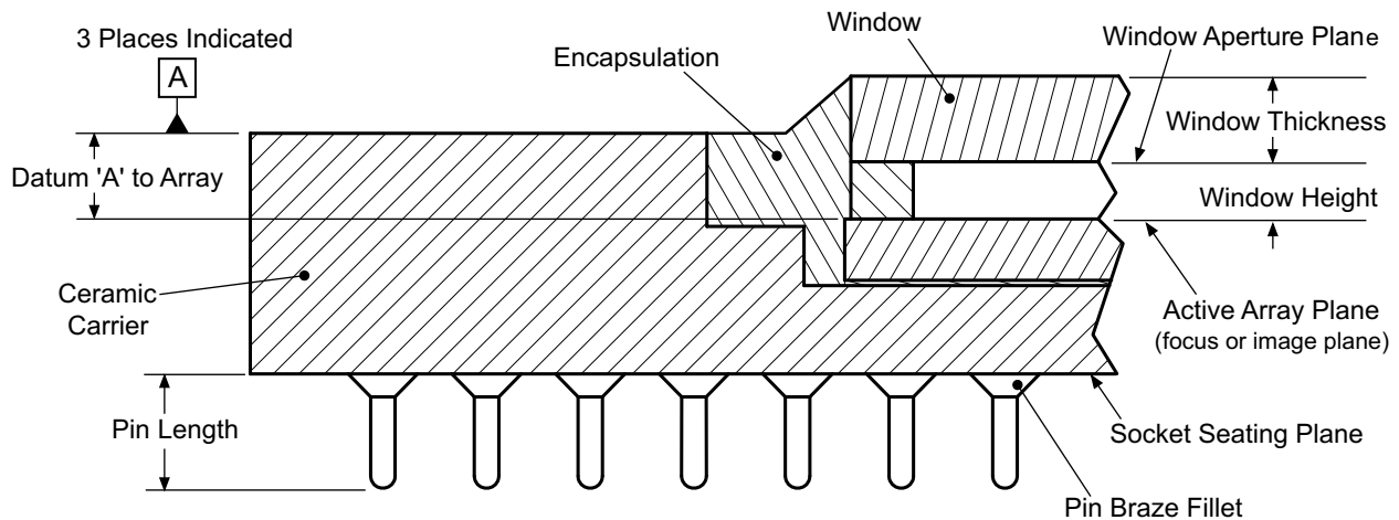
Figure 4. Series-600 DMD Cross Section View
