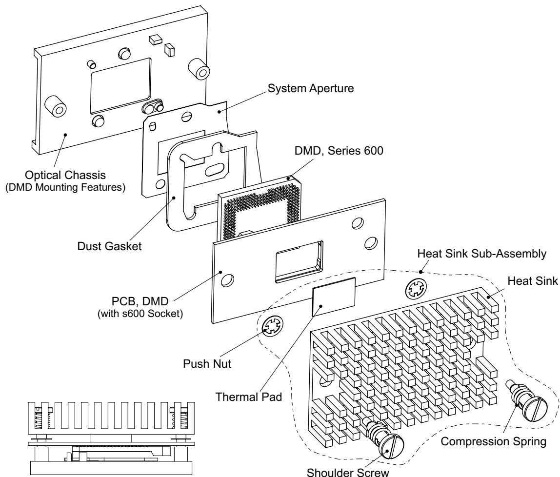
Figure 11. Basic DMD Mechanical Mounting Concept
