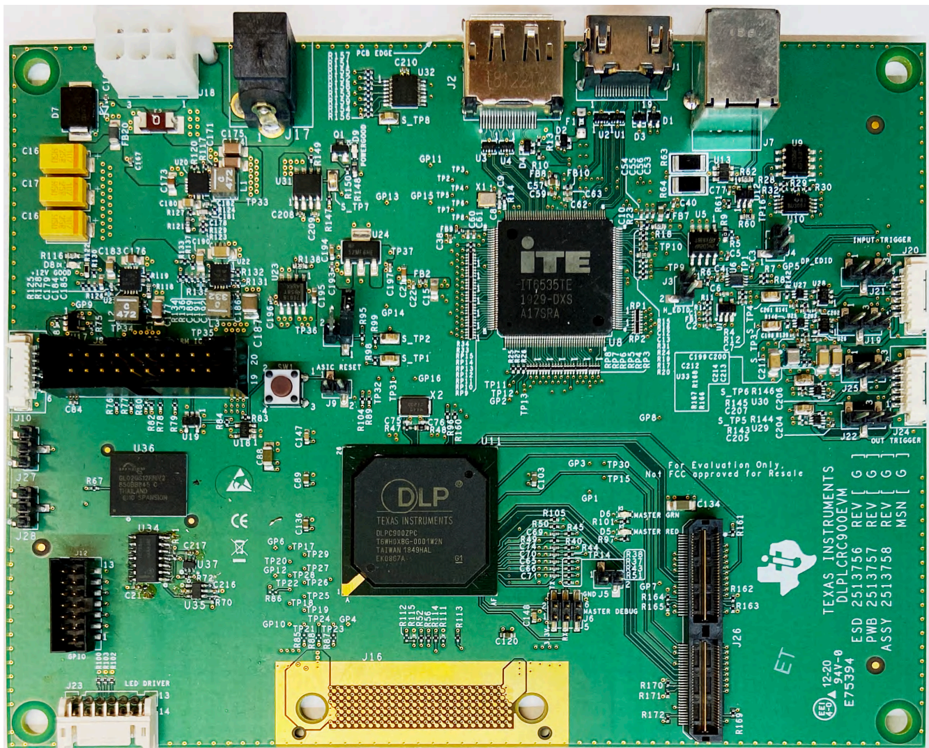
Figure 1-1. DLP LightCrafter Single DLPC900 Evaluation Module
