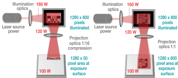
Figure 9: Optical compression as a means to attenuate power per pixel including a QR code (a) and a grayscale image (b).
