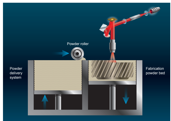
Figure 1: SLS 3D printing process.
