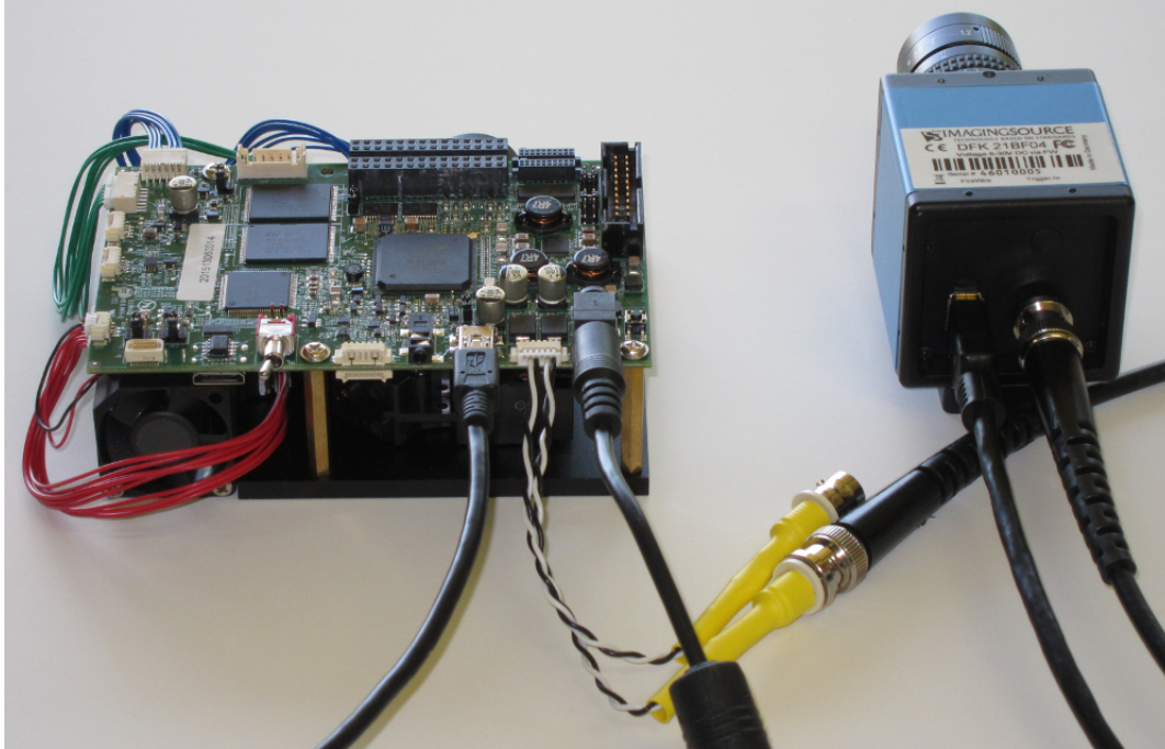
Figure 6. Example Setup of DLP LightCrafter 4500 and Firewire Camera from The Imaging Source
