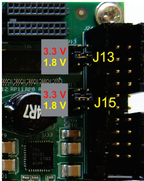
Figure 4. Jumper Locations for Setting Voltage Levels on J13 (Trigger Out 1) and J15 (Trigger Out 2)
