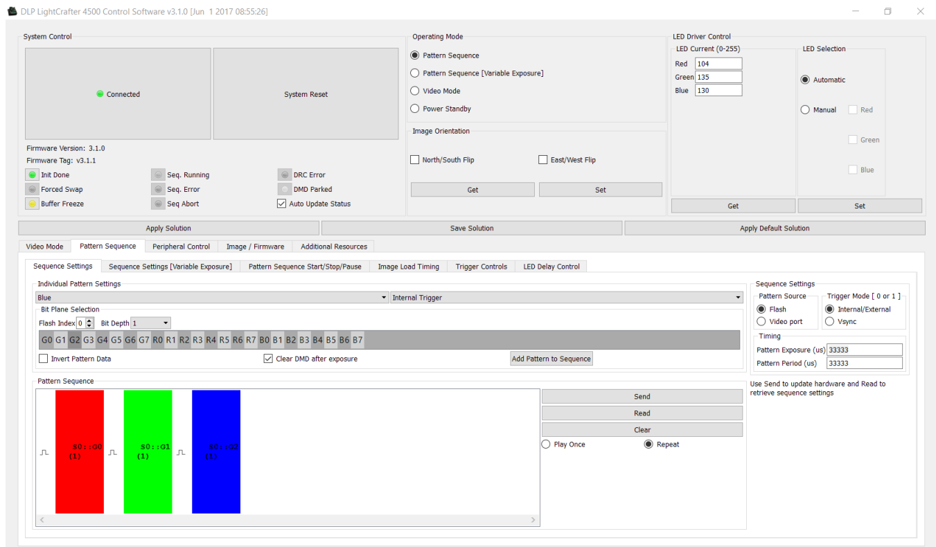
Figure 7. DLP LightCrafter 4500 Control Software – Pattern Sequence/Sequence Settings Tab
