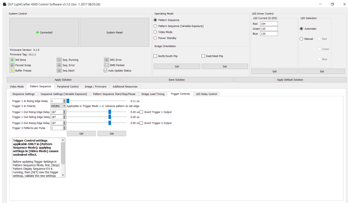
Figure 8. DLP LightCrafter 4500 Control Software – Pattern Sequence/Trigger Controls Tab
