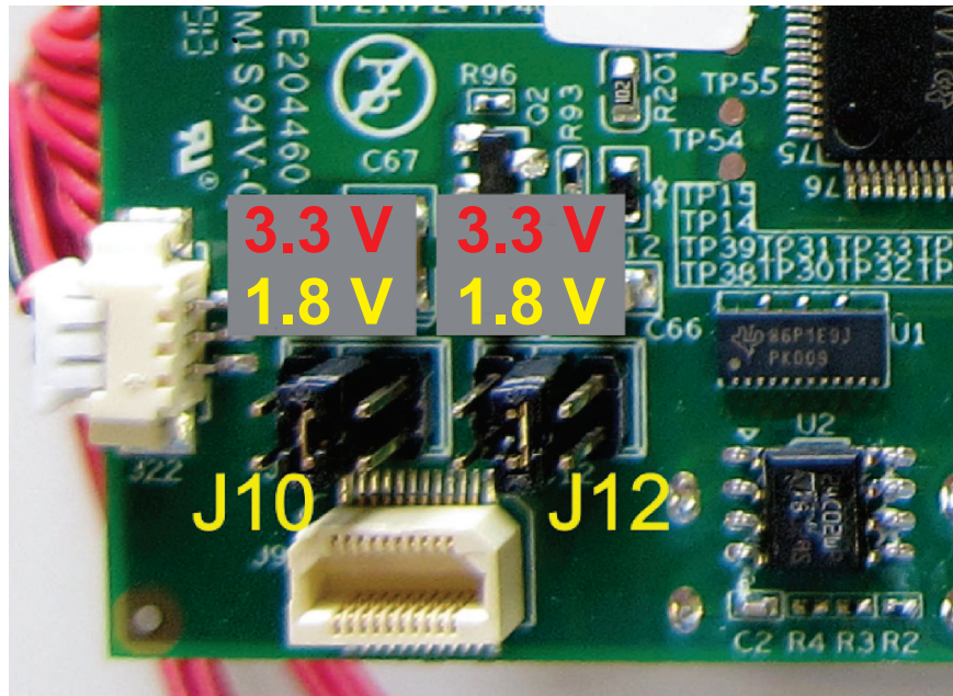
Figure 5. Jumper Locations for Setting Voltage Levels on J10 (Trigger In 1) and J12 (Trigger In 2)
