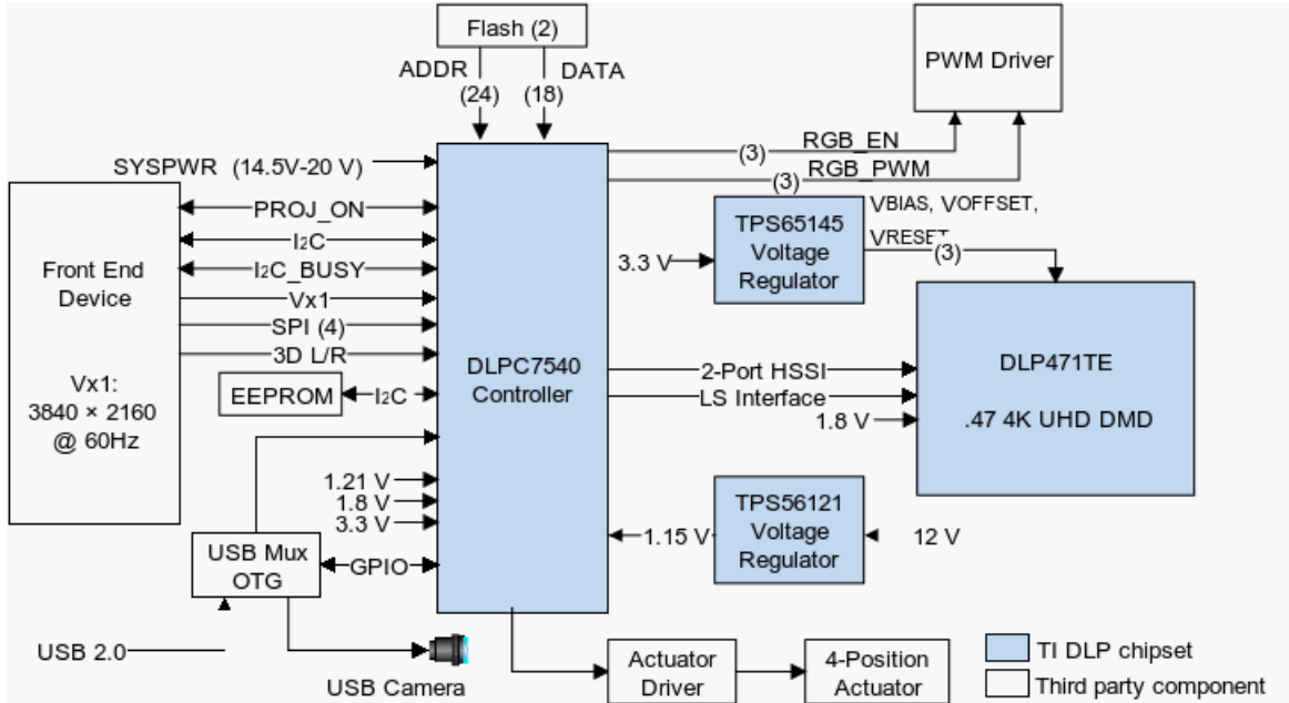
Figure 1-1. Typical Projector System Block Diagram
