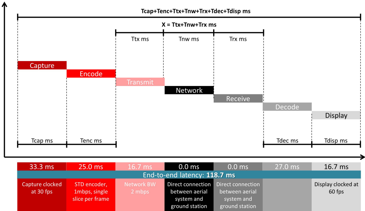
Figure 3: Video capture and display timeline.
