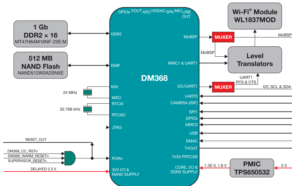
Figure 6: The TMS320DM368 digital media processor in a low-latency video-encoding Wi-Fi system for use in drones.
