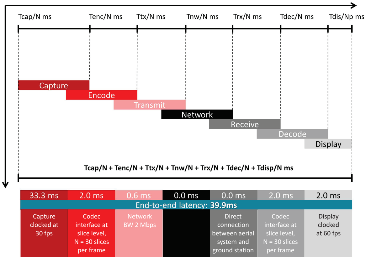
Figure 4: Slice-based impact on processing timeline.
