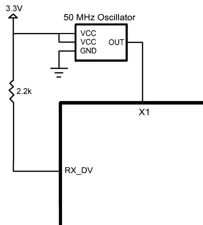
Figure 3. RMII Selection
