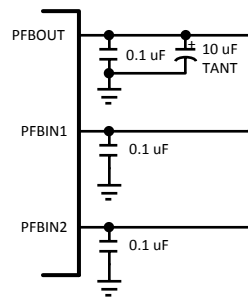
Figure 1. PFBOUT Connection
