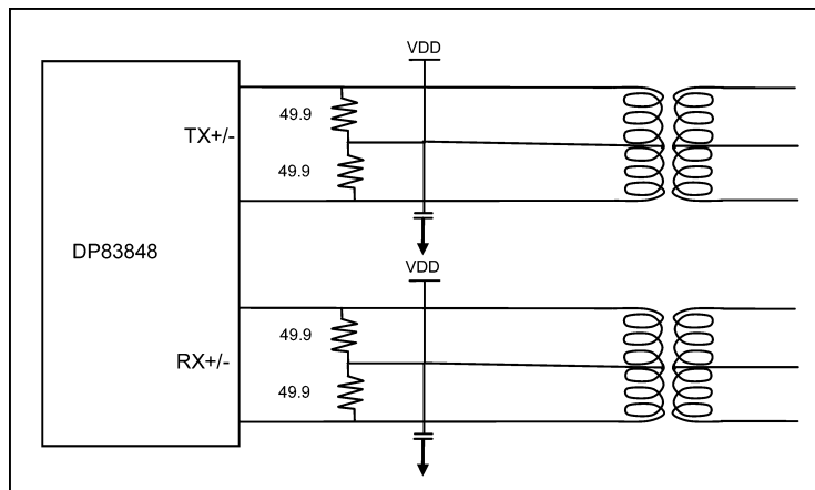
Figure 2. DP83848 PMD Connections (Termination)
