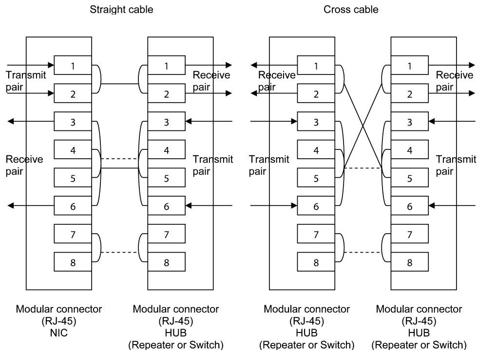
Figure 4. Auto-MDIX Operation
