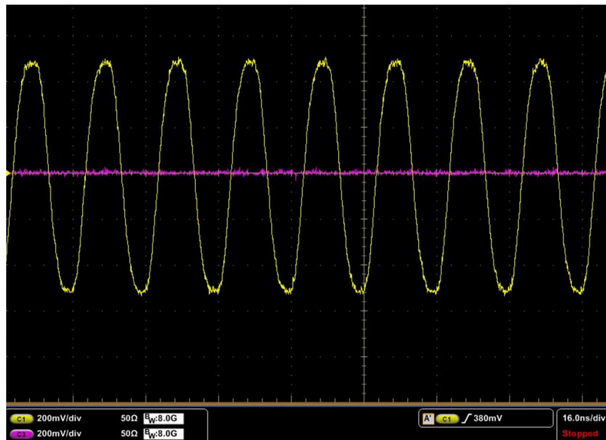
Figure C-4. DP83867 Test Mode 2 and 3 Output Waveform
