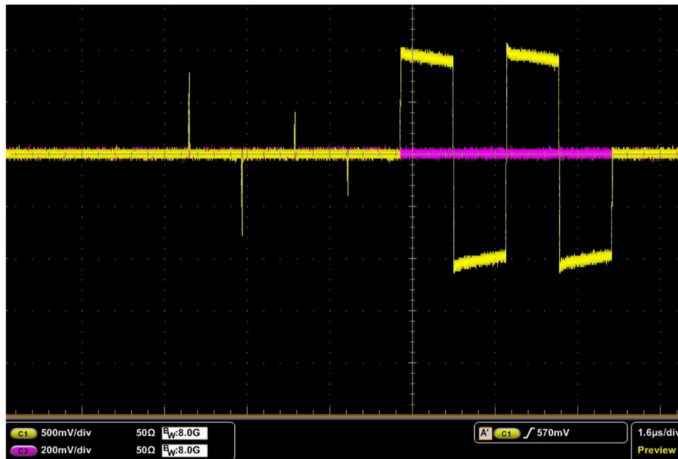
Figure C-2. DP83867 Test Mode 1 Output Waveform
