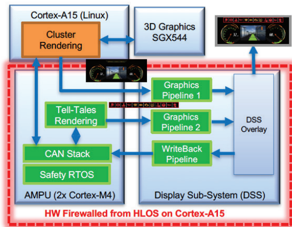
Figure 6. Jacinto 6 safety architecture based on AMPU.
