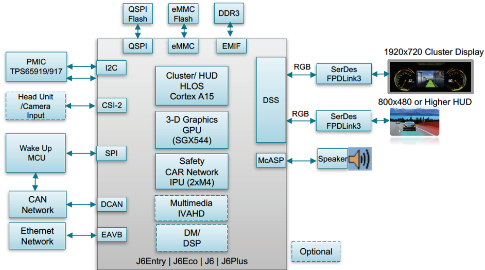
Figure 1. Digital cluster system block diagram.
