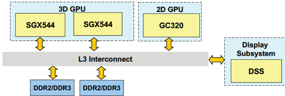
Figure 5. Jacinto 6 graphics and display subsystem architecture.
