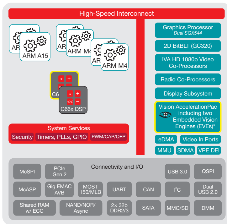
Figure 2. TI's "Jacinto 6 Ex" processor diagram
