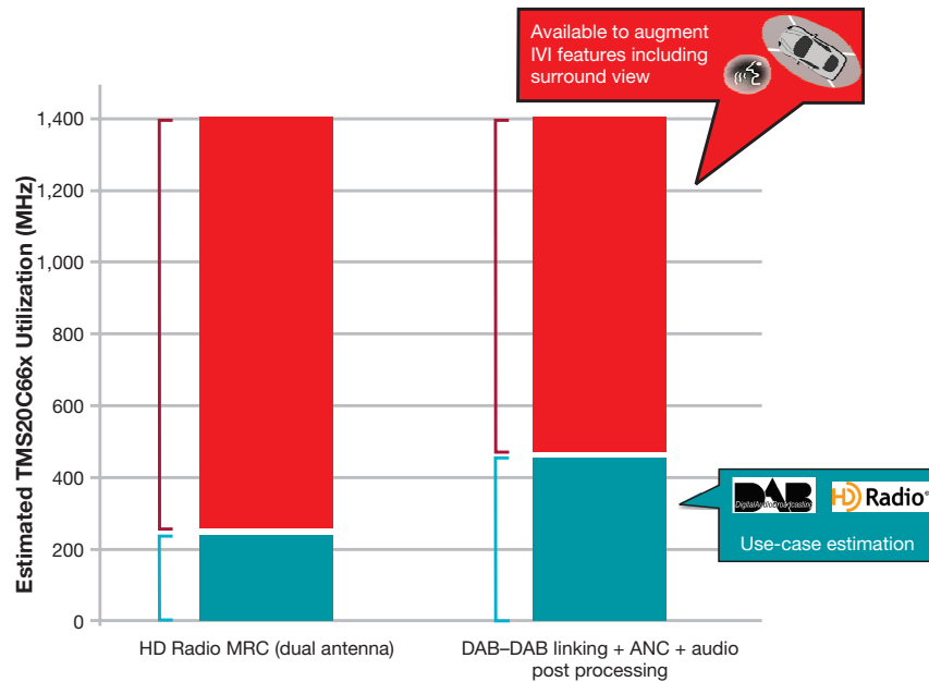
Figure 3. Example DSP partitioning on “Jacinto 6 Ex” combining radio/audio features with headroom for informational ADAS
