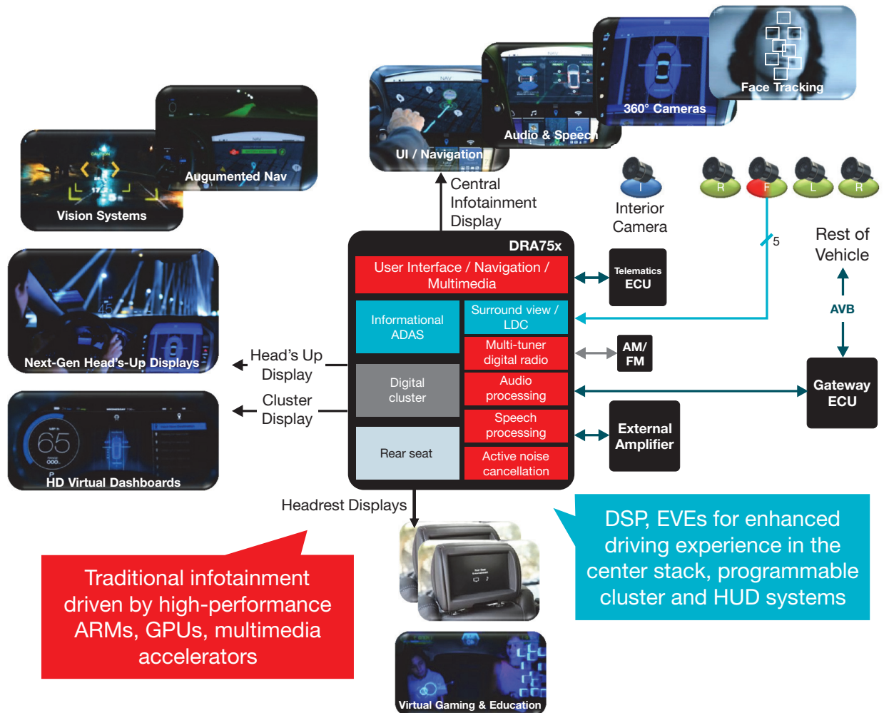
Figure 5. DRA75x “Jacinto 6 Ex” integrated capabilities including informational ADAS
