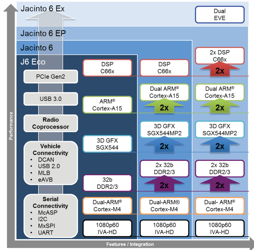
Figure 6. "Jacinto 6" family scalability
