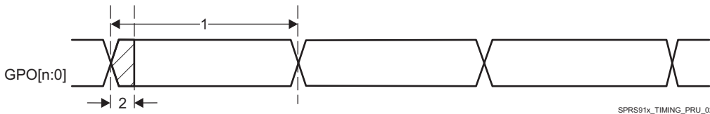
Figure 5-110. PRU-ICSS PRU Direct Output Timing
