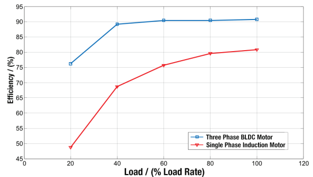
Figure 12: Efficiency comparison*
