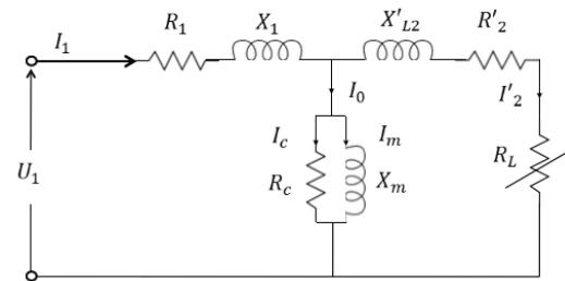
Figure 8: Per-phase equivalent circuit for a three-phase induction motor [7]
