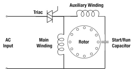
Figure 3: Capacitor start/run single-phase induction motor drive [1]
