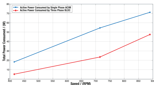
Figure 15: Comparison of power consumption between single-phase AC induction motor versus three-phase BLDC motor
