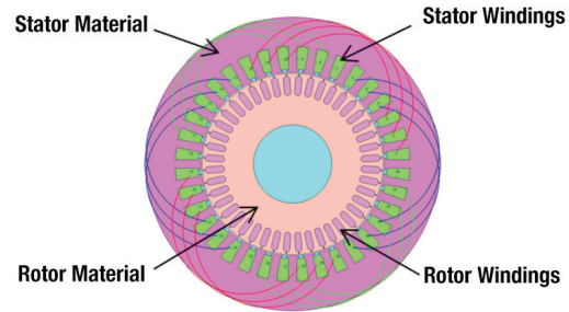
Figure 7: Example three-phase ACIM cross-section
