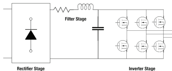
Figure 1: Drive stage for three-phase systems
