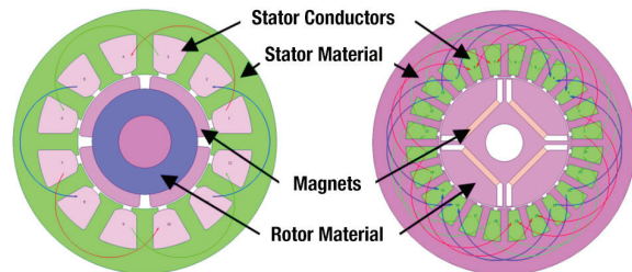
Figure 9: Example of three-phase BLDC motor cross-section: SM-PMSM (left); IPMSM (right)
