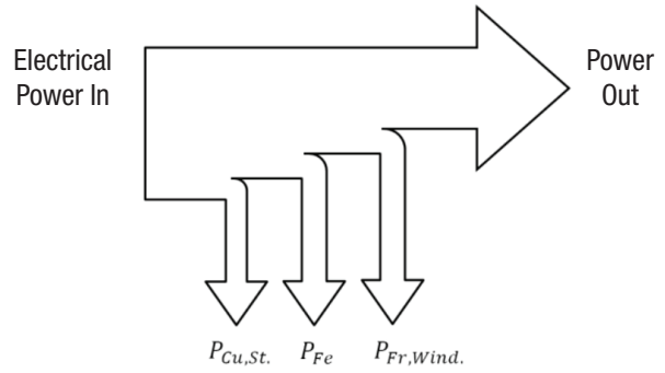
Figure 11: Power flow diagram of a brushless DC motor
