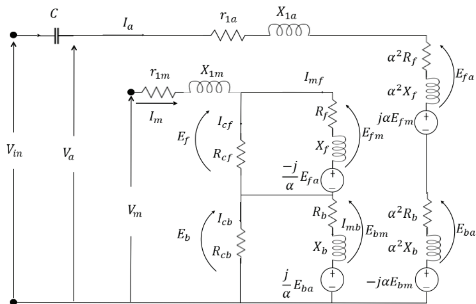
Figure 4: Equivalent circuit model for a SPIM [3]
