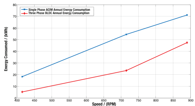
Figure 16: Comparison of annual energy consumption between single-phase AC induction motor versus three-phase BLDC motor-based on the selected use case (two hours per day for 365 days)
