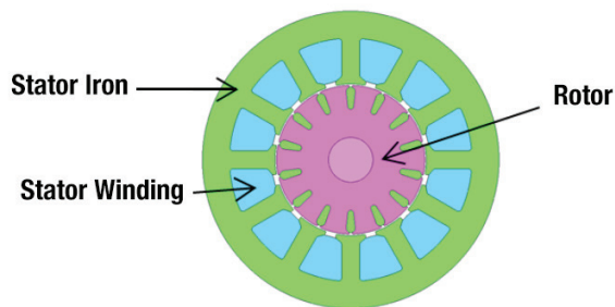
Figure 2: Single-phase induction motor example cross section
