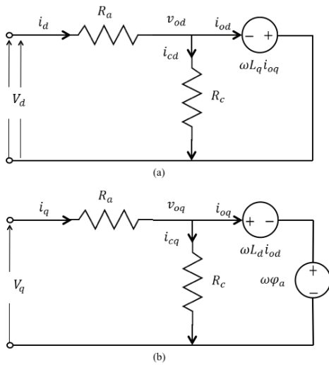
Figure 10: Rotor reference frame loss model of a BLDC motor
