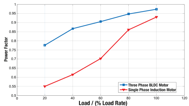
Figure 13: Power factor comparison*
