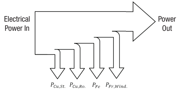
Figure 6: Losses in a single-phase induction motor [02]
