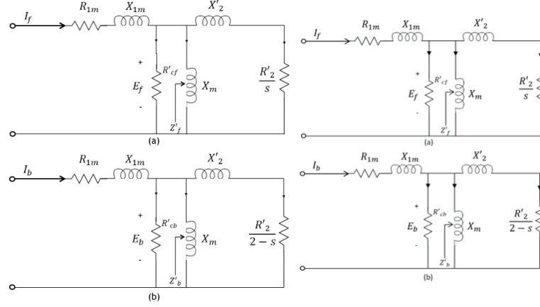
Figure 5: Equivalent circuit for SPIM forward (a) and backward (b) components [3]
