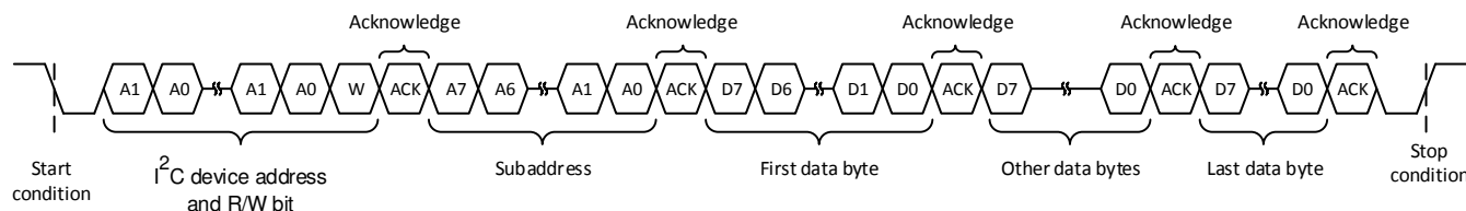
Figure 10. Multiple-Byte Write Transfer
