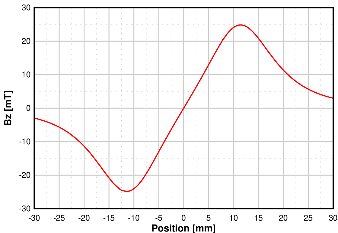
Figure 2-2. Observed DRV5055 Magnetic Flux Density
