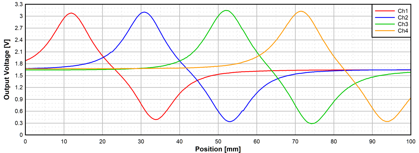
Figure 5-1. Measured DRV5055 Array Output
