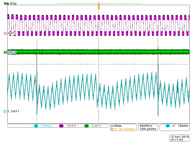
Figure 145. Motor Operation in PWM Mode
