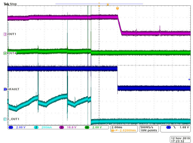
Figure 147. Active Open-Load Detection
