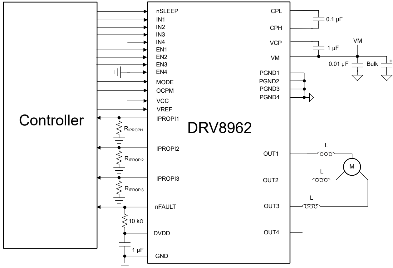
Figure 8-9. Driving BLDC Motor with DRV8962
