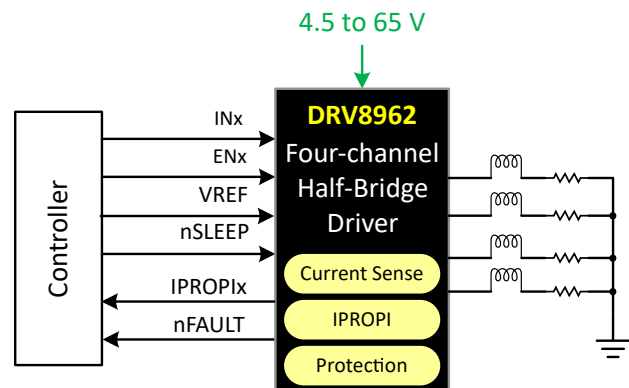
DRV8962 Simplified Schematic
