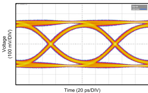
Figure 7. Typical Application Transmit Eye Diagram, 10.3125 Gbps
