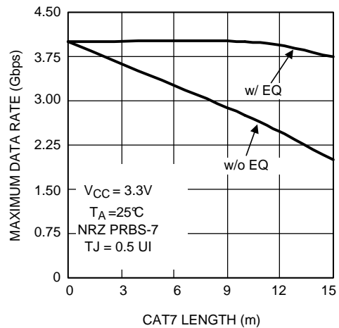
Figure 16. Maximum Data Rate as a Function of CAT7 (Siemon Tera) Length
