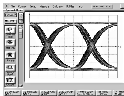
Figure 10. Data Eye After 20-In Backplane With 3 dB Tx Pre-Emphasis and 5 dB Rx Equalization
