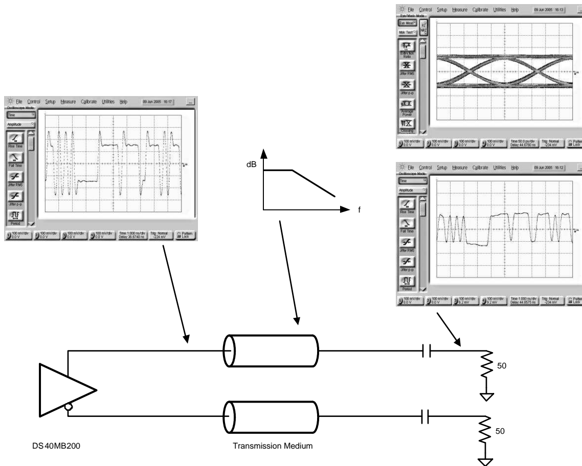
Figure 1. Pre-Emphasis Waveforms
