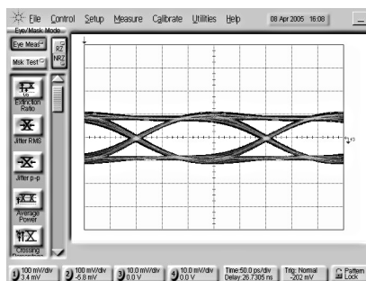
Figure 6. Data Eye After 30-In FR4 Board Trace – Over Equalized
