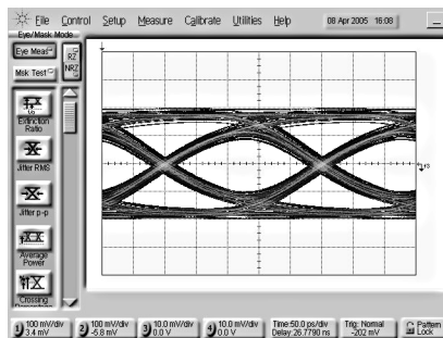
Figure 5. Data Eye After 30-In FR4 Board Trace – Under Equalized
