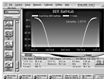
Figure 12. Bathtub Plot Showing Prediction of Eye Opening at Various Error Rates
