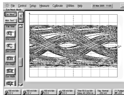
Figure 9. Data Eye After 20-In Backplane Without Equalization
