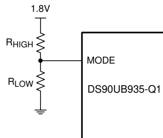
Figure 7-7. MODE Configuration
