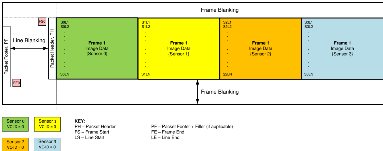
Figure 7-17. Line-Concatenated Format
