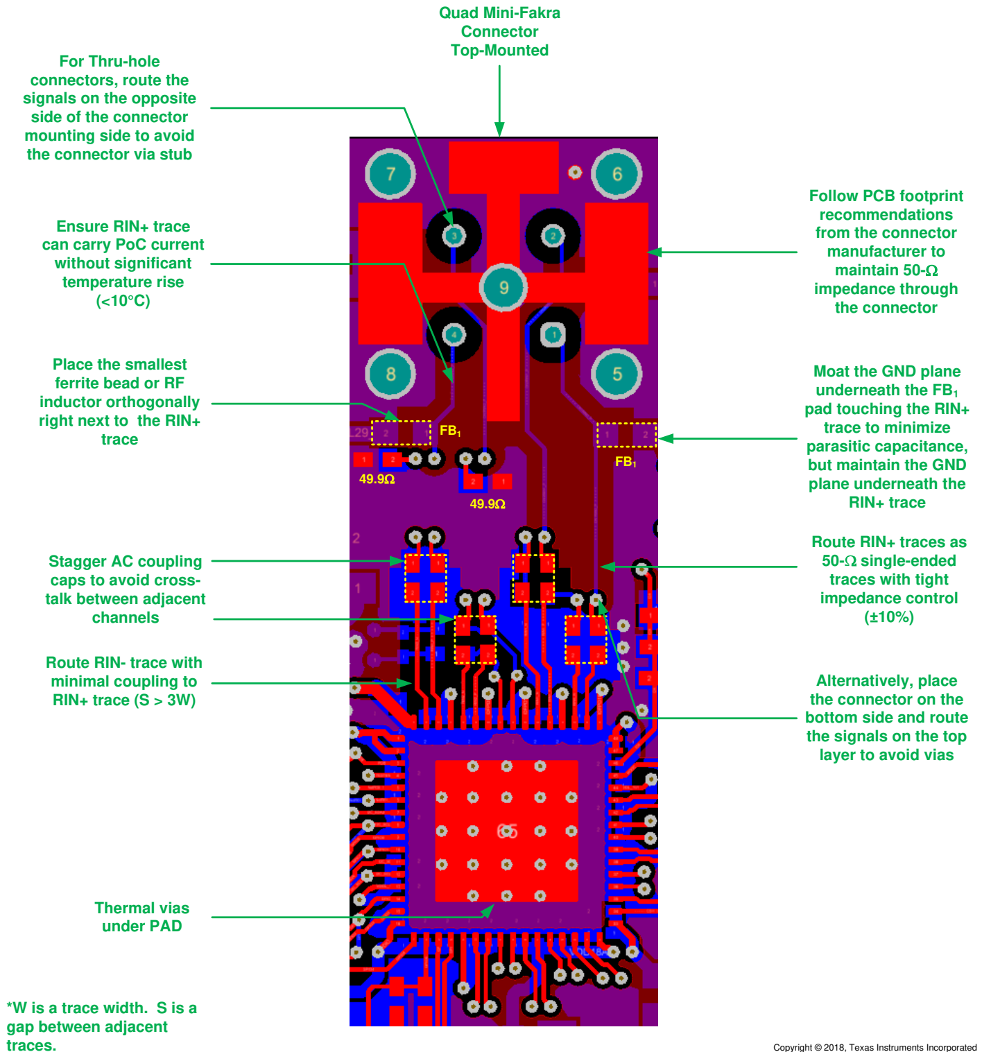
Figure 10-1. DS90UB962-Q1 Example PCB Layout With Quad Mini-Fakra Connector
