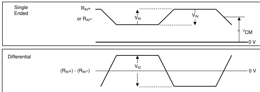
Figure 6-2. FPD-Link Receiver VID
