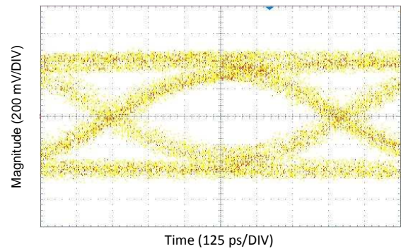
Figure 25. DS90UR241 DOUT \pm at 1.2 Gbps Measured at RIN \pm Termination; VODSEL=HIGH
