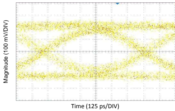
Figure 24. DS90UR241 DOUT \pm at 1.2 Gbps Measured at RIN \pm Termination; VODSEL=LOW
