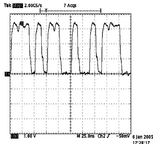
Figure 8. 2 mA FPGA Output +4" Trace with PRBS Data
