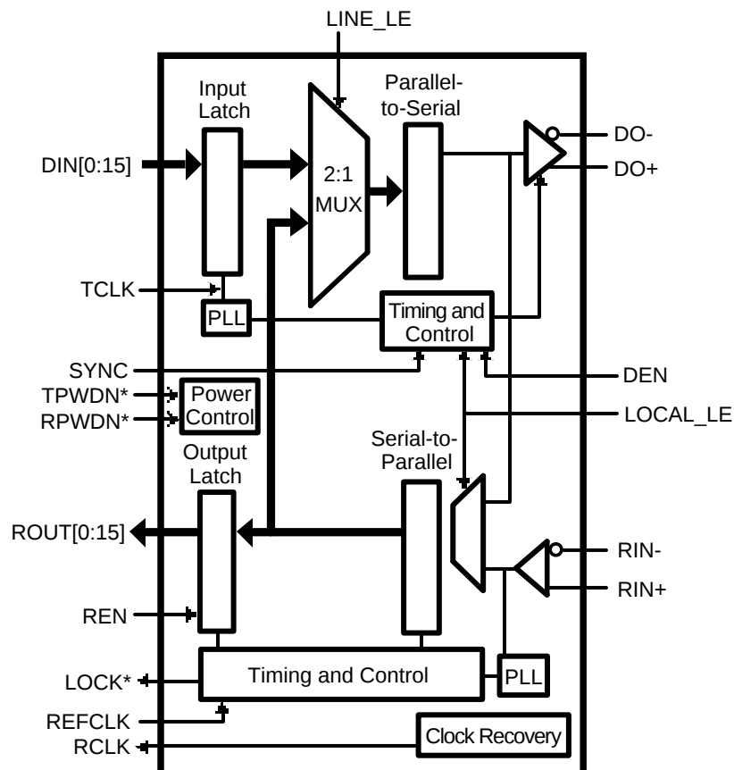
Figure 3. DS92LV16 Block Diagram
