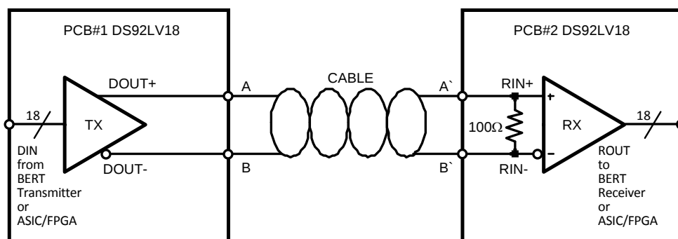
Figure 10. DS92LV18 SerDes BER Test Setup
