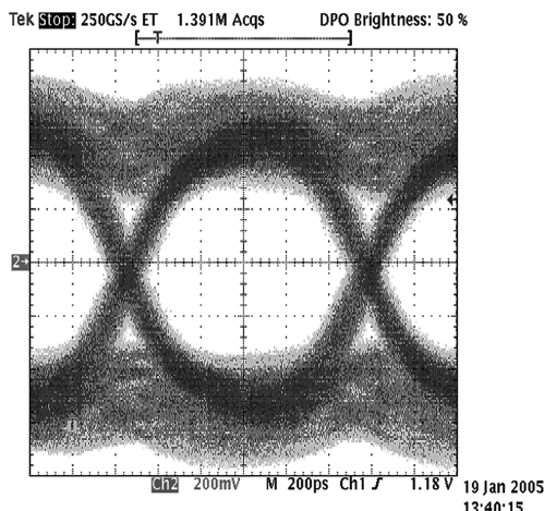
Figure 9. Eye Diagram after 1m of CAT5 Cable
