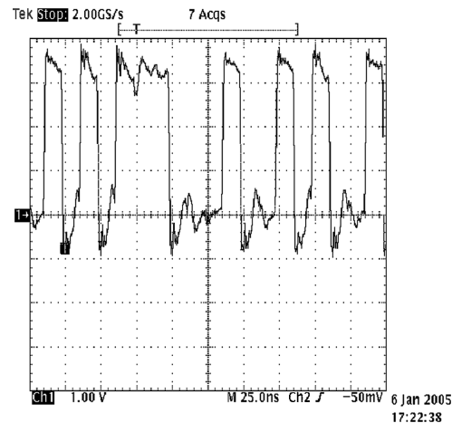
Figure 7. 24 mA FPGA Output +4" Trace with PRBS Data
