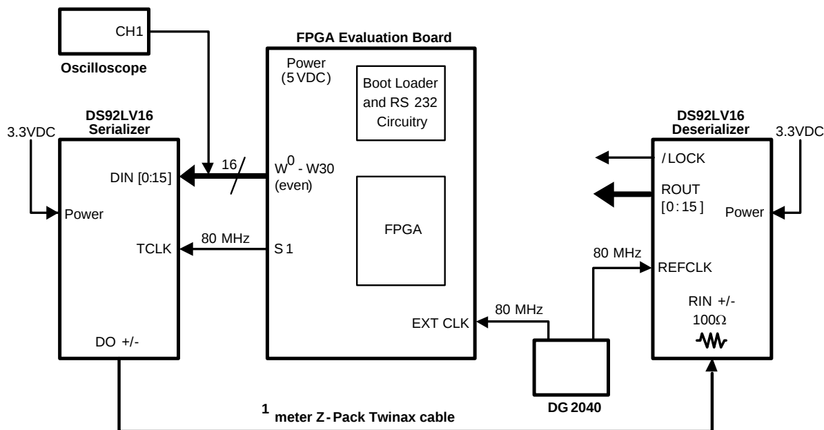
Figure 1. DS92LV16 SerDes and Cyclone FPGA Test Setup
