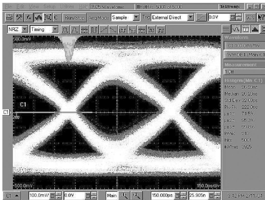
Figure 12. Eye Diagram Measured after 15m of Infiniband Cable at the Input of the DS92LV18 Receiver; f_{TCLK} = 66 MHz (1.32 Gbps); Max Pre-emphasis
