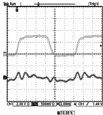
Figure 5. Active Output Transitions and “Quiet Output” (bottom), SS Data, 2 mA
