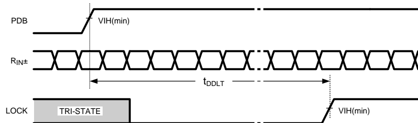
Figure 8. Deserializer PLL Lock Times
