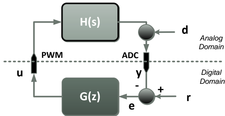
Figure 3. Digitally Controlled Control System
