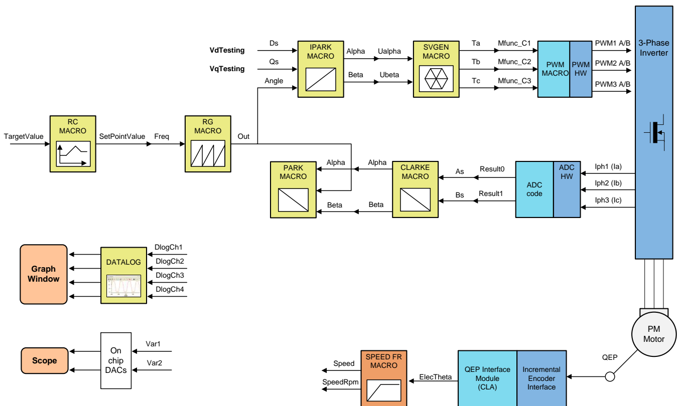
Figure 13. Level 2 Block Diagram
