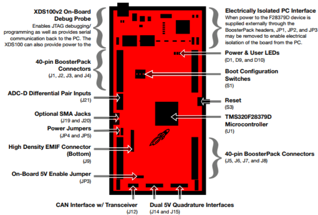
Figure 4. LAUNCHXL-F28379D Layout Diagram
