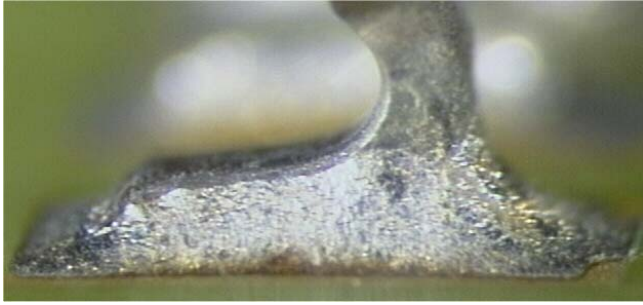
Figure 12. Group 1A, NiPdAu Finish, Stored Loose, 96-h Exposure
