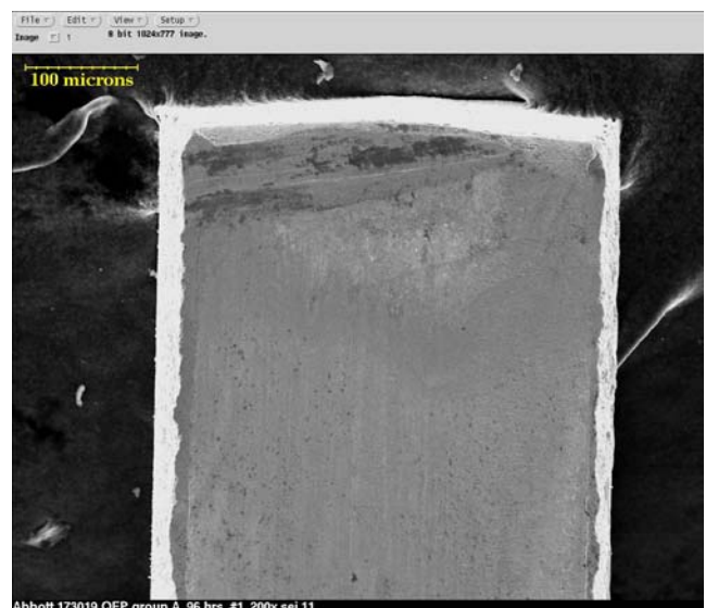
Figure 3. Group 1A NiPdAu 0.01- \mu m (0.4- \mu ”) Pd, Loose, 96 h, 200 \times
