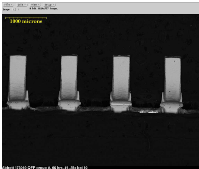
Figure 2. Group 1A NiPdAu 0.01- \mu m (0.4- \mu ”) Pd, Loose, 96 h, 25 \times , Bottom Lead View
