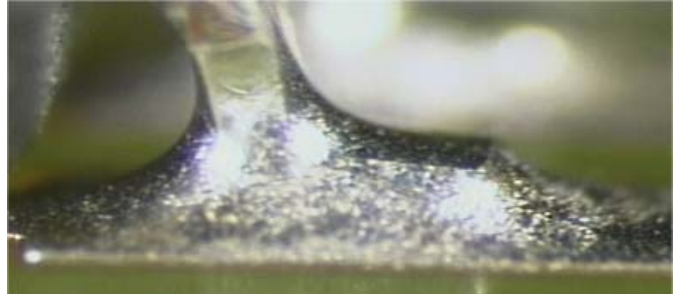
Figure 19. Group 4B, Sn Finish, Stored in Tubes, 96-h Exposure
