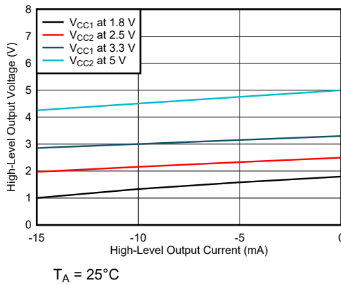
Figure 6-11. High-Level Output Voltage vs High-level Output Current
