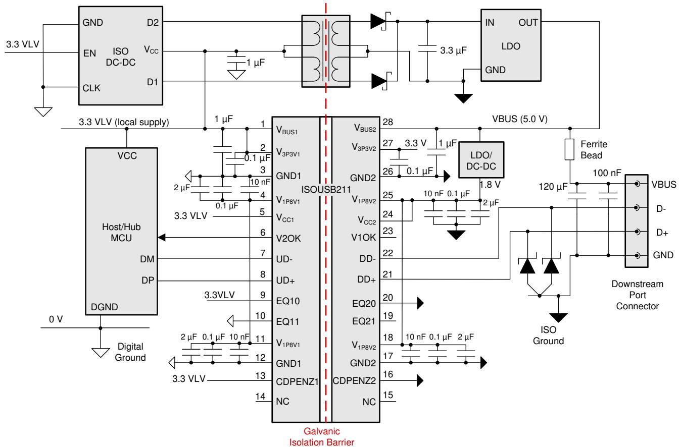
Figure 9-1. Isolated Host or Hub with ISOUSB211
